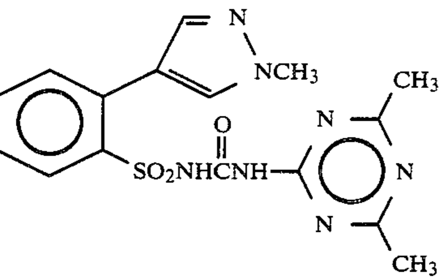
Compound 36
