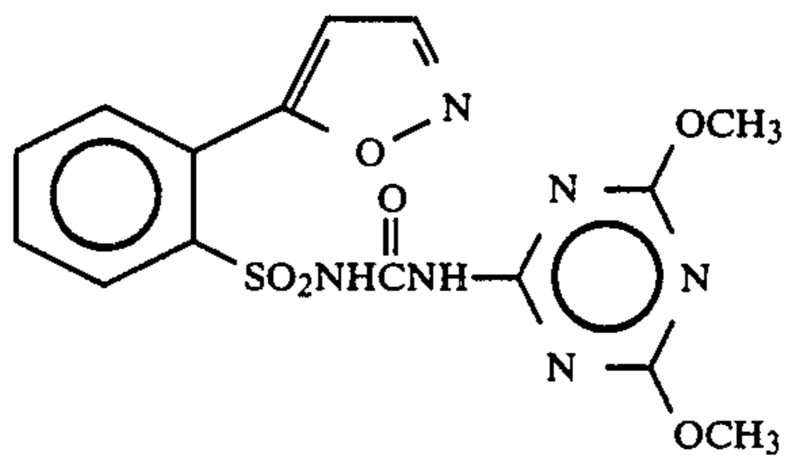
Compound 27
