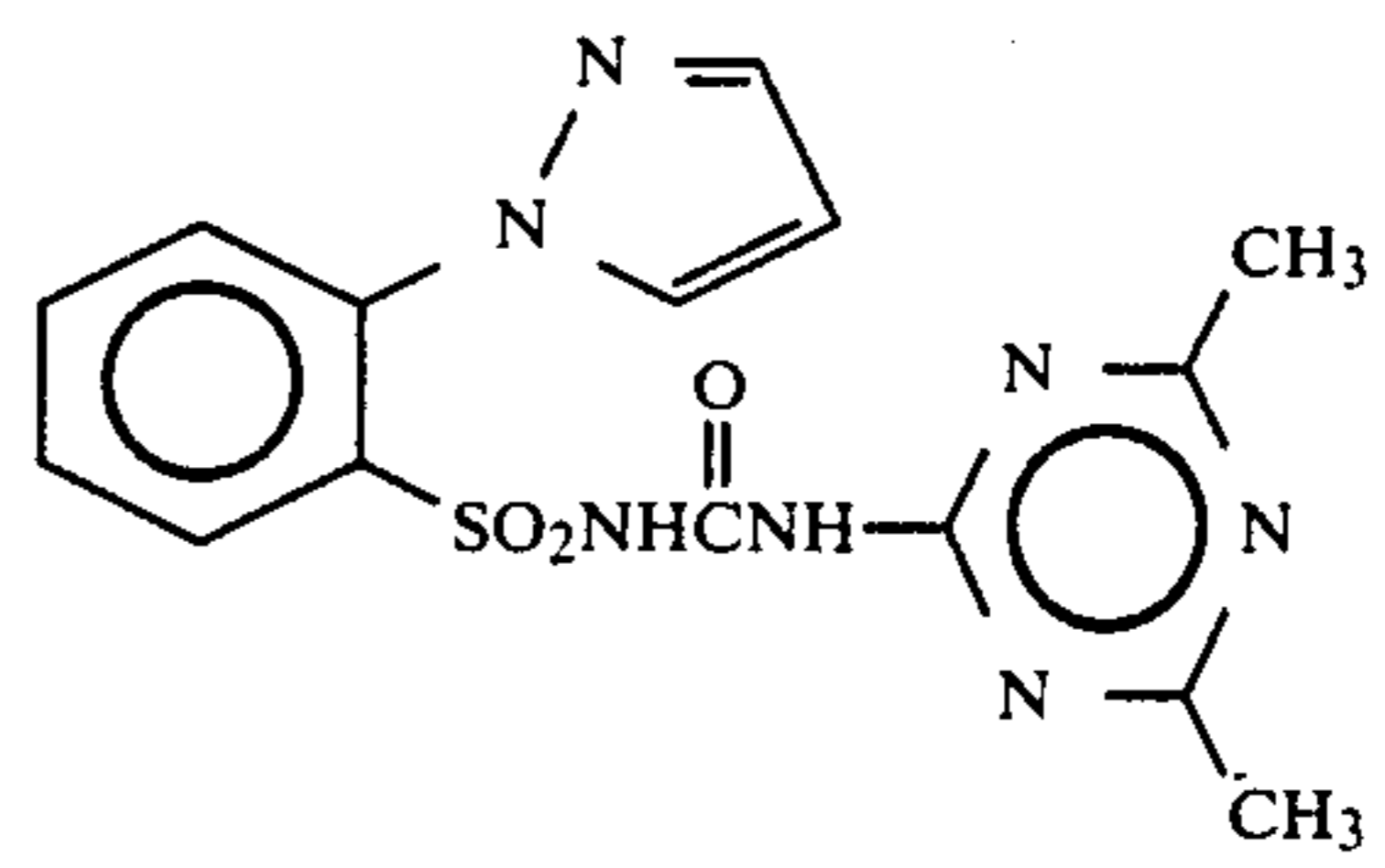
Compound 50
