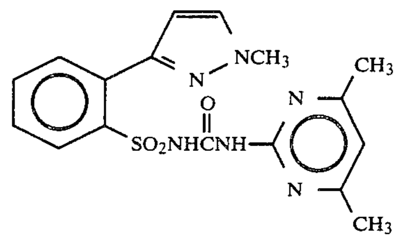
Compound 38
