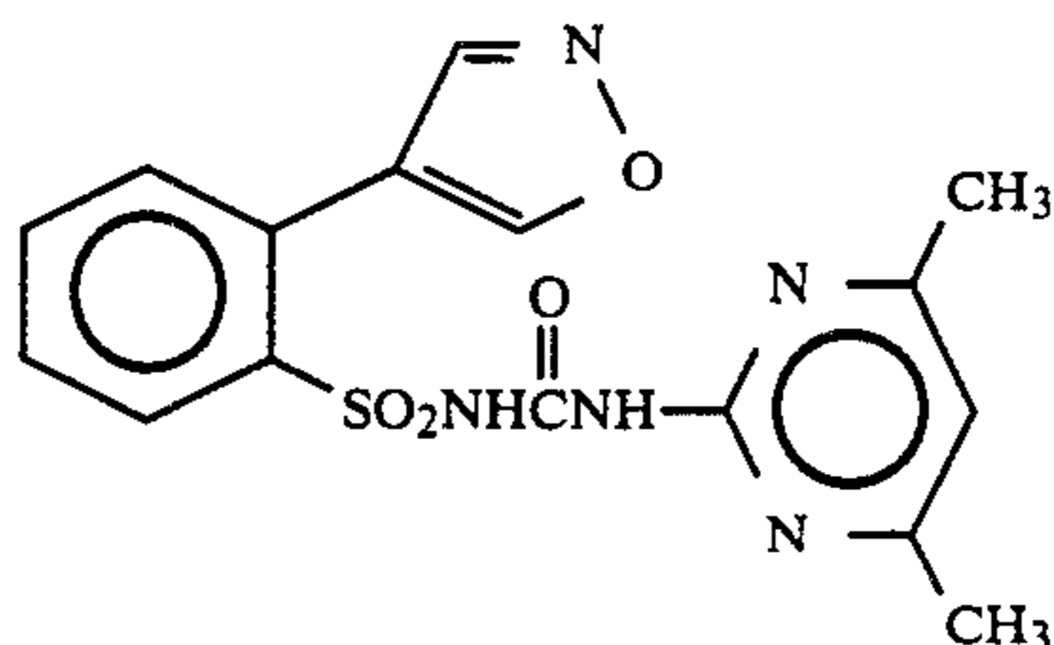
Compound 30
