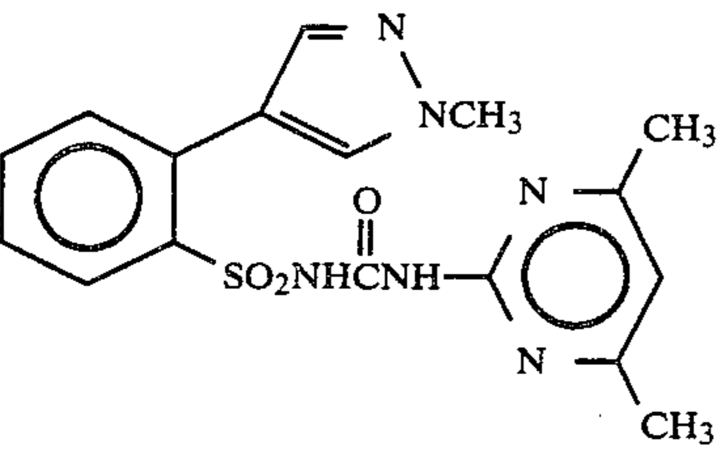
Compound 34
