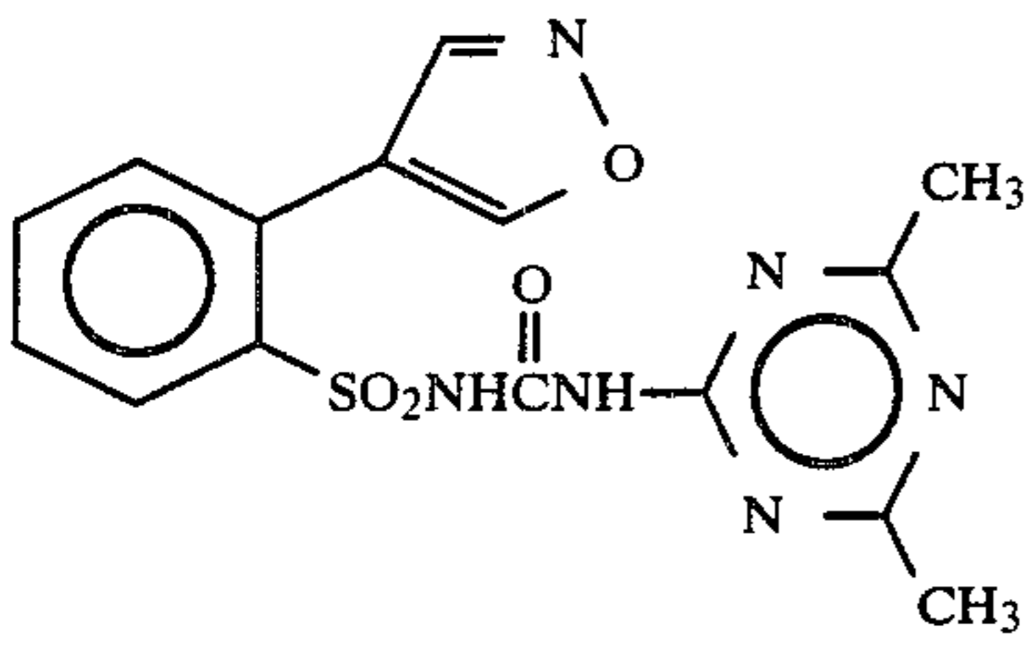
Compound 32
