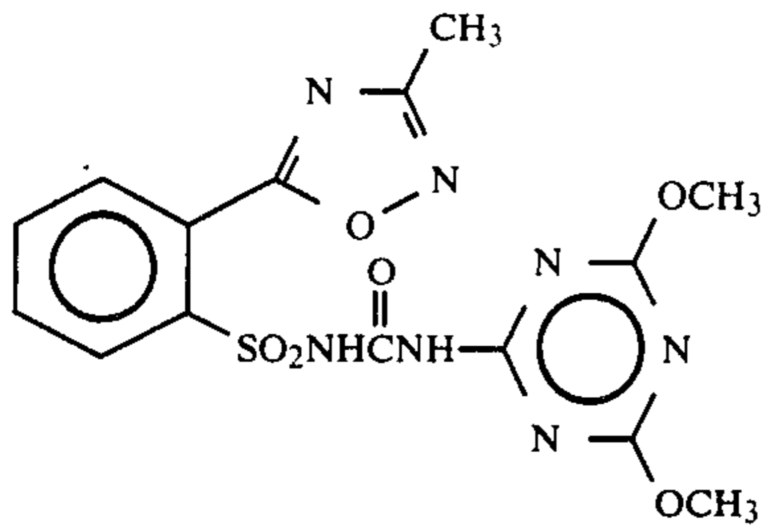
Compound 18 5
