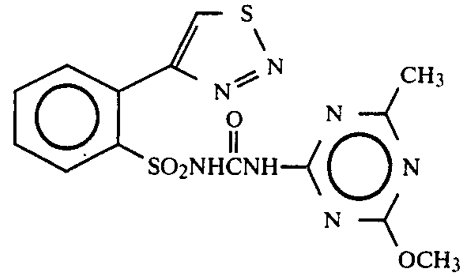
Compound 24
