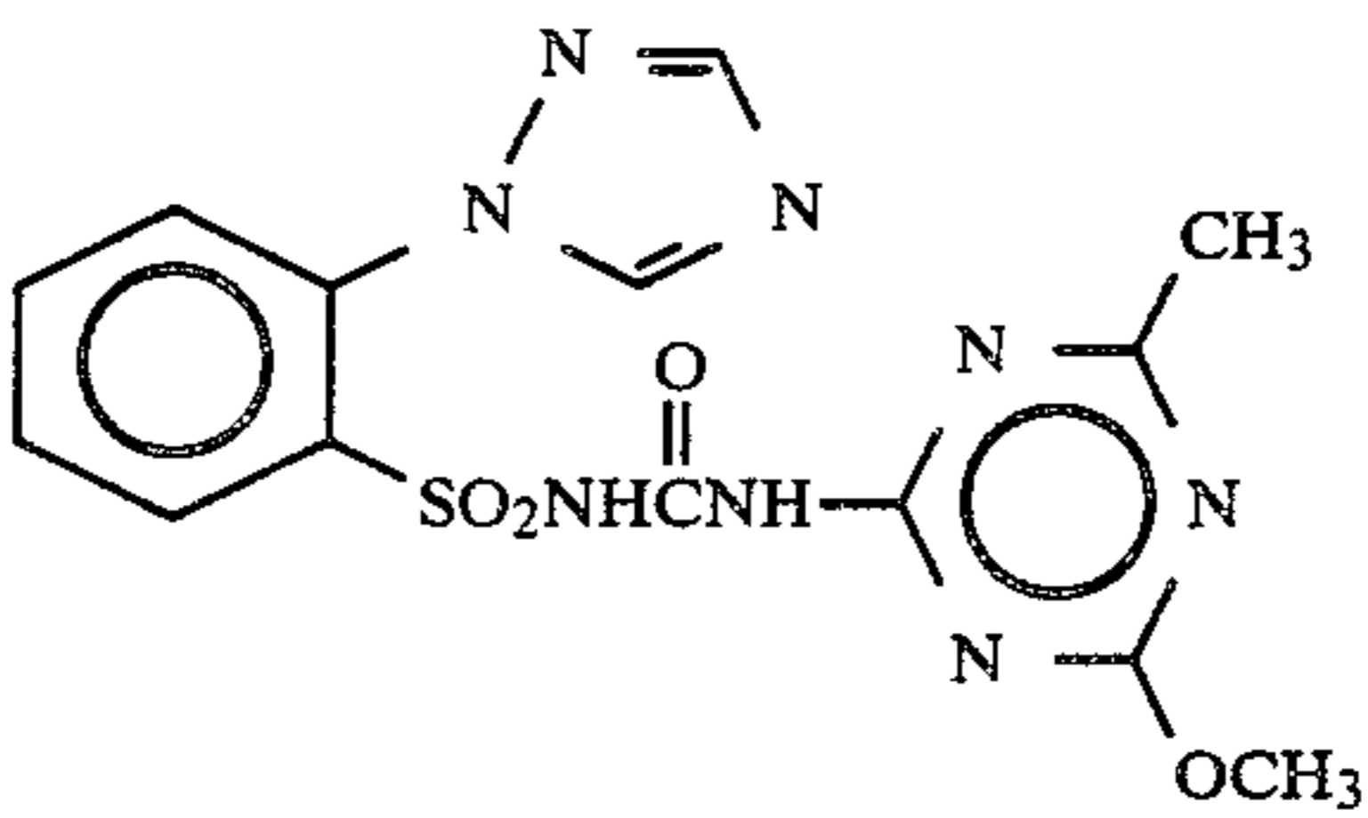
Compound 42
