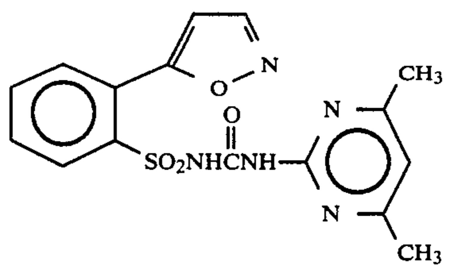
Compound 26
