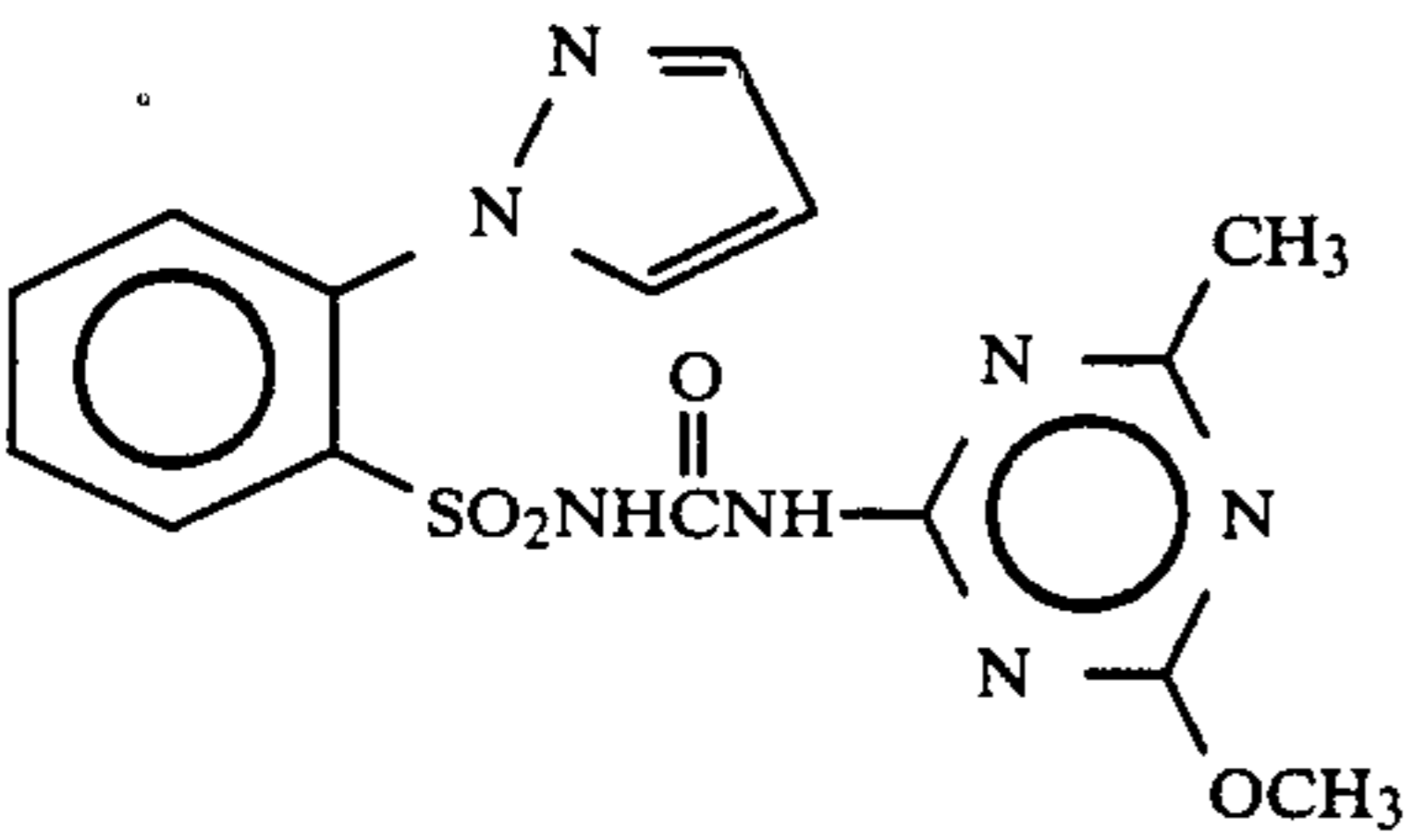
Compound 48
