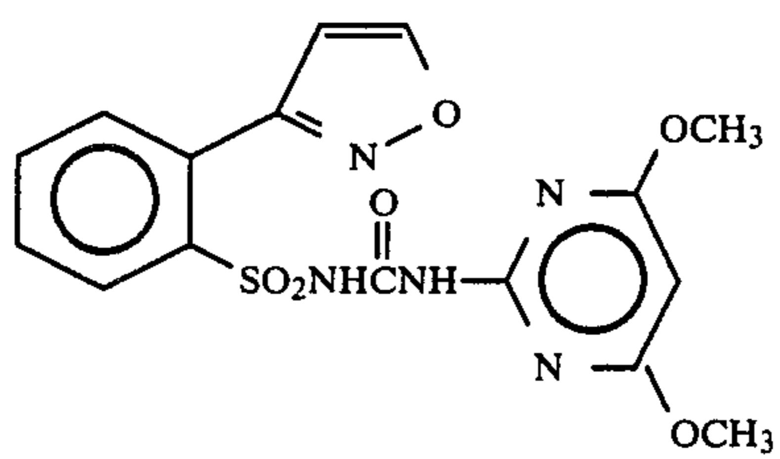
Compound 52
