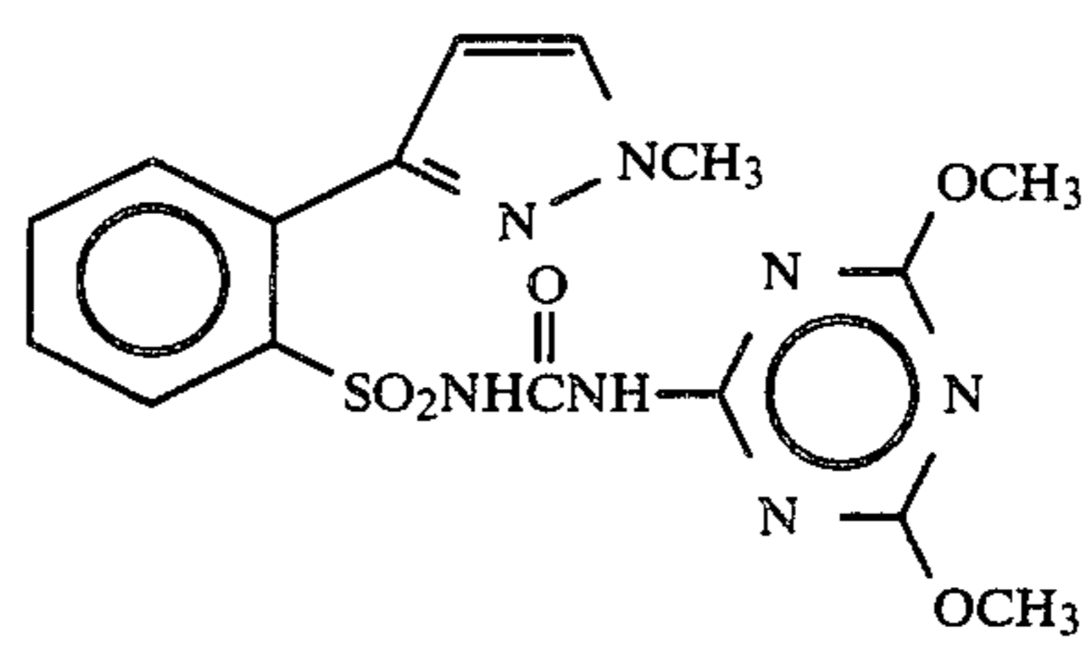
Compound 39
