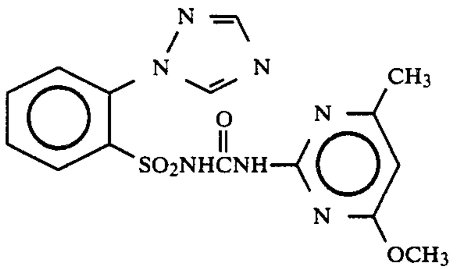
Compound 55
