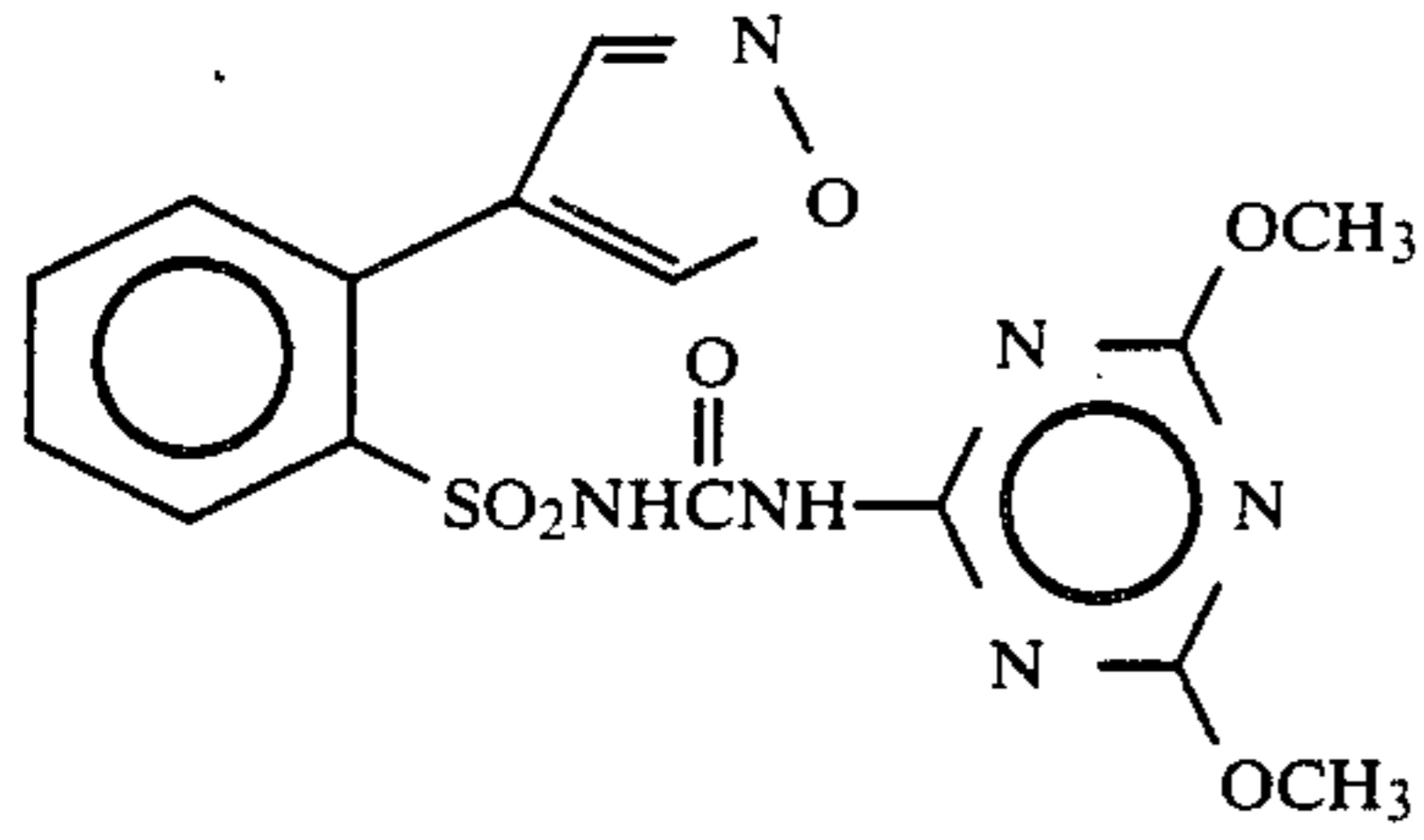
Compound 31
