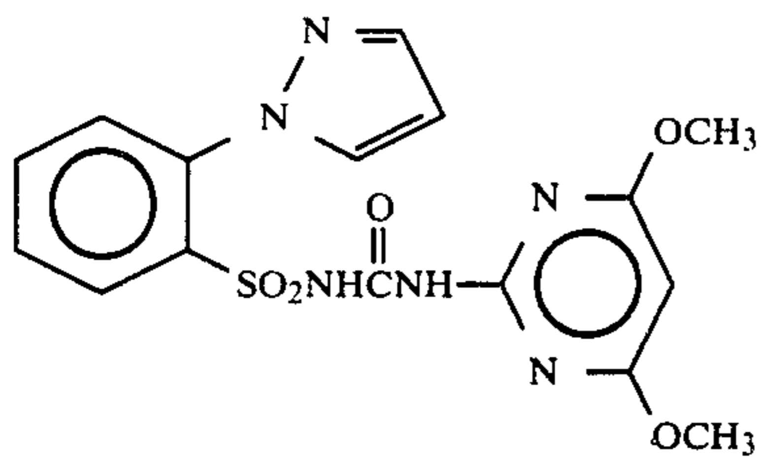
Compound 45
