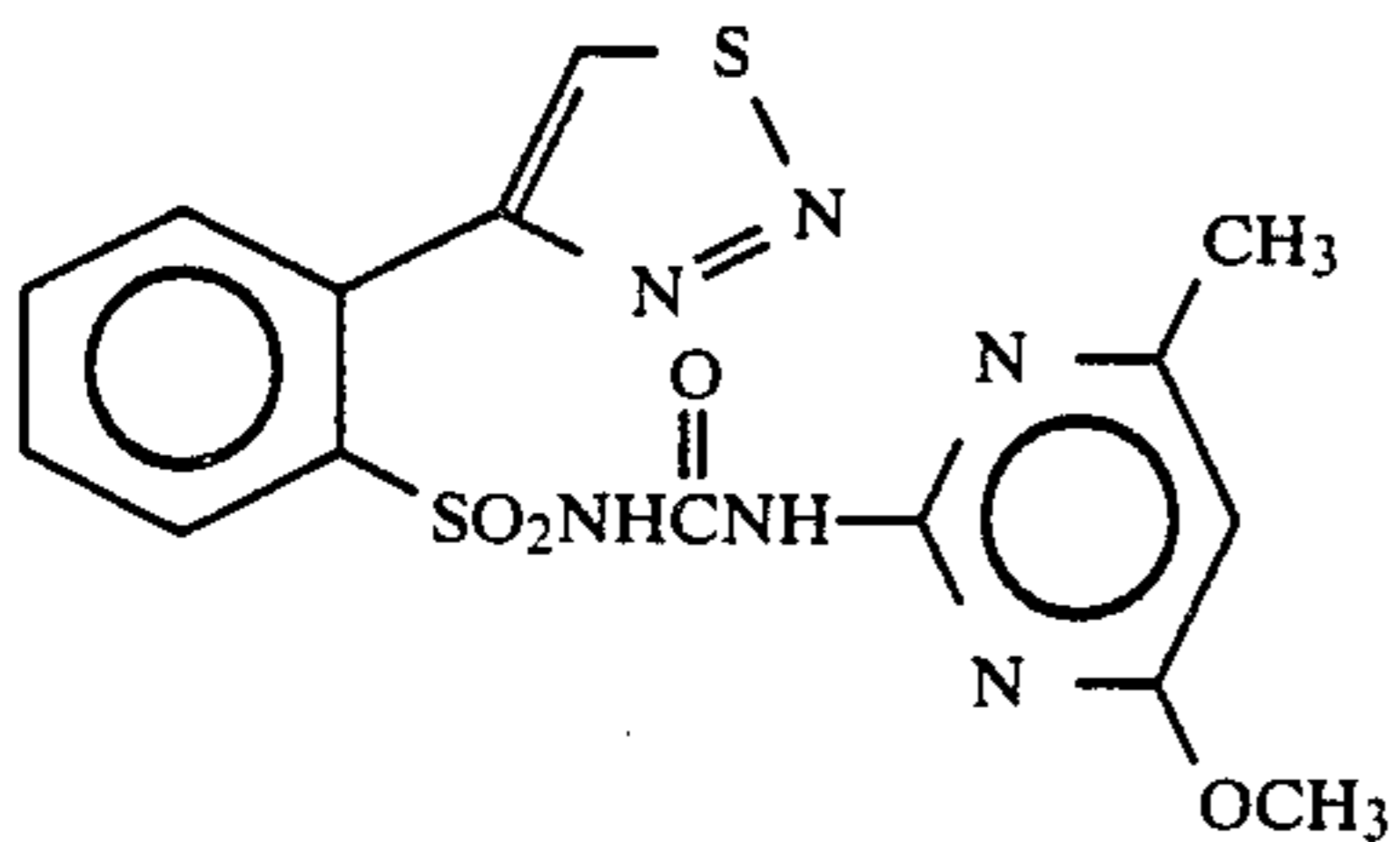
Compound 21
