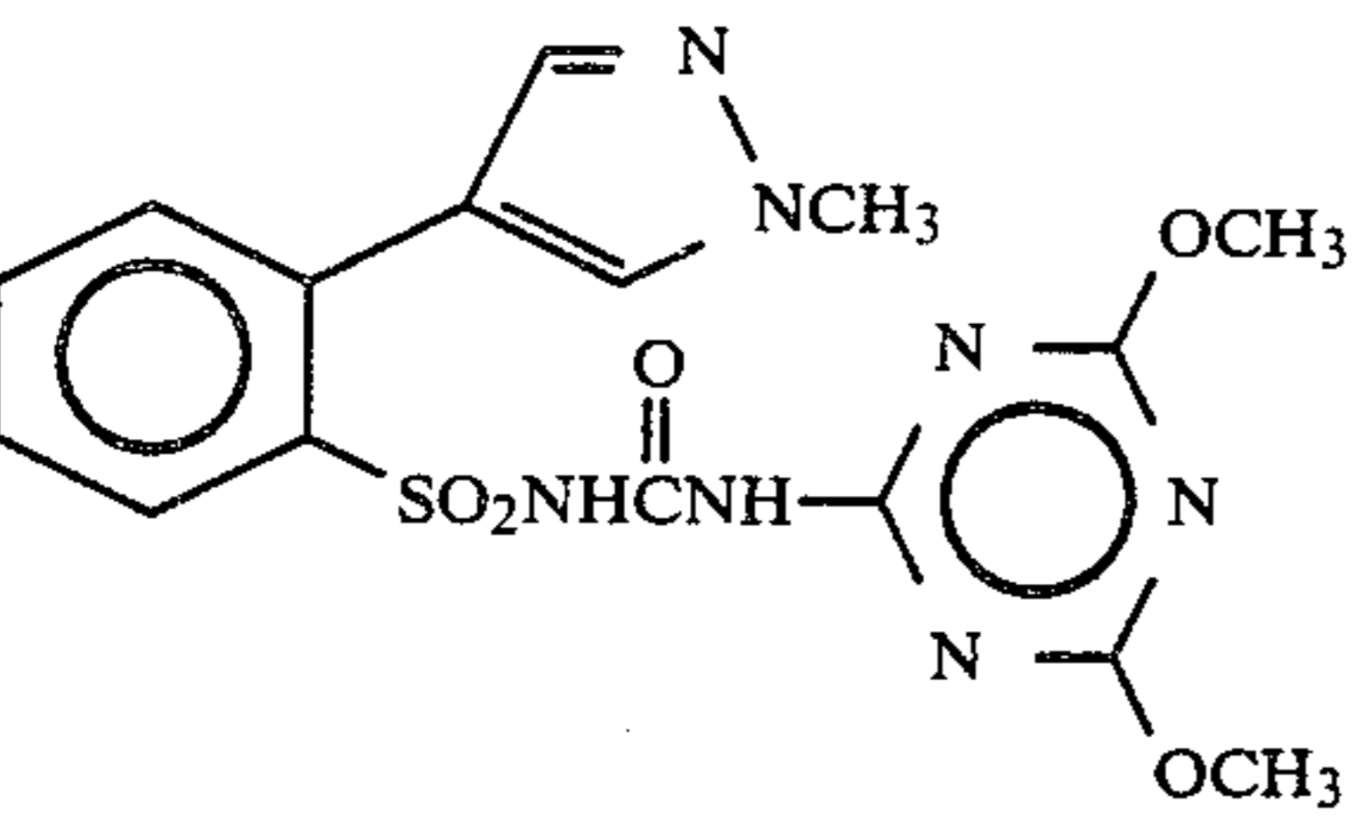
Compound 35
