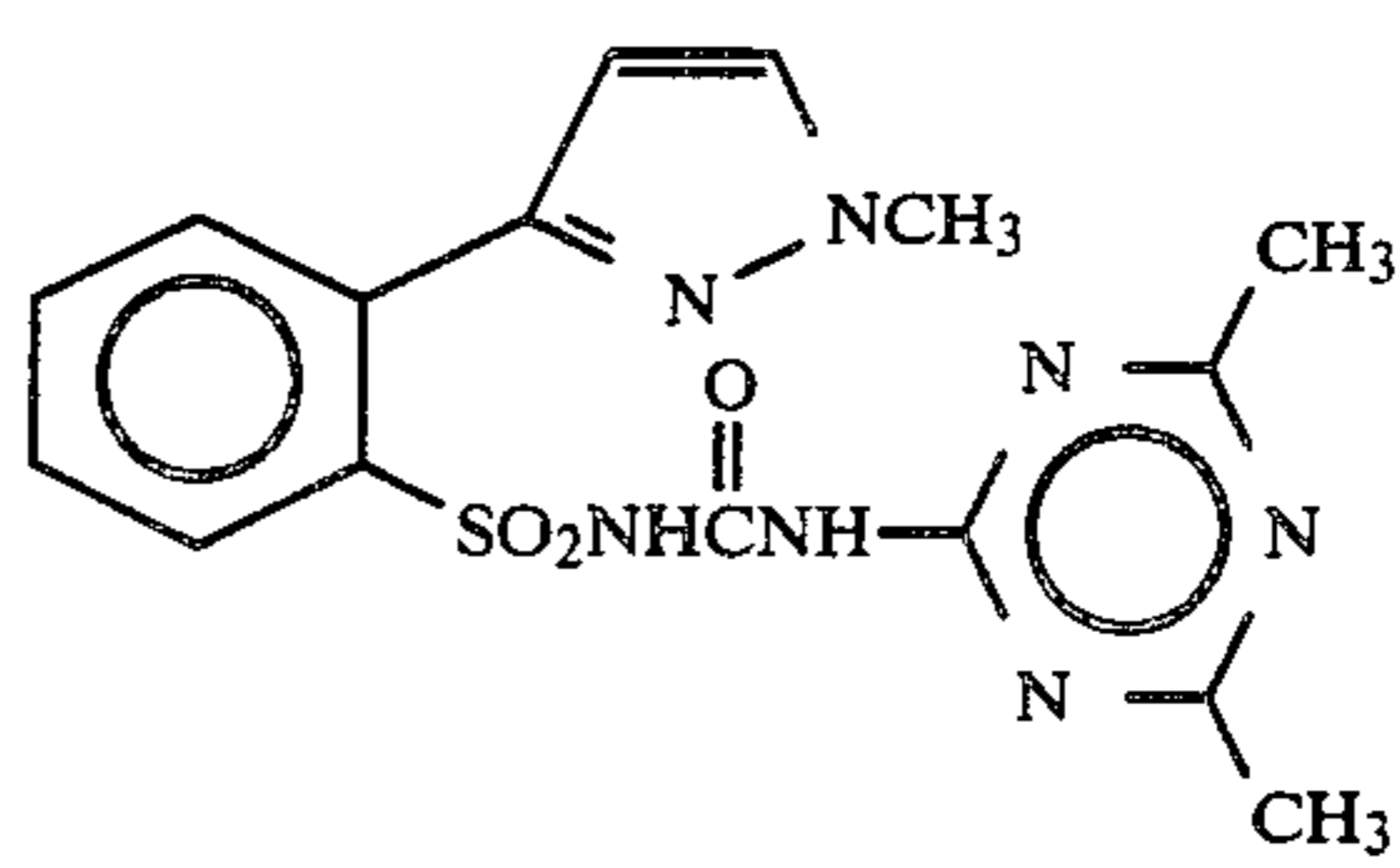
Compound 40
