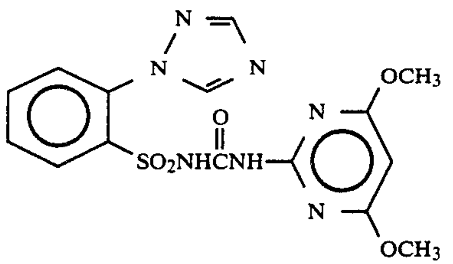
Compound 54
