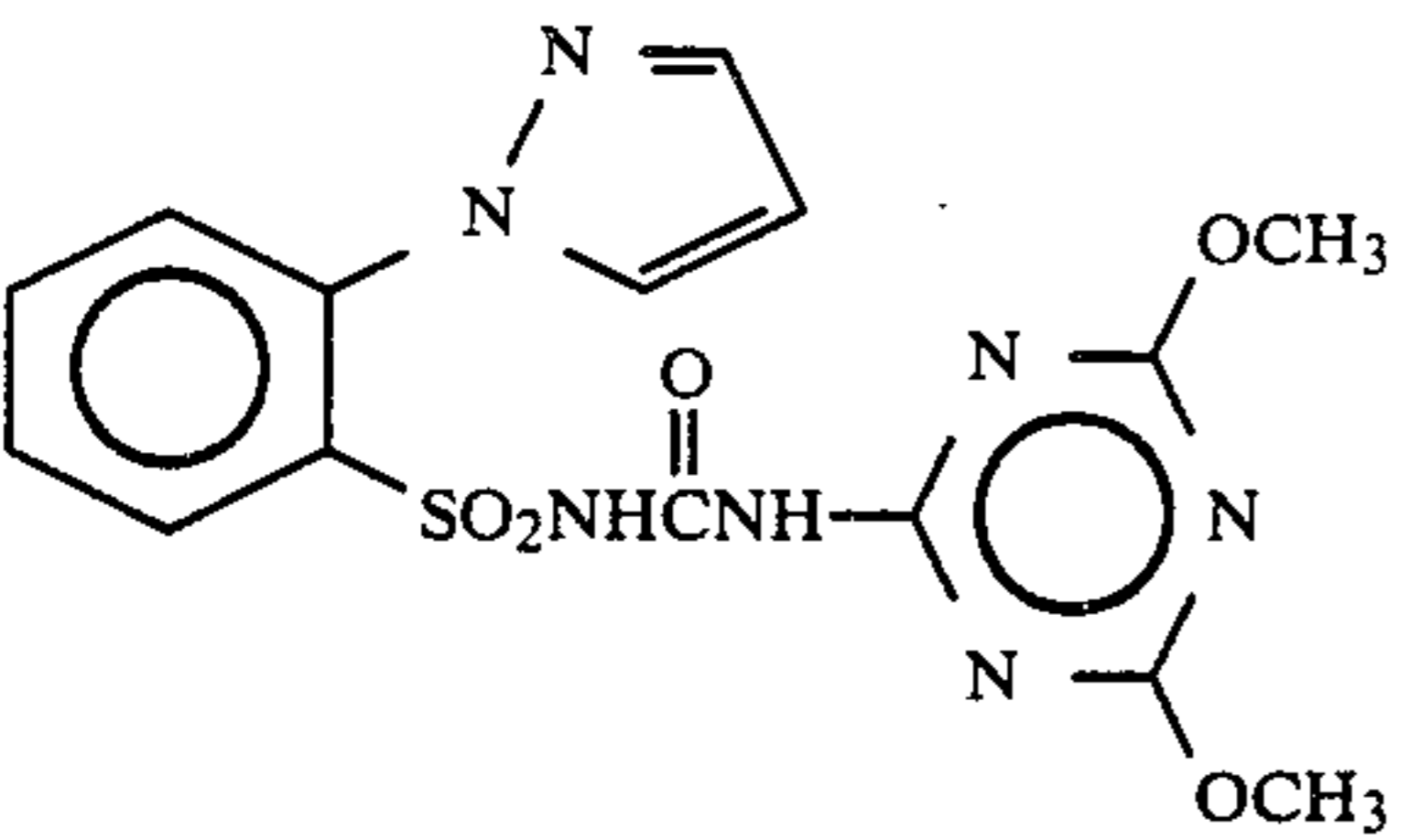
Compound 49
