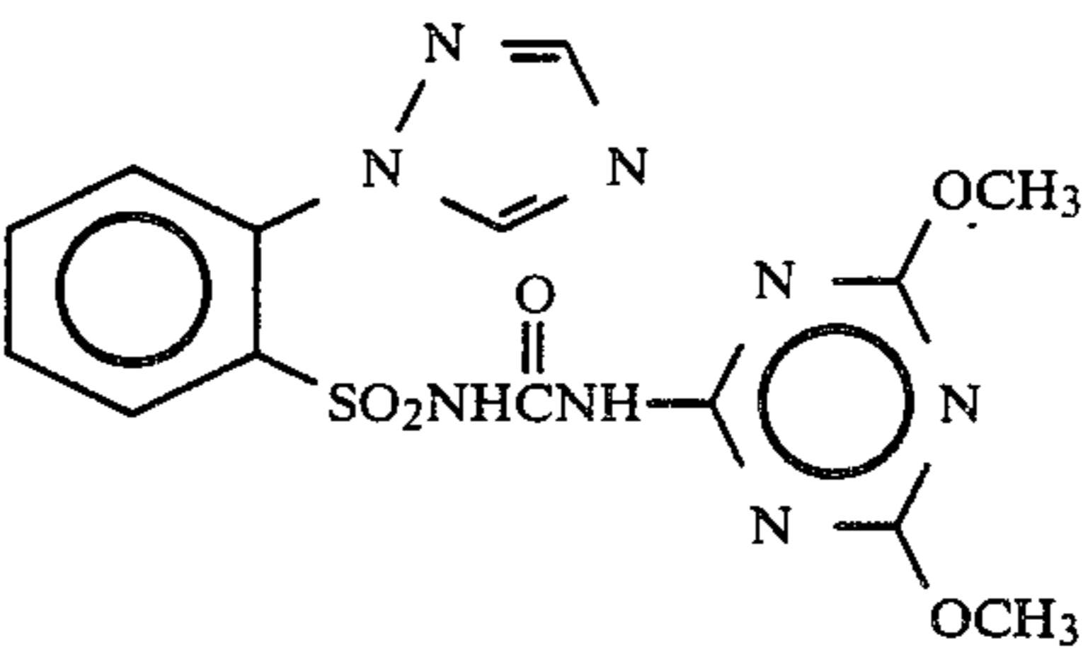
Compound 43
