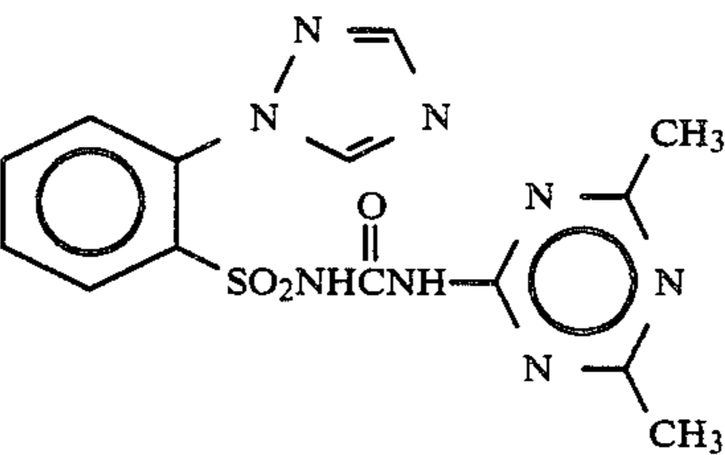
Compound 44
