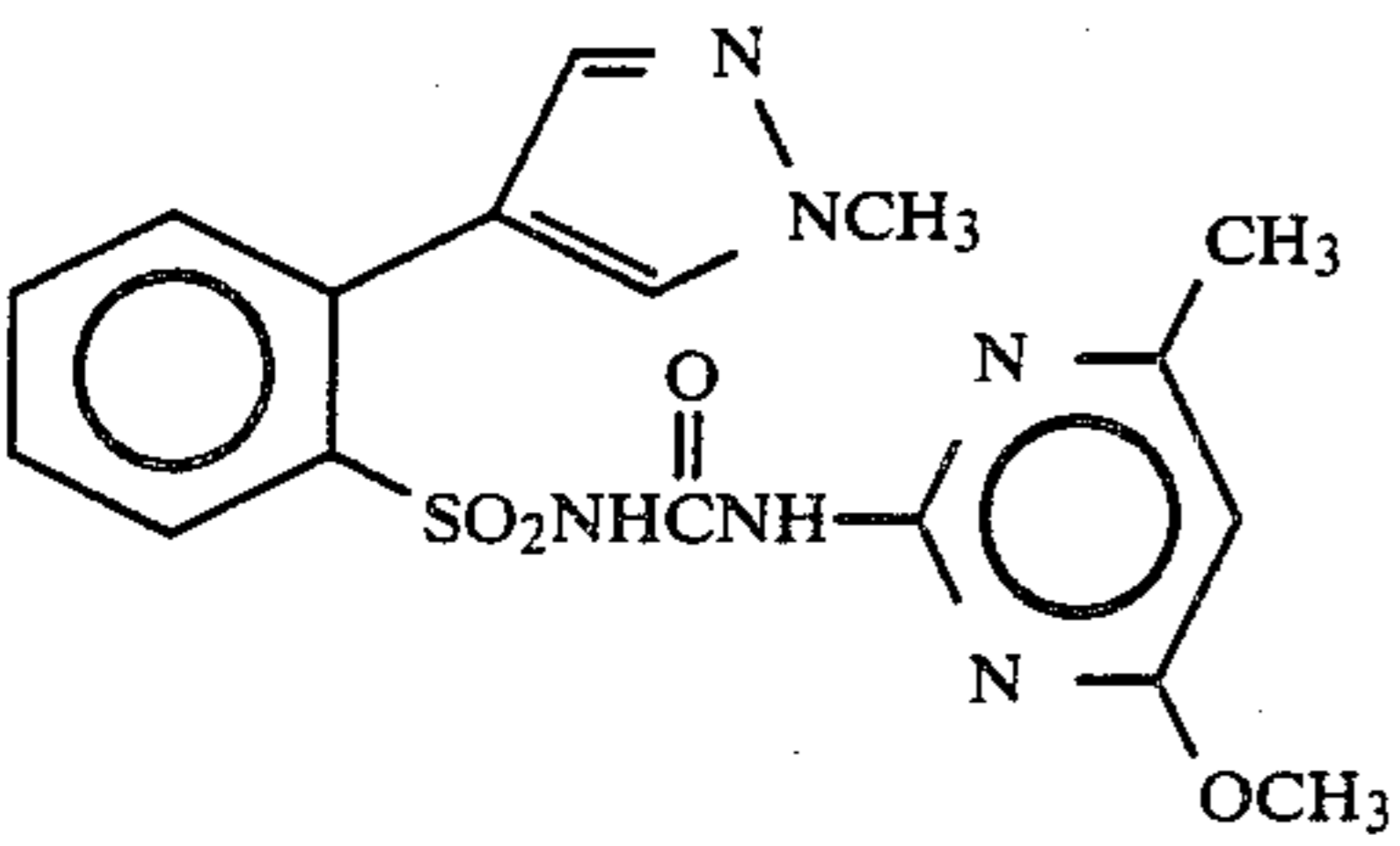
Compound 33
