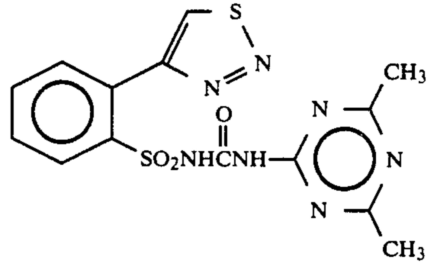
Compound 25
