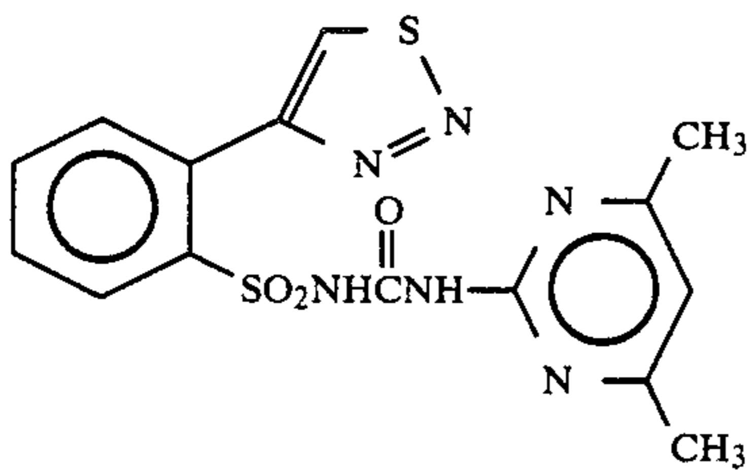
Compound 22
