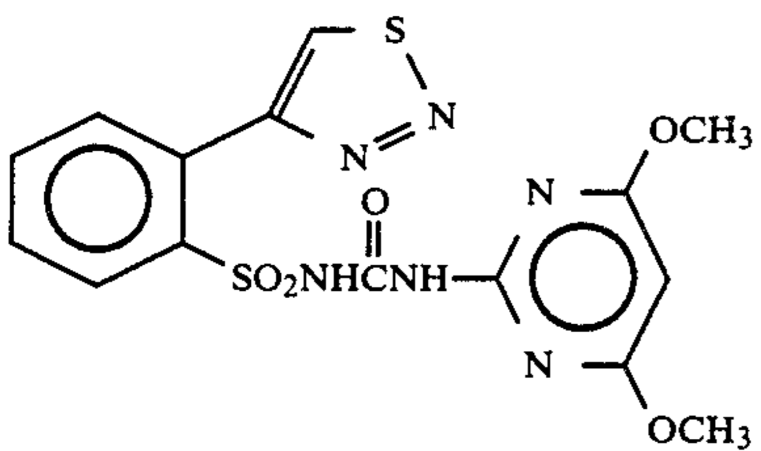
Compound 20
