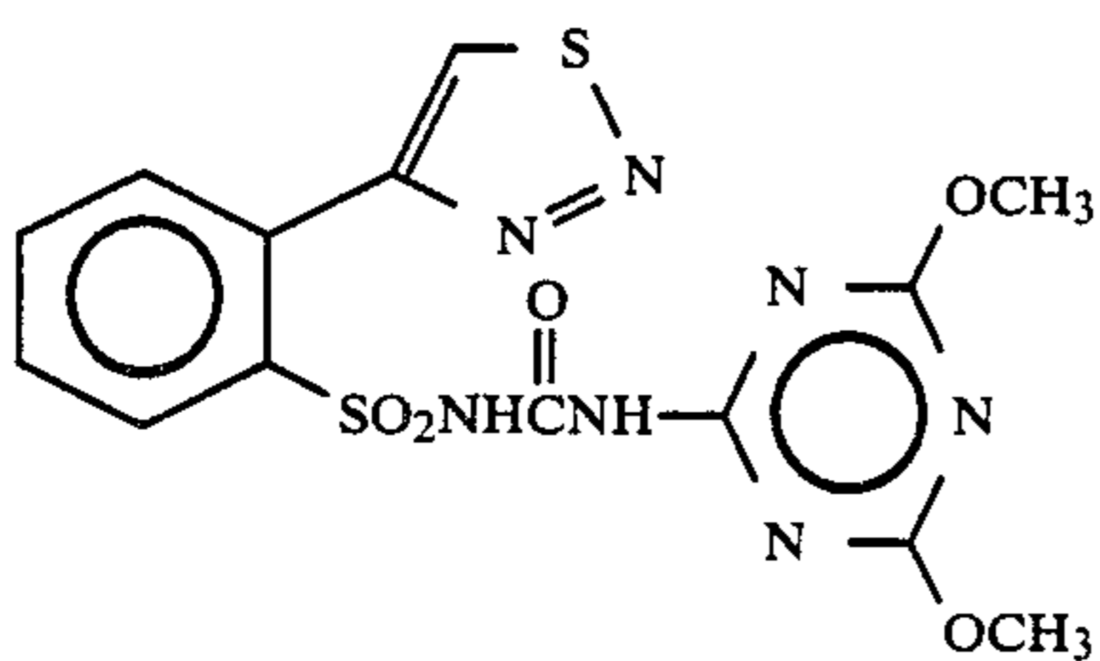
Compound 23
