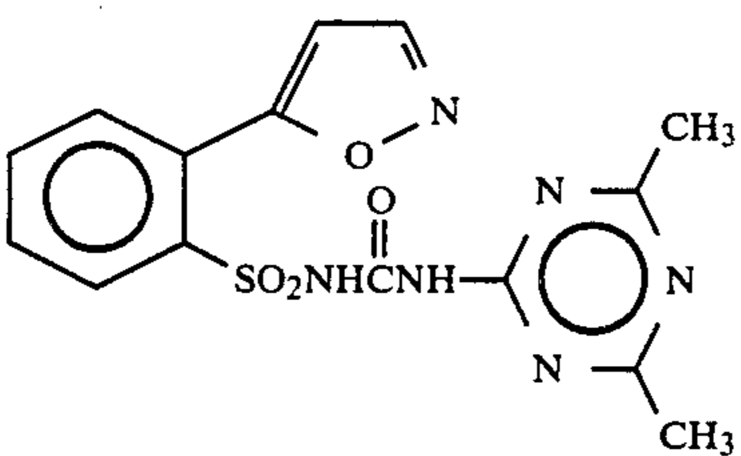
Compound 29
