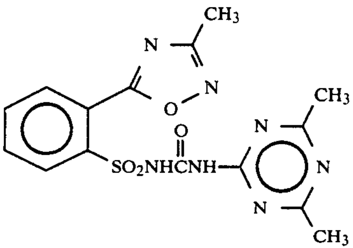
Compound 19
