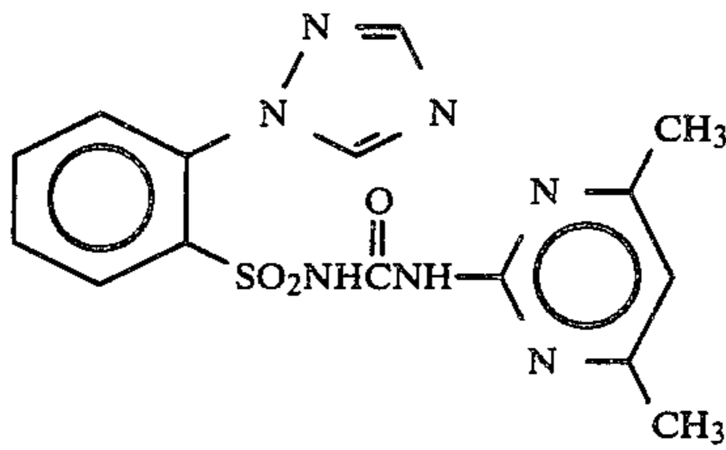
Compound 41
