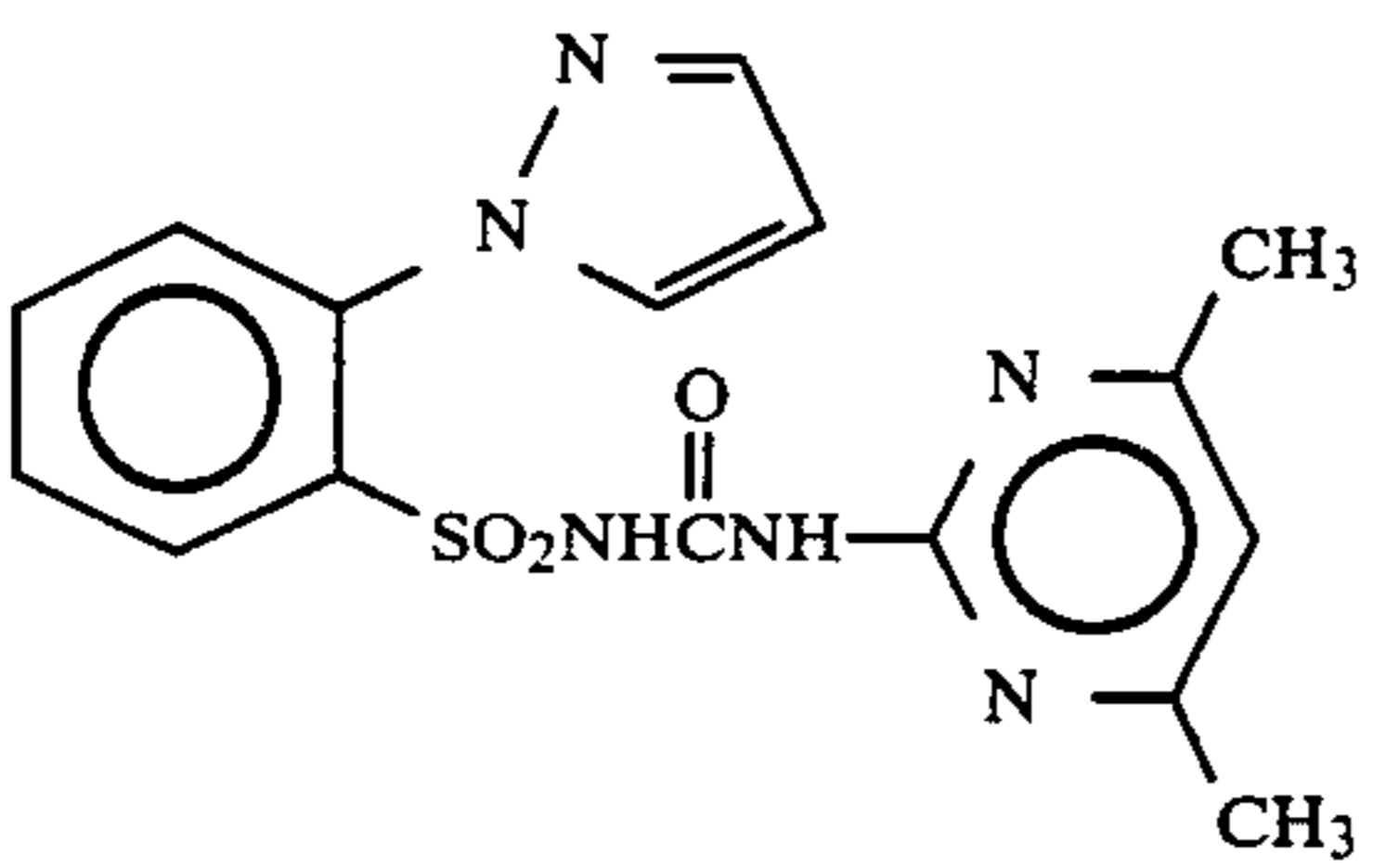
Compound 47
