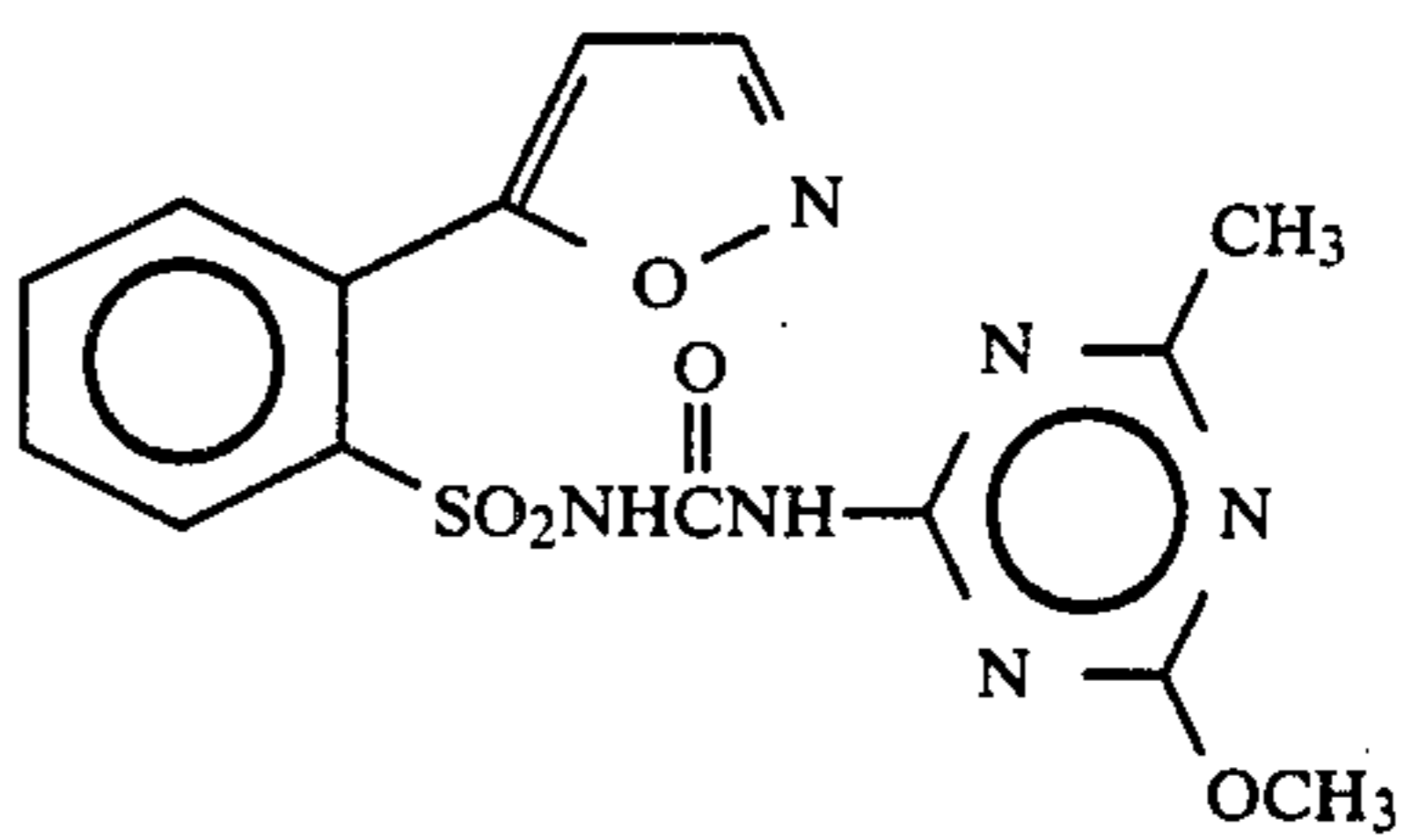
Compound 28
