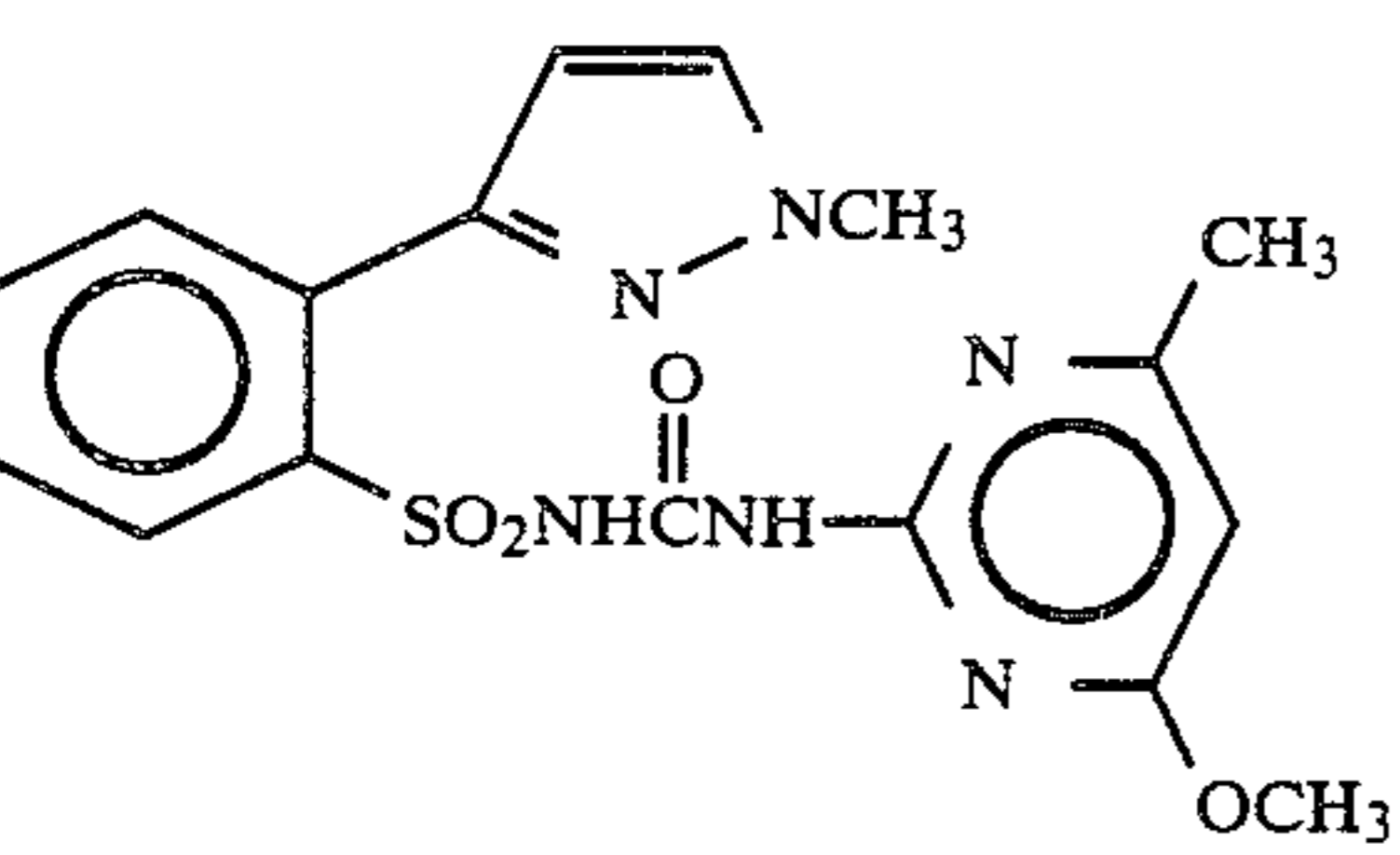
Compound 37
