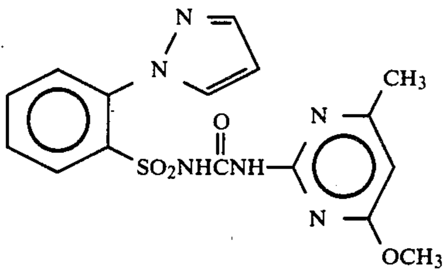
Compound 46
