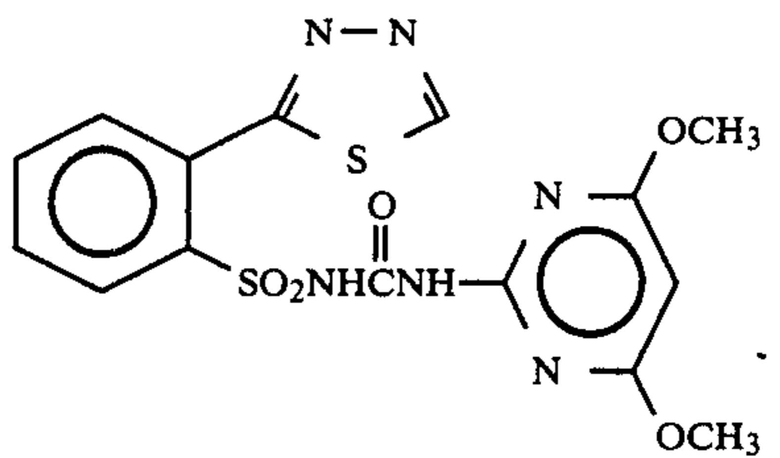
Compound 53
