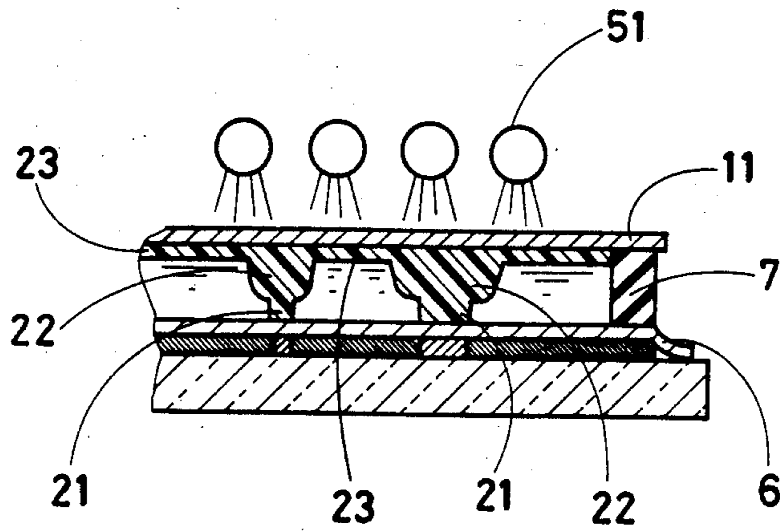
FIG. 10 PRIOR ART
