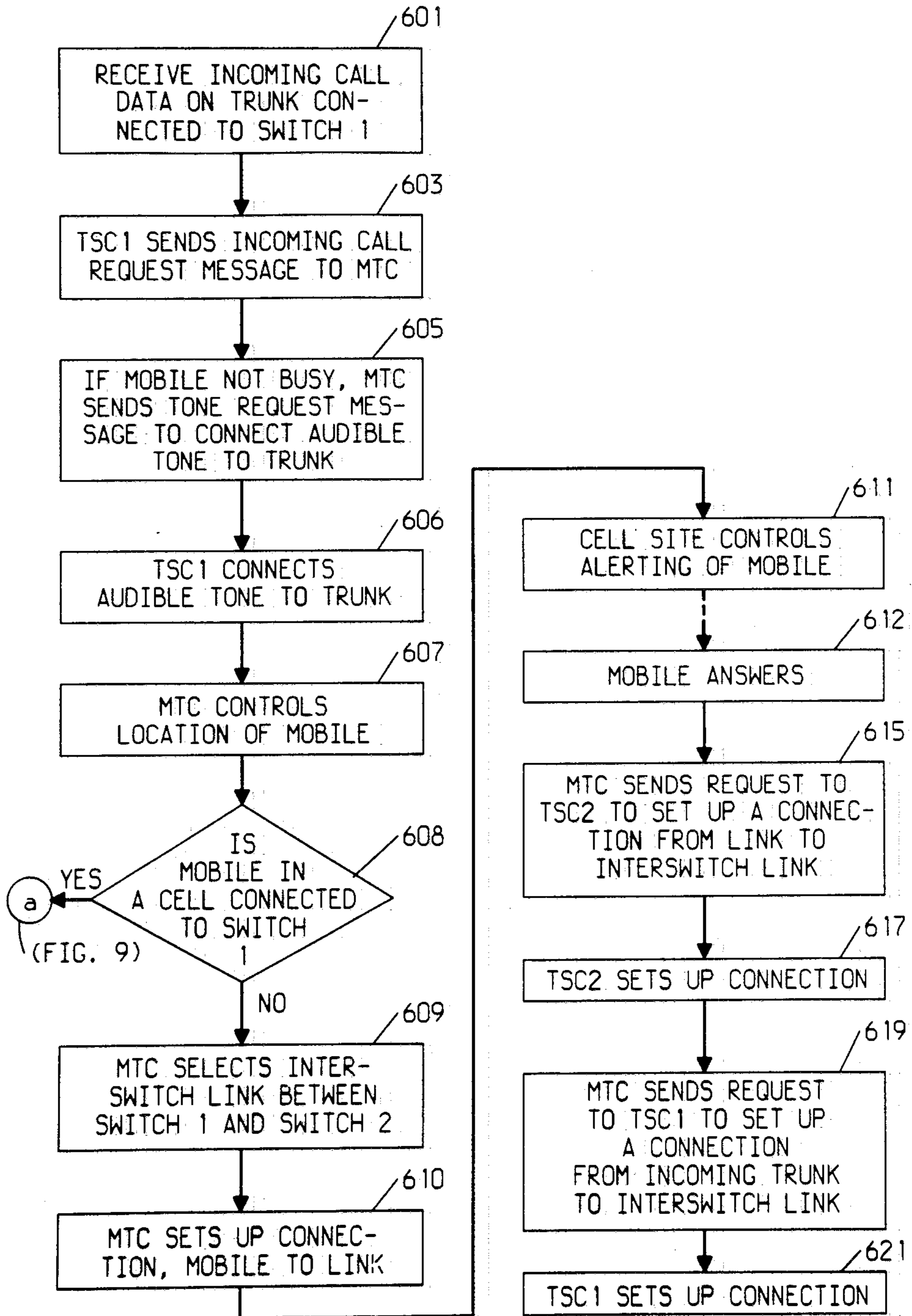
FIG. 15 INCOMING CALL: MULTISWITCH CONFIGURATION
