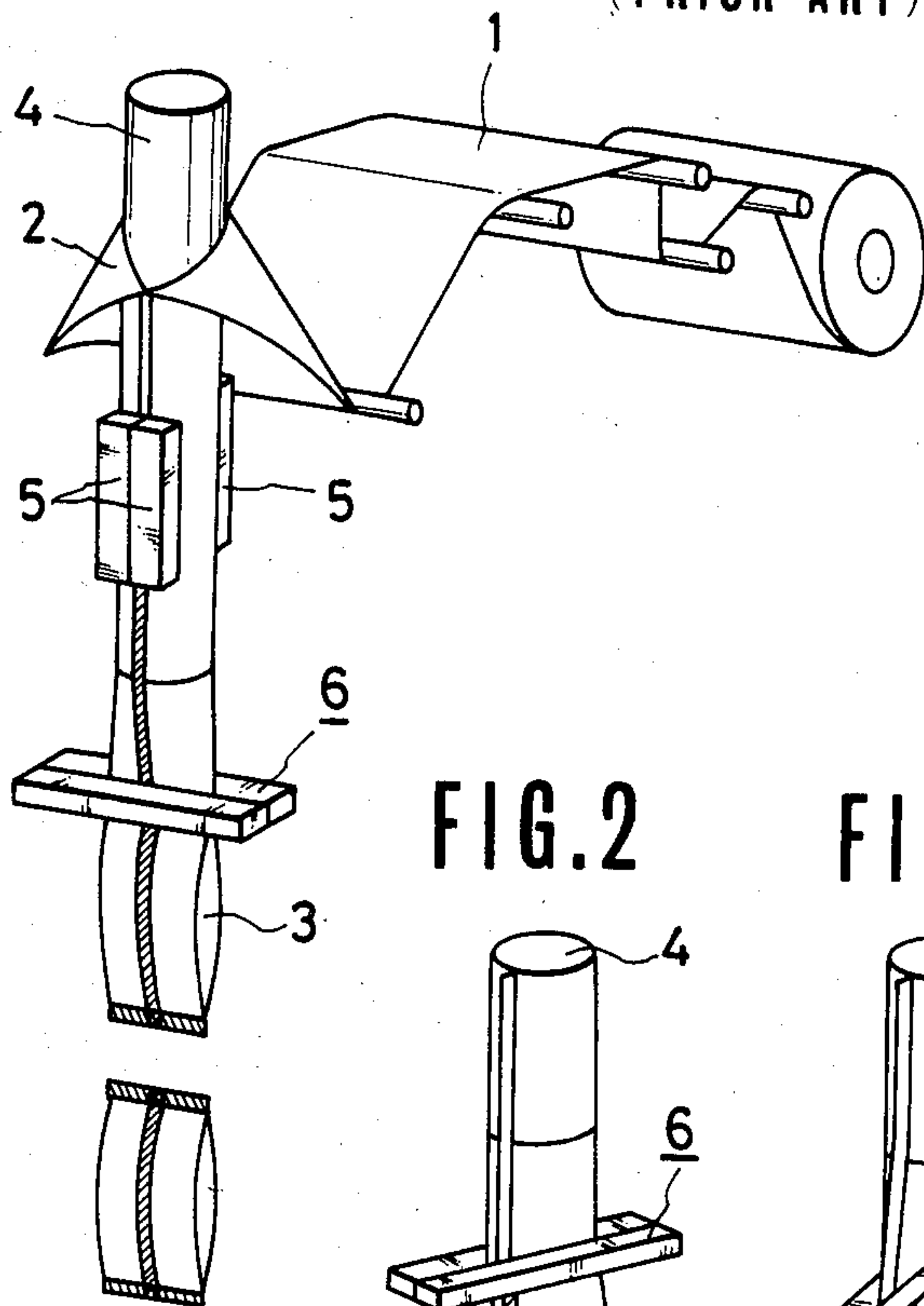
FIG. 1 (PRIOR ART)
