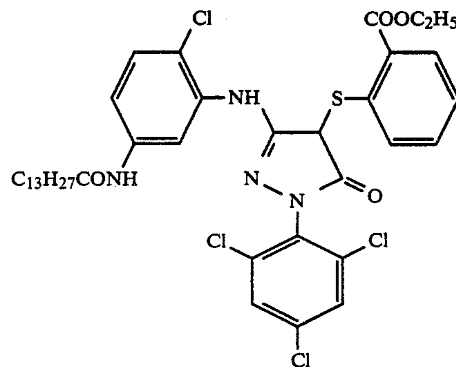
Comparative Magenta Coupler (B)
