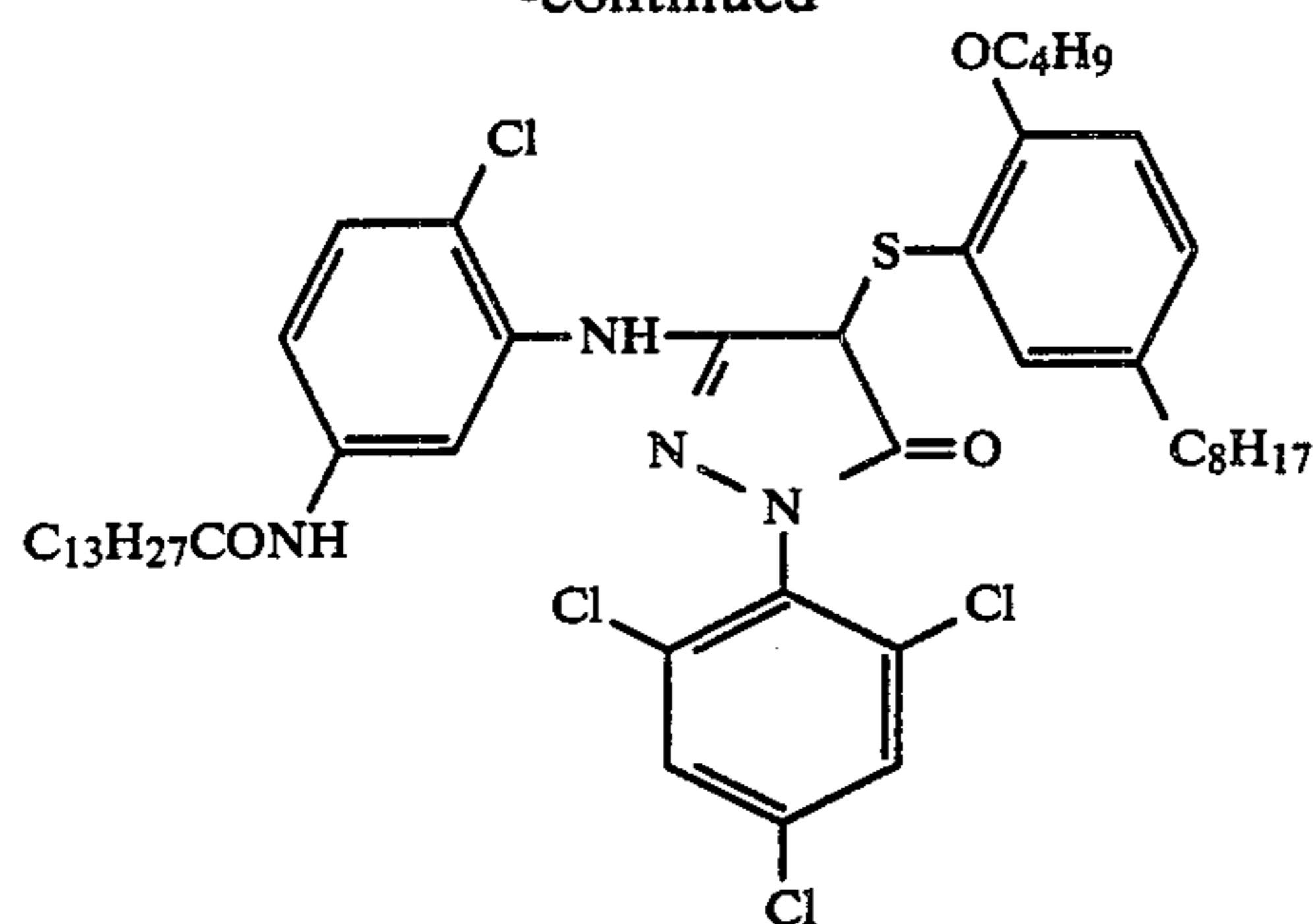
Comparative Magenta Coupler (C)
