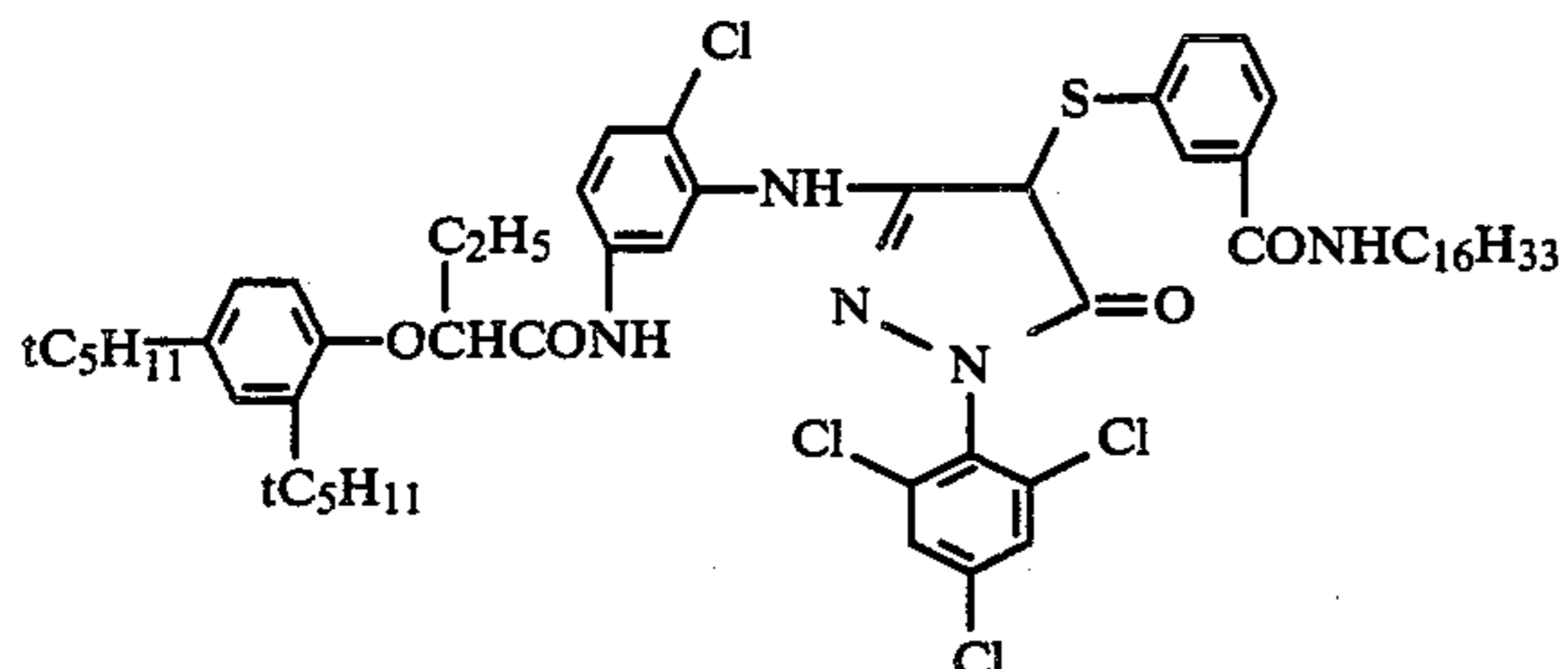
Comparative Magenta Coupler (C)
