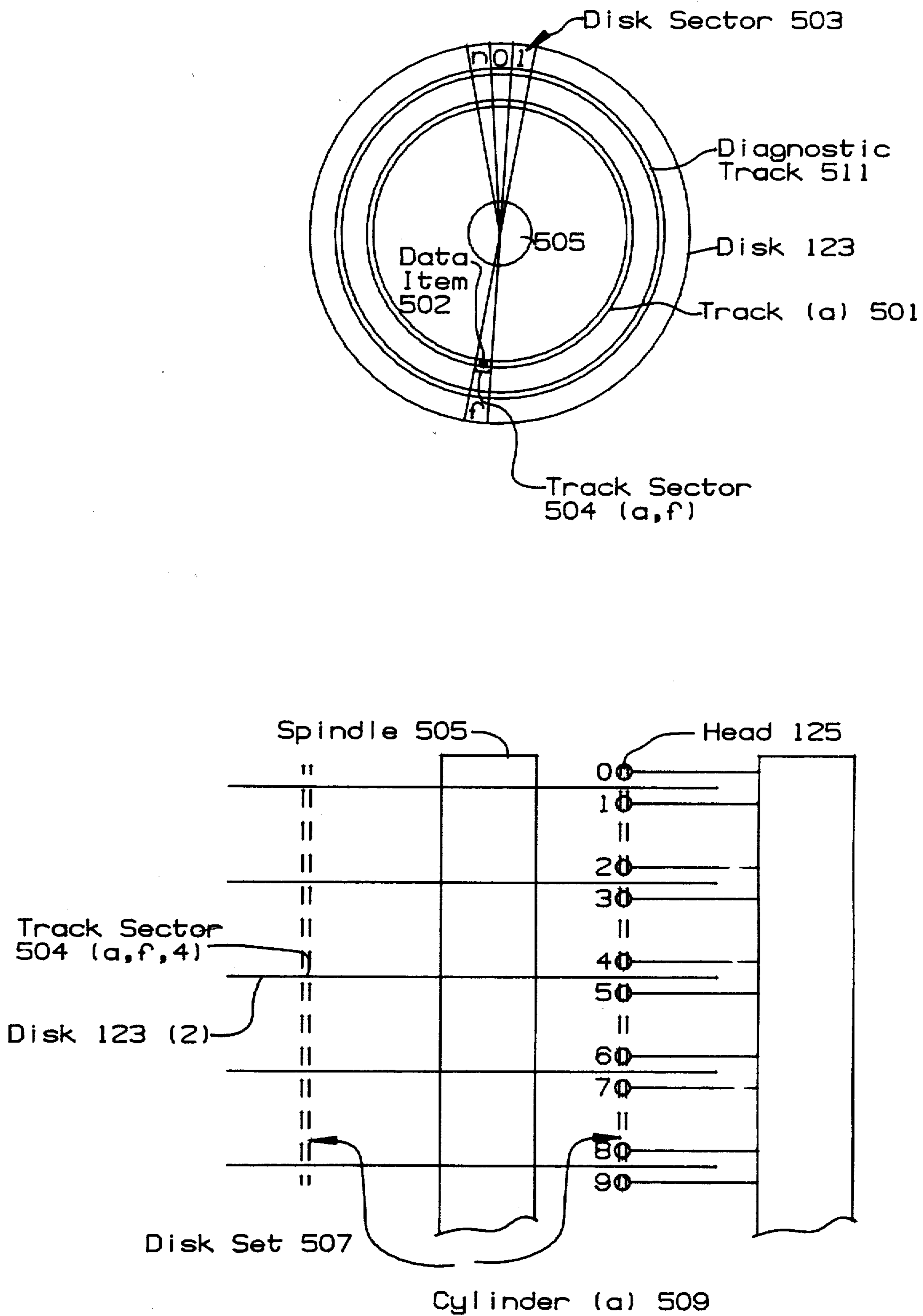
Fig.5: Disk Structure
