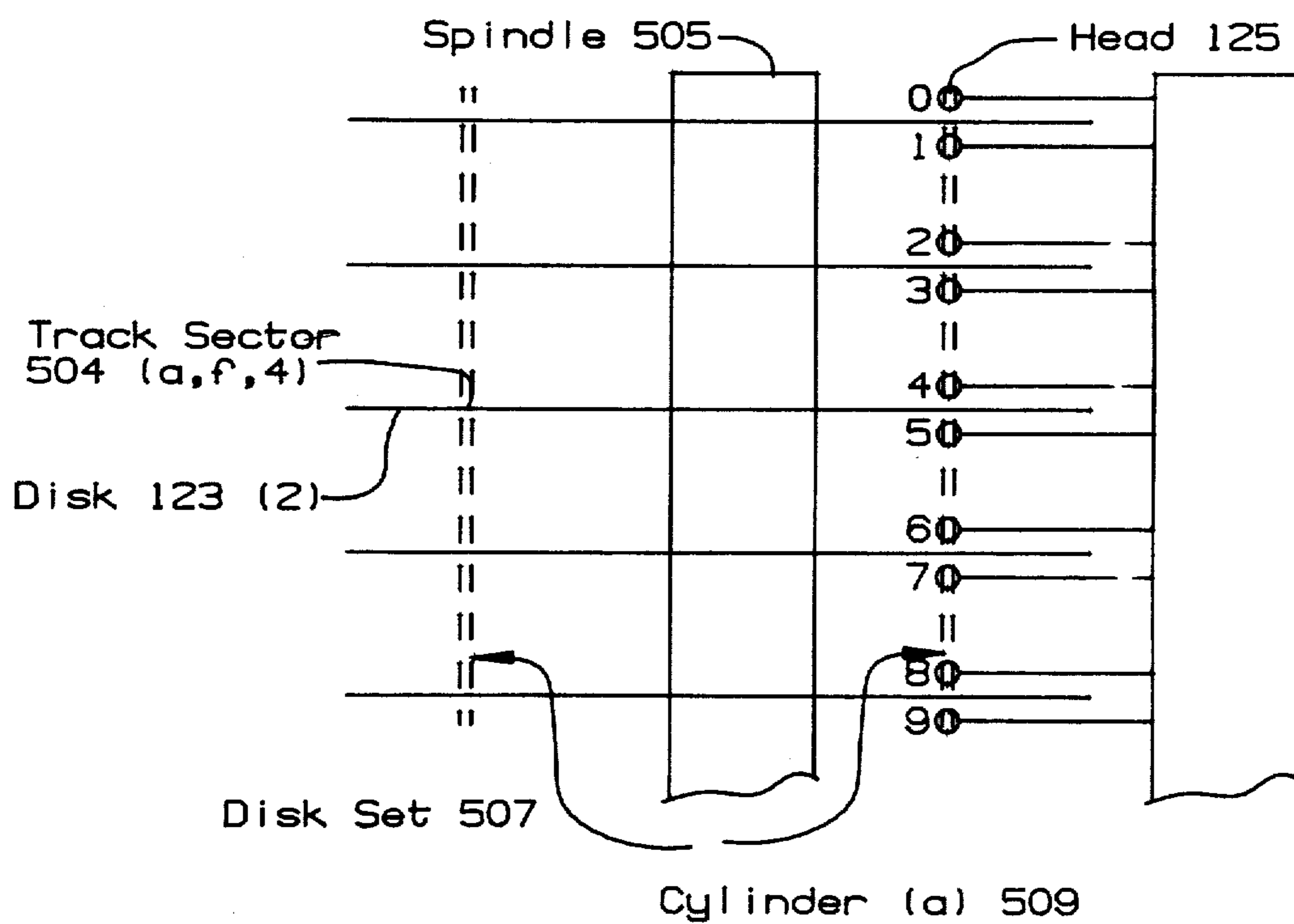
Fig.5: Disk Structure
