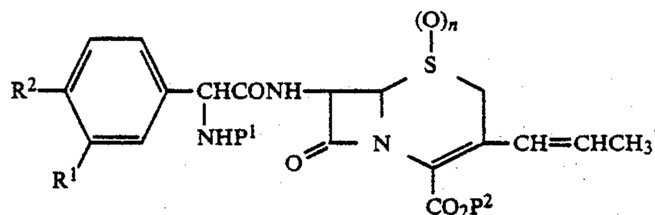
Formula XIII
