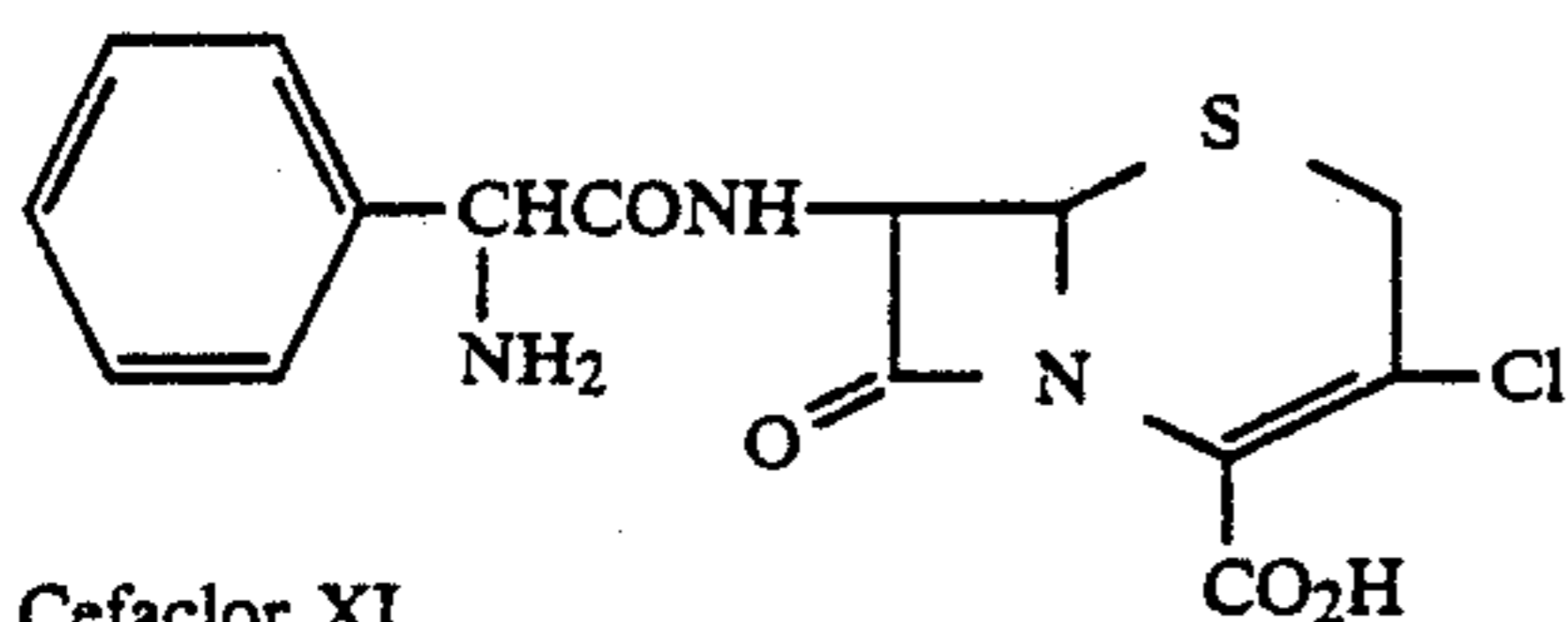
Cefaclor XI
