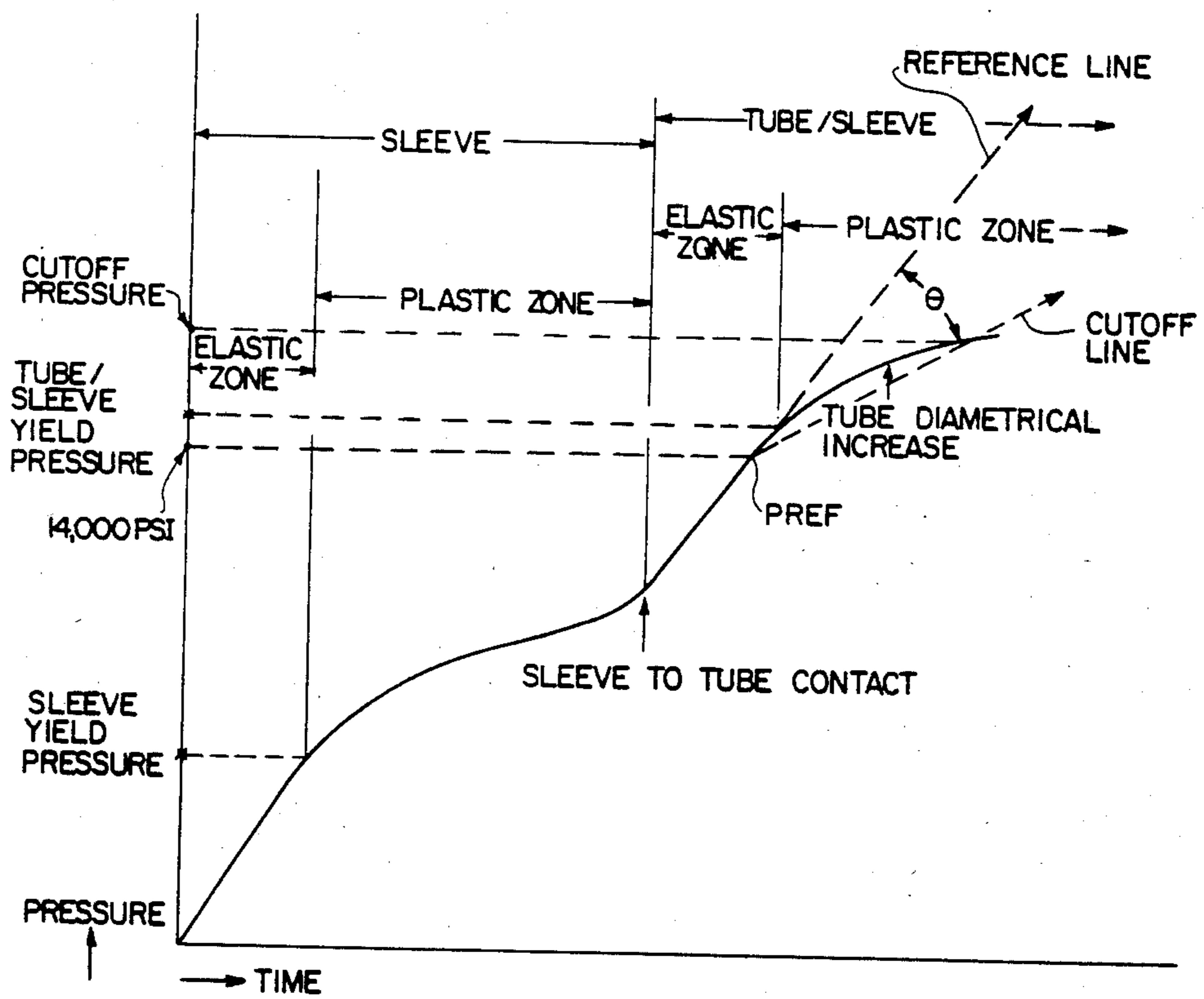
TUBE/SLEEVE HYDRAULIC EXPANSION
