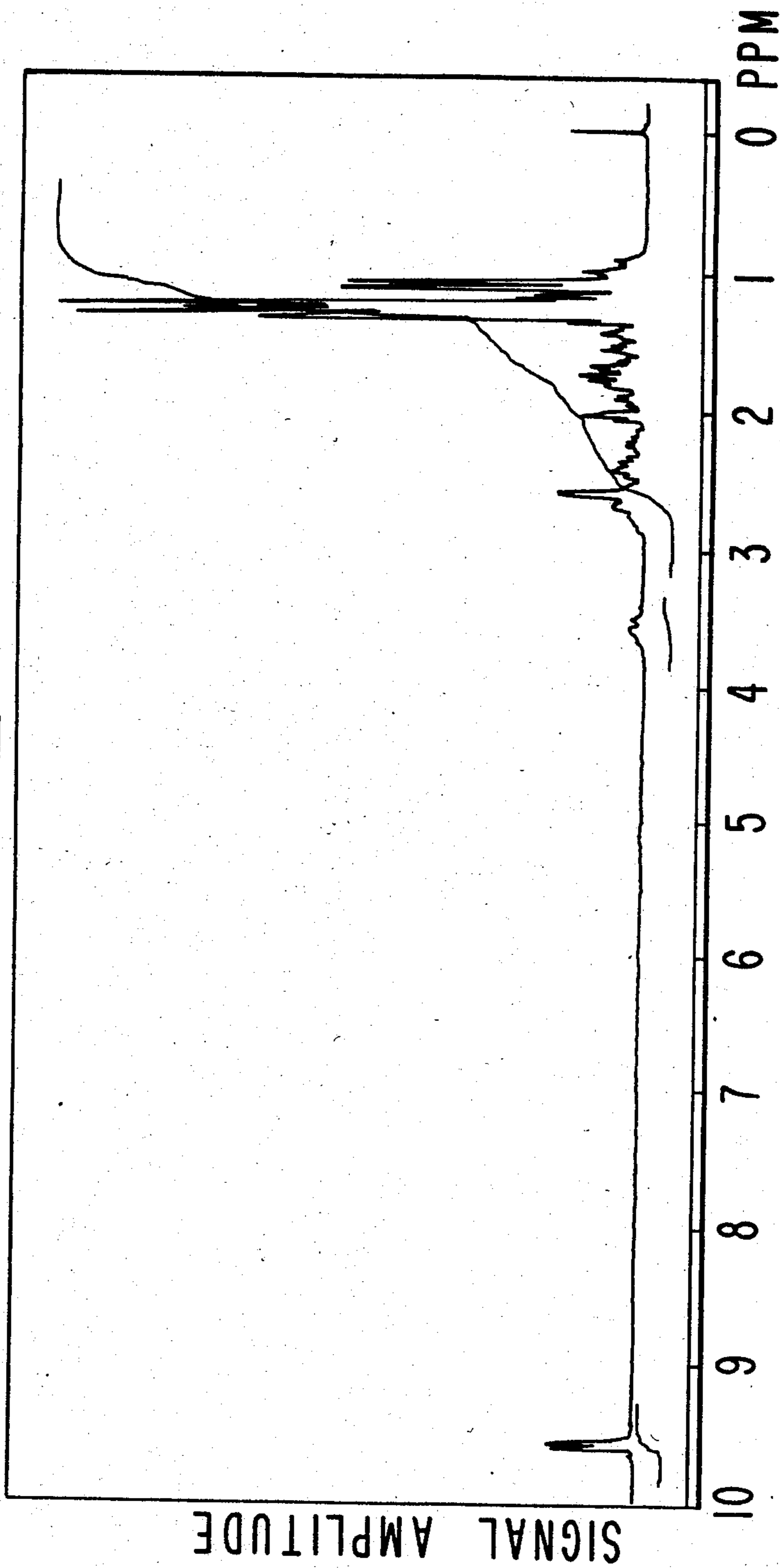
NMR SPECTRUM FOR EXAMPLE II.
