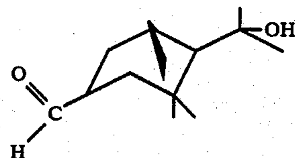
produced according to Example II. (Conditions: Field strength: 100 MHz; Solvent: CFC1 3 ).
