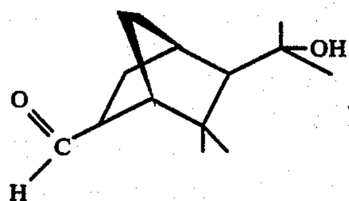
FIG. 7 is the NMR spectrum for a mixture of compounds having the structures:
