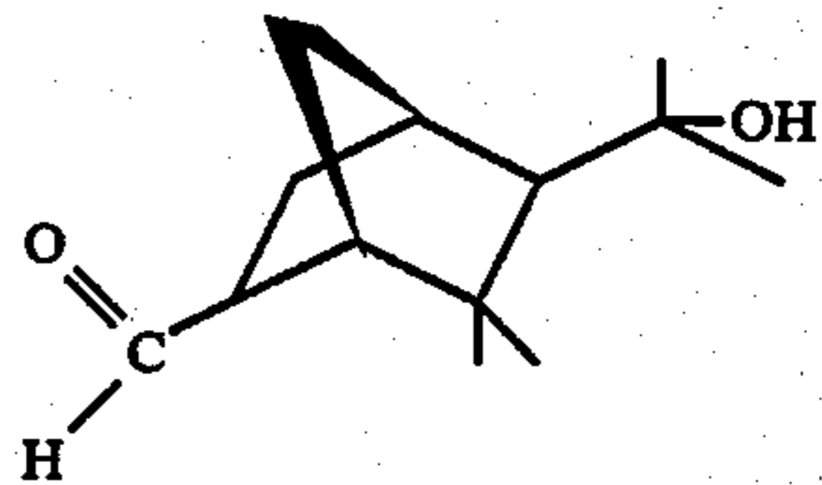
FIG. 9 is the GLC profile for bulked fractions 5 and 6 of the first distillation of the reaction product of Example III containing the compound having the structure:
