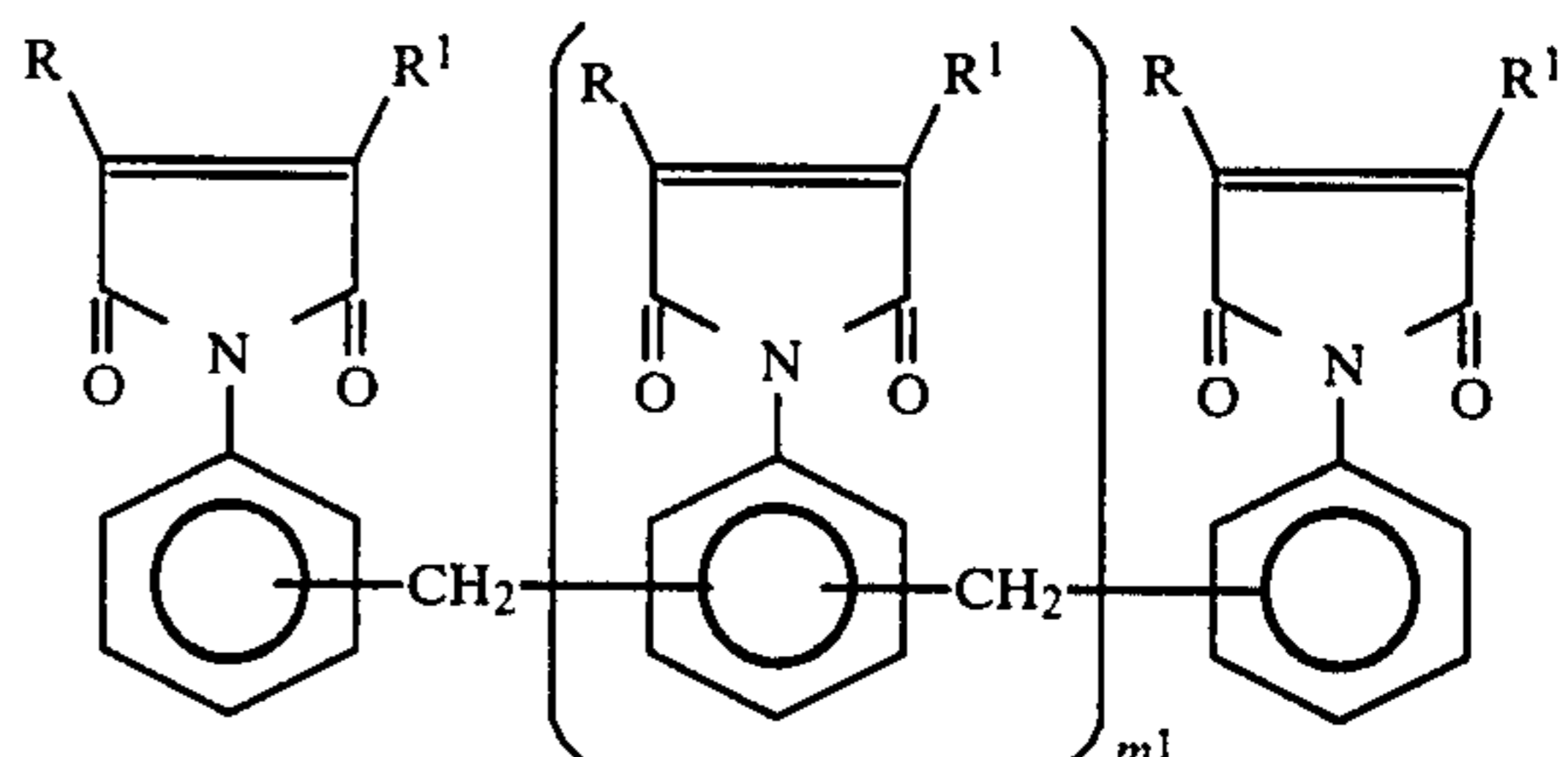
FORMULA VII
