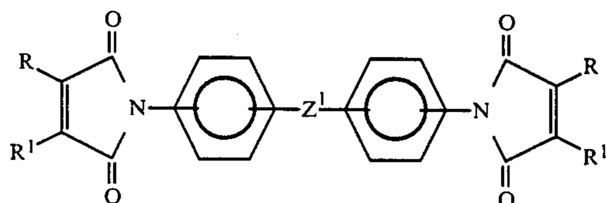
FORMULA VI
