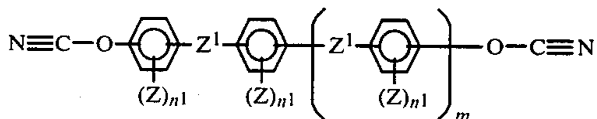
FORMULA IIIB
