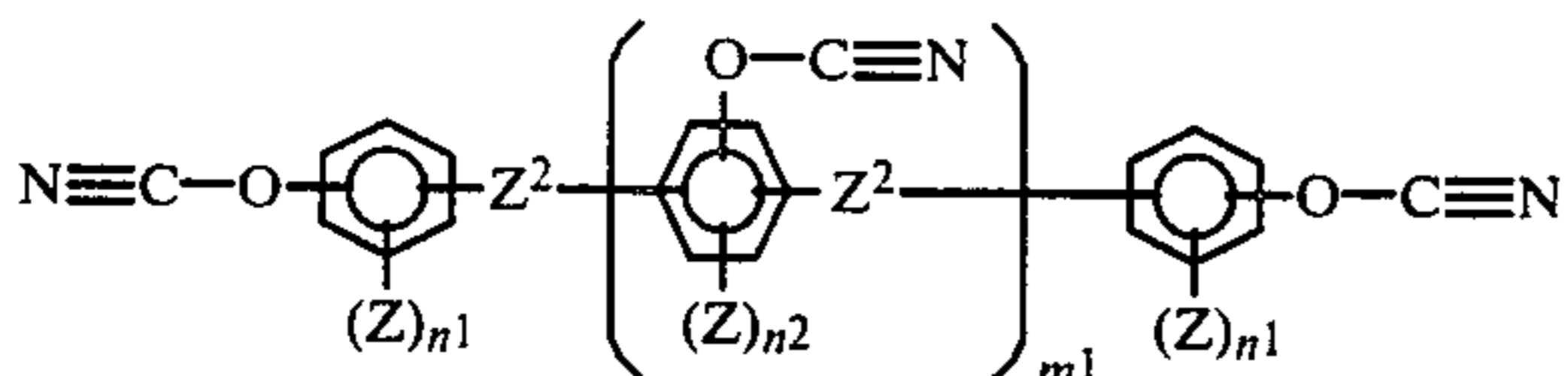
FORMULA IIIC
