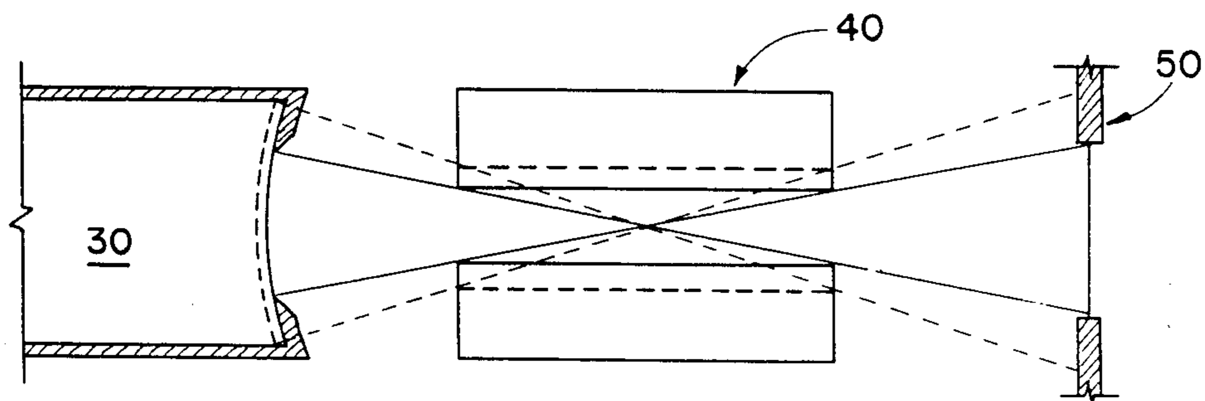
FIG. 9 (PRIOR ART)
