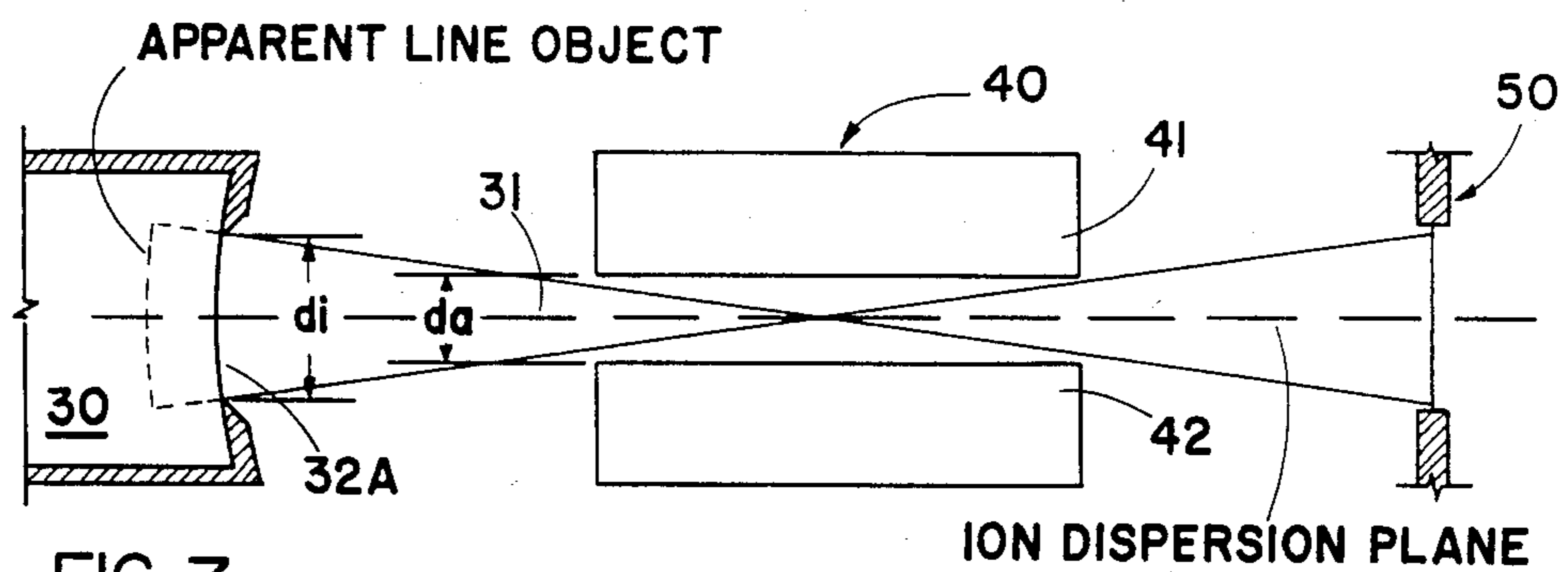
FIG. 7 (PRIOR ART)
