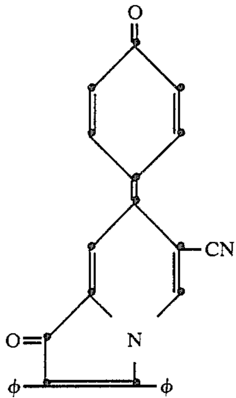
6-(4-azastyryl)-1,2-diphenyl-7-(4-oxo-1-phenylidene)-3(7H)-indolizinone
