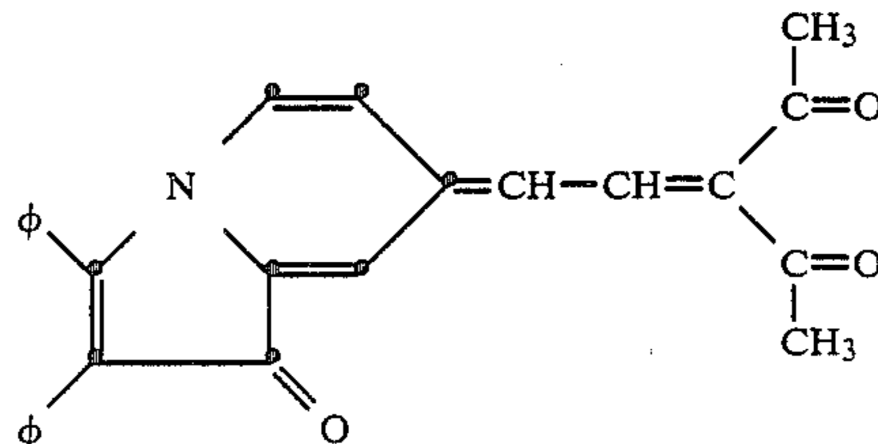
7-(3,3-diacetyl-1-propenylidene)-2,3- diphenyl-1-(7H)-indolizone
