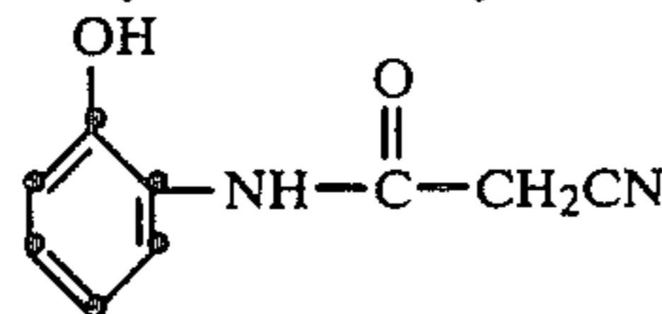
2-cyanoacetamidophenol
