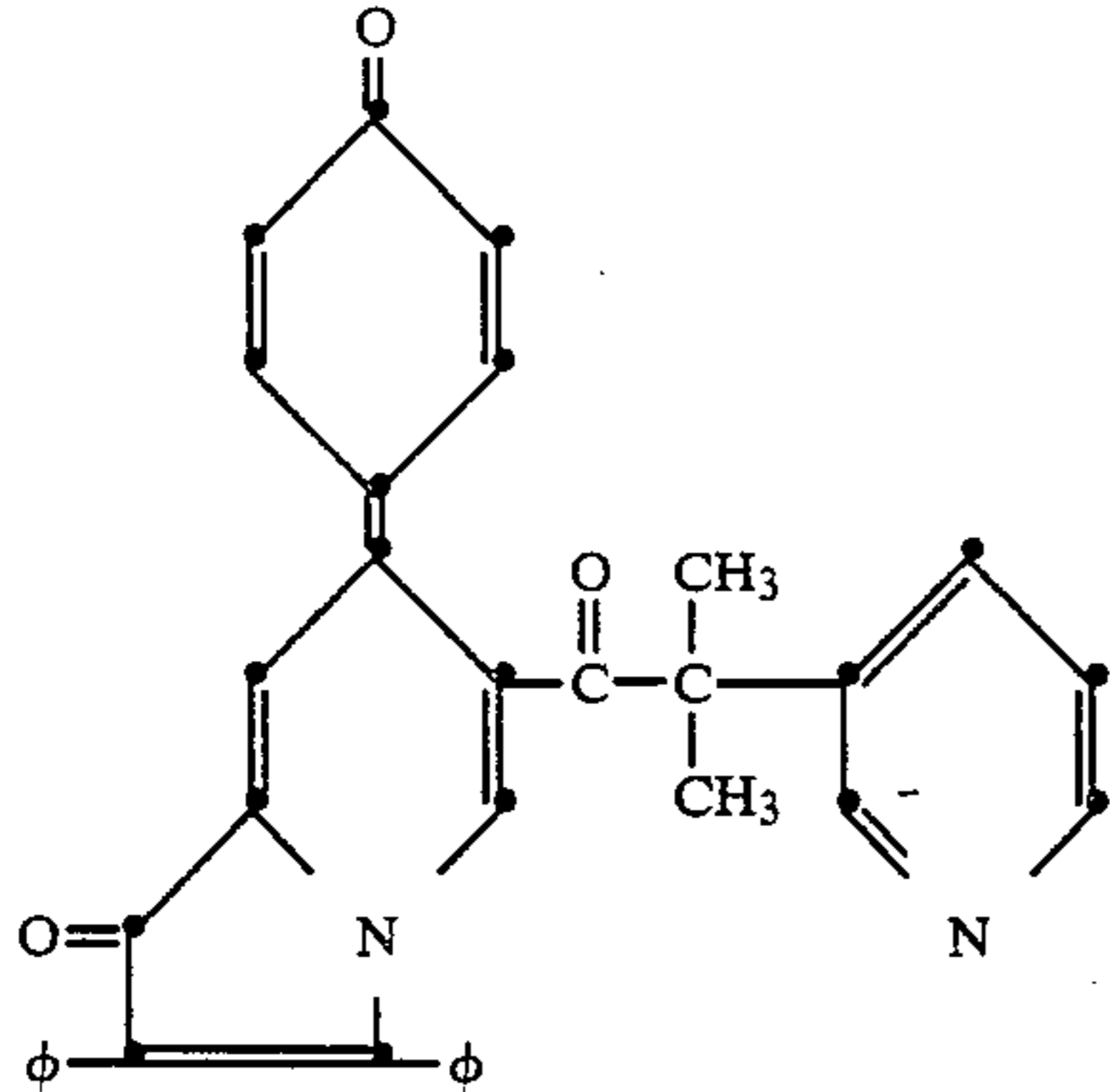
1,2-bis[6,6'-[2,3-diphenyl-7-(4-oxo-1-phenylidene)-1(7H)-indolizine]-3-phenylidene]-1(7H)-indolizine
