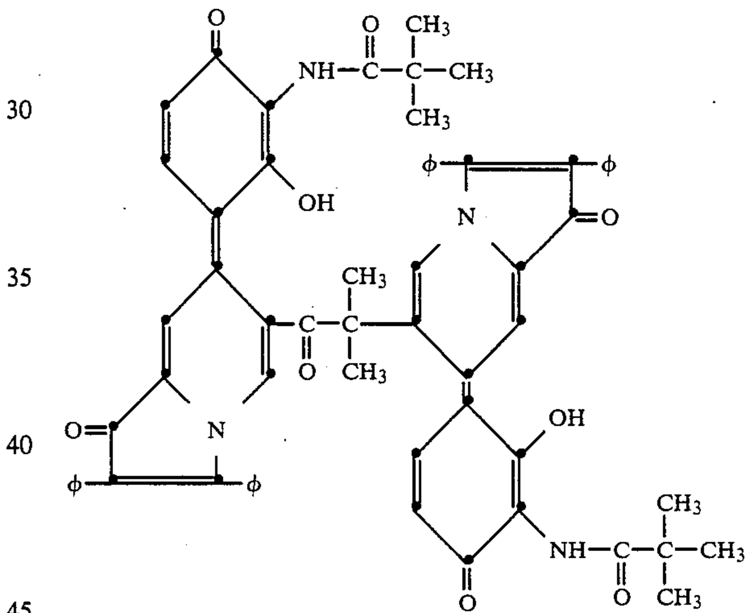
20 1,2-bis-{6,6'-[7-[3-(4-tert-butylbenzamido)-2-hydroxy-4-oxo-1-phenylidene]}-2,3-diphenyl-1(7H)-indolizinonyl}-2-methyl-1-oxo-propane
