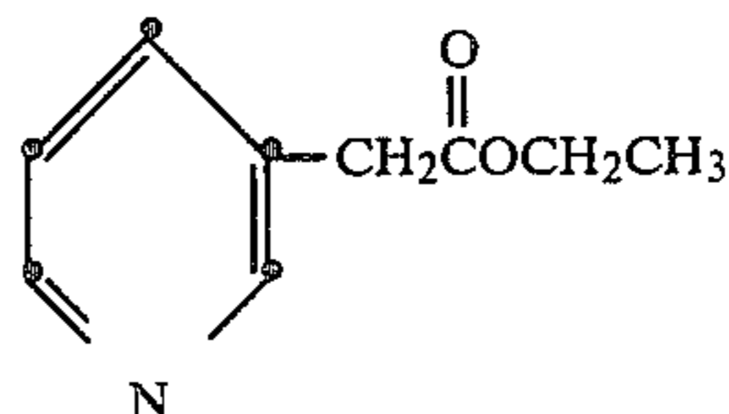
Ethyl 3-pyridylacetate:
