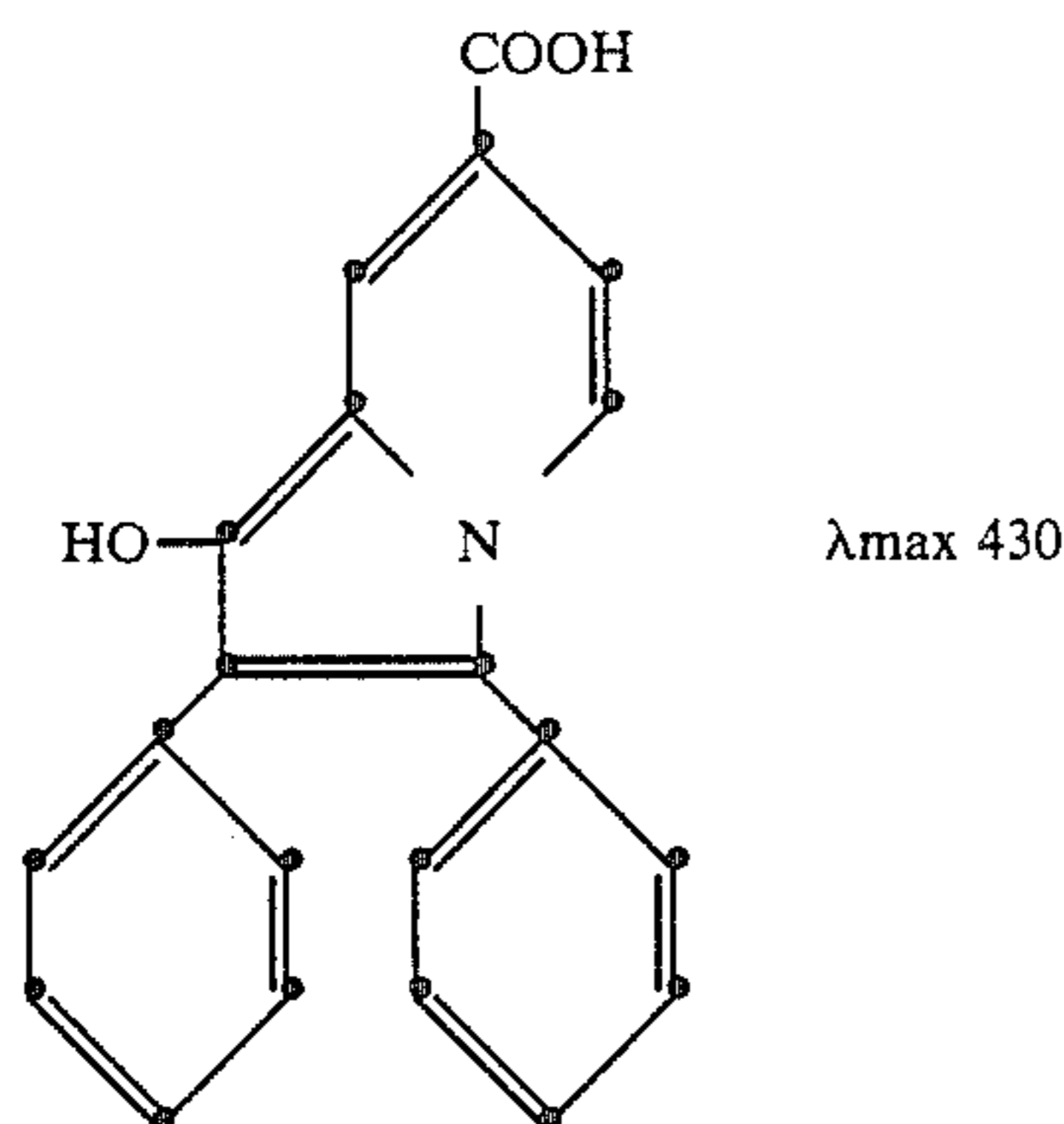
7-carboxyl-2,3-diphenyl-1-indolizino
