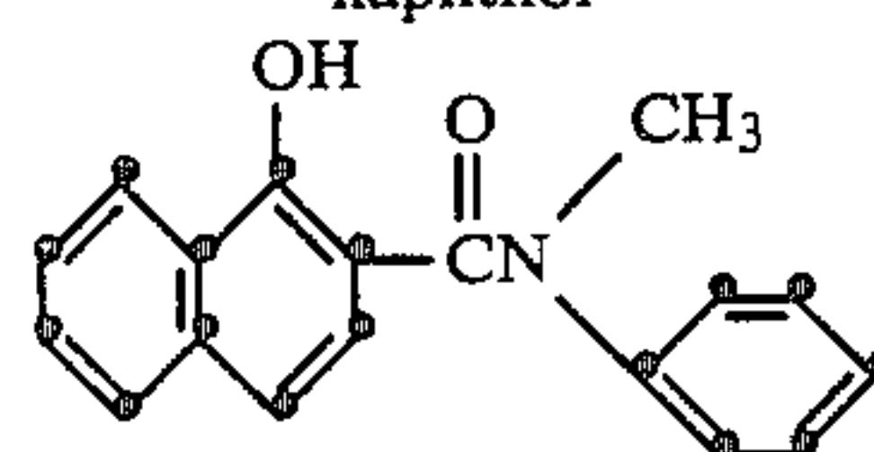
2-(N-methylanilinocarbonyl)-1-naphthol
