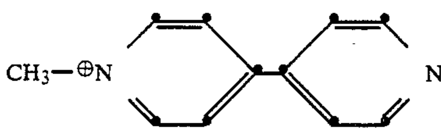
1-Methyl-4-(4-pyridyl)pyridinium-p-toluene-sulfonate:
