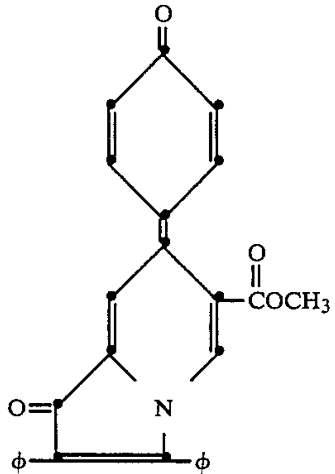
2,3-diphenyl-6-[2-methyl-2-(3-pyridyl)propionyl]-7-(4-oxo-1-phenylidene)-1(7H)-indolizine
