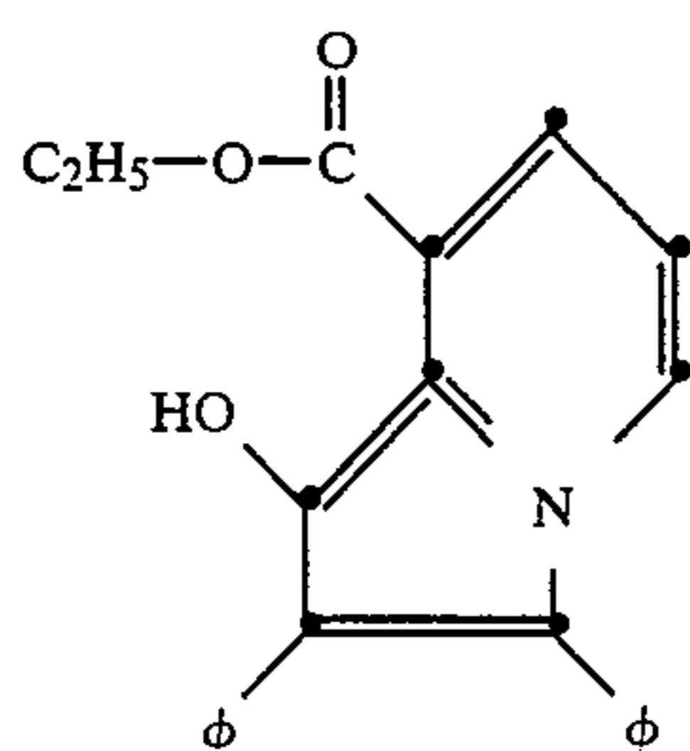
7-carboxy-2,3-diphenyl-1-indolizinol
