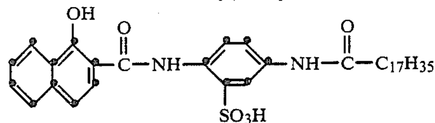
2-(2-sulfonyl-4-stearoylamino anilino-carbonyl)-1-naphthol
