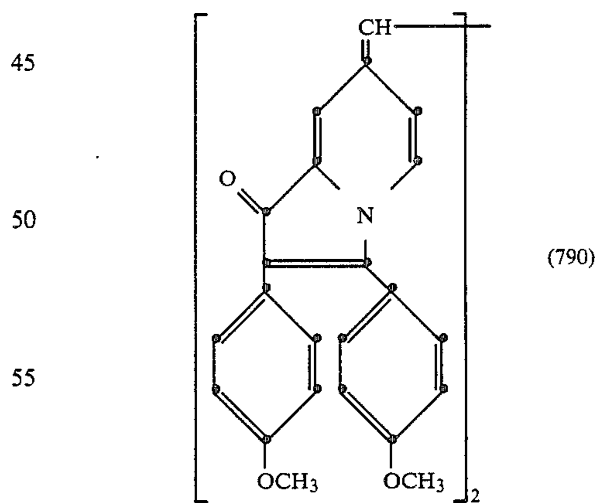
1,2-bis[2,3-di-(4-methoxyphenyl)-1(7H)-indolizinonylidene]ethane
