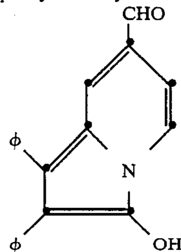
7-formylmethylidene-2,3-diphenyl-1(7H)-indolizinone
