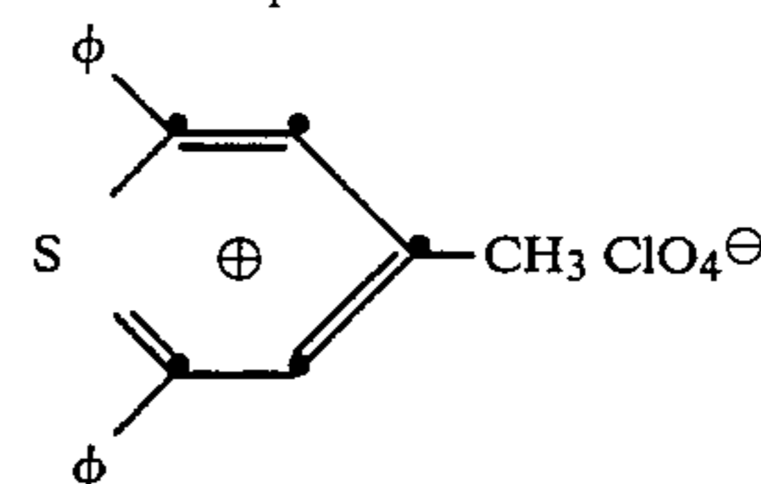
2,6-Diphenyl-4-methylthiopyrylium perchlorate M-3
