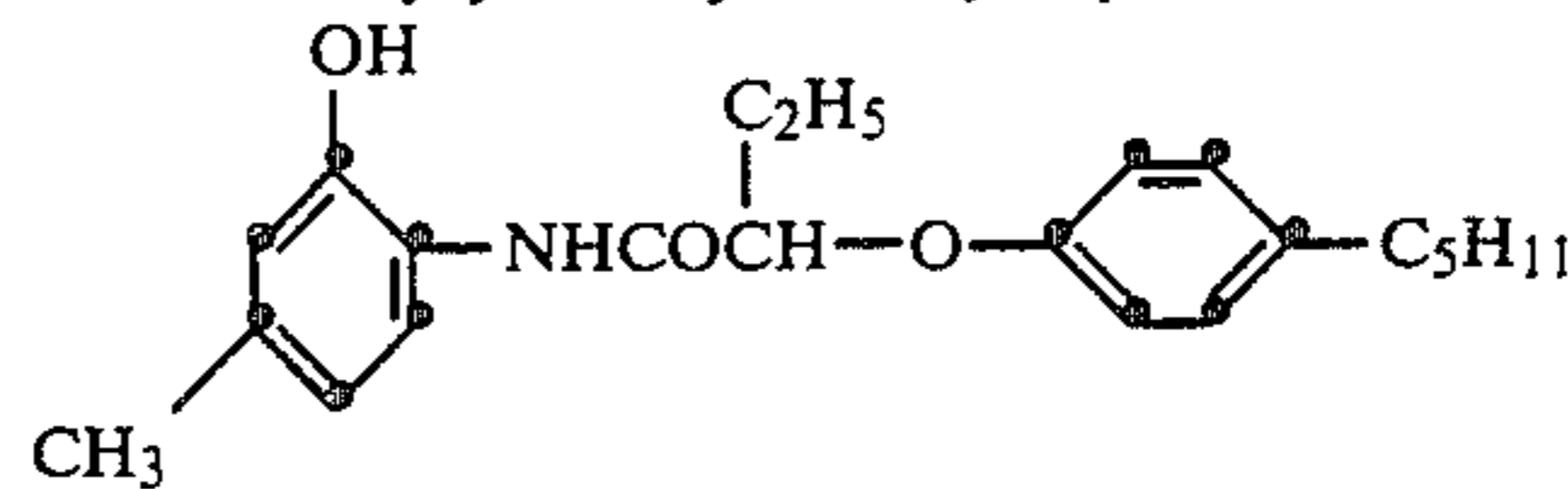
2-[ \alpha -(4'-tert.-amylphenoxy)-butyrylamino]-5-methyl-1-phenol
