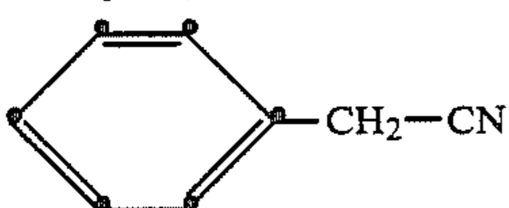
phenylacetonitrile
