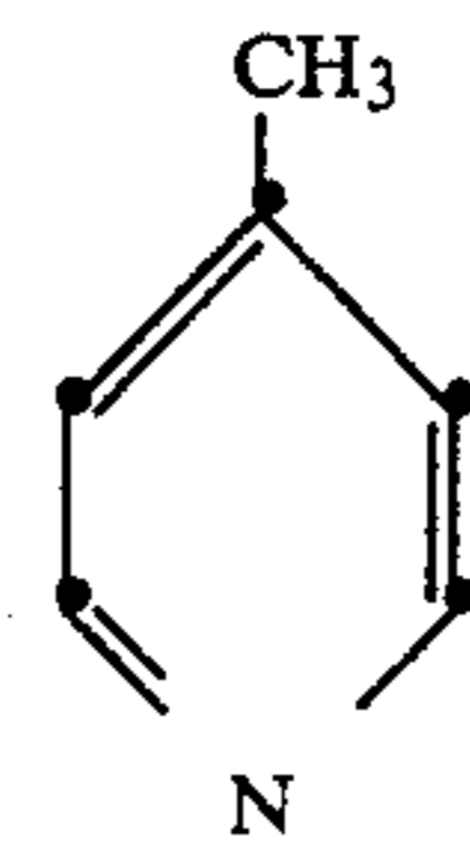
4-Picoline:
