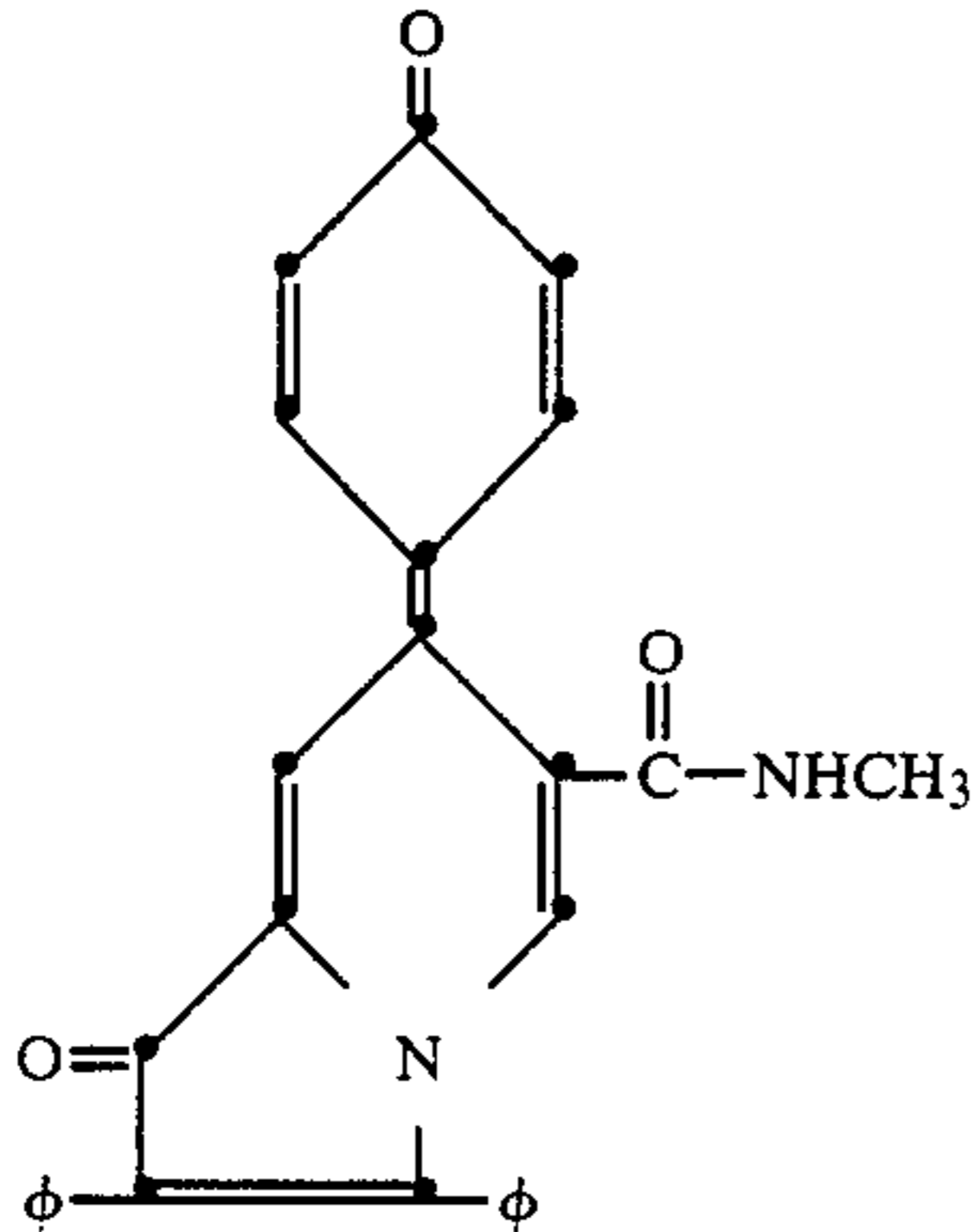
2,3-diphenyl-6-methoxycarbonyl-7-(4-oxo-1-phenylidene)-1(7H)-indolizine
