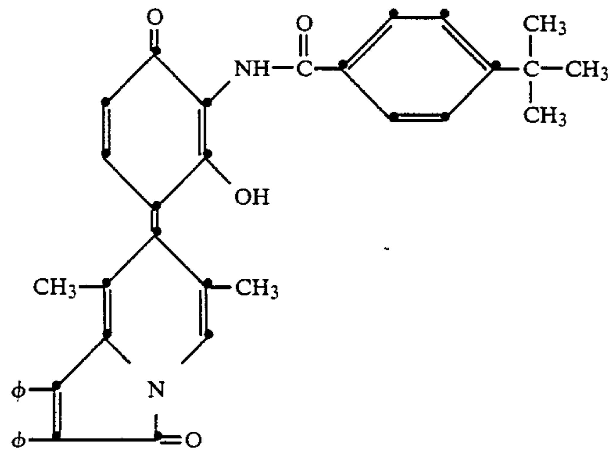
7-[3-(4-tert-butylbenzamido)-2-hydroxy-4-oxo-1-phenylidene]-6-diethylcarbamyl-2,3-diphenyl-1(7H)-indolizinone
