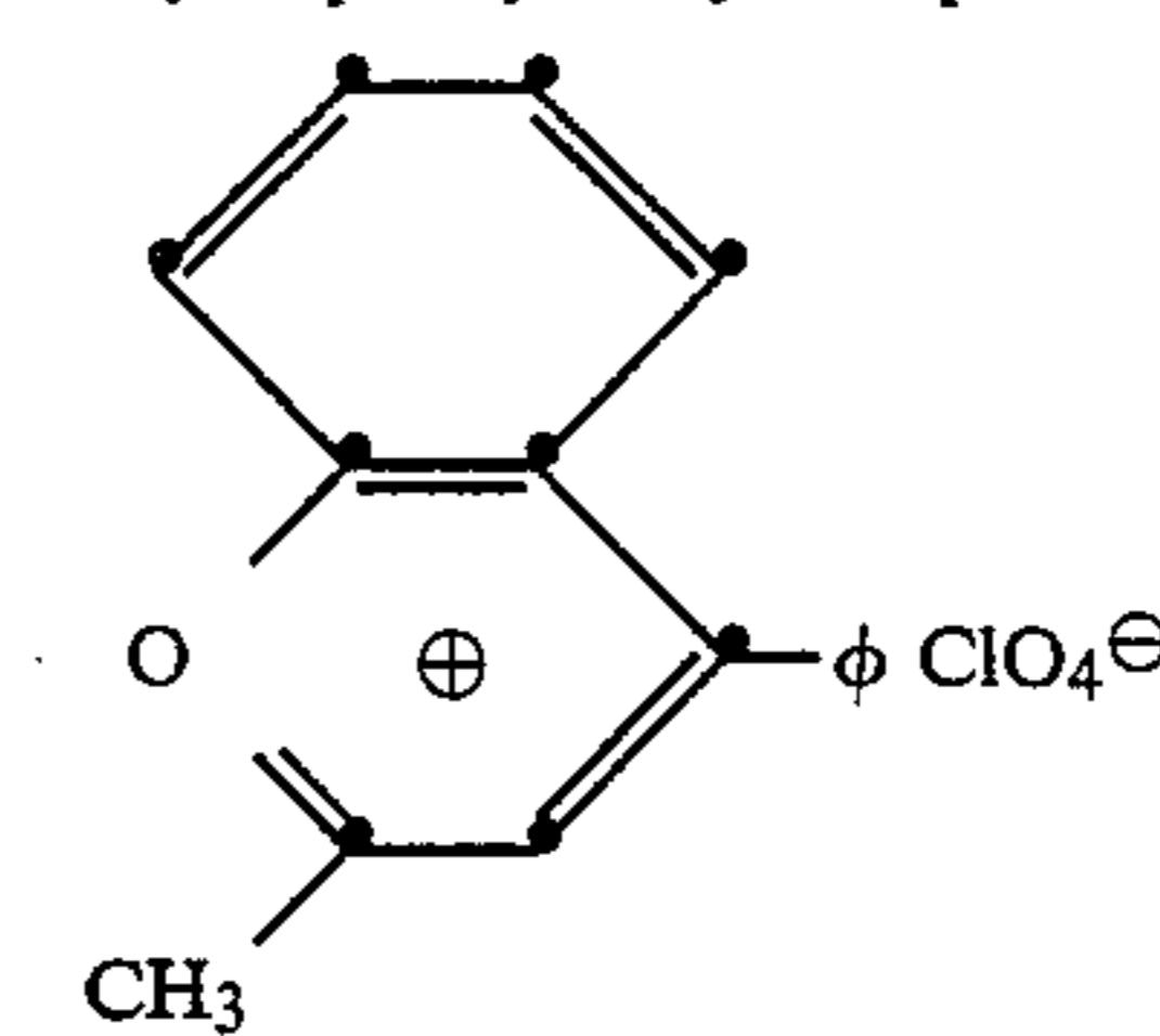
2-Methyl-4-phenylflavylium perchlorate M-5
