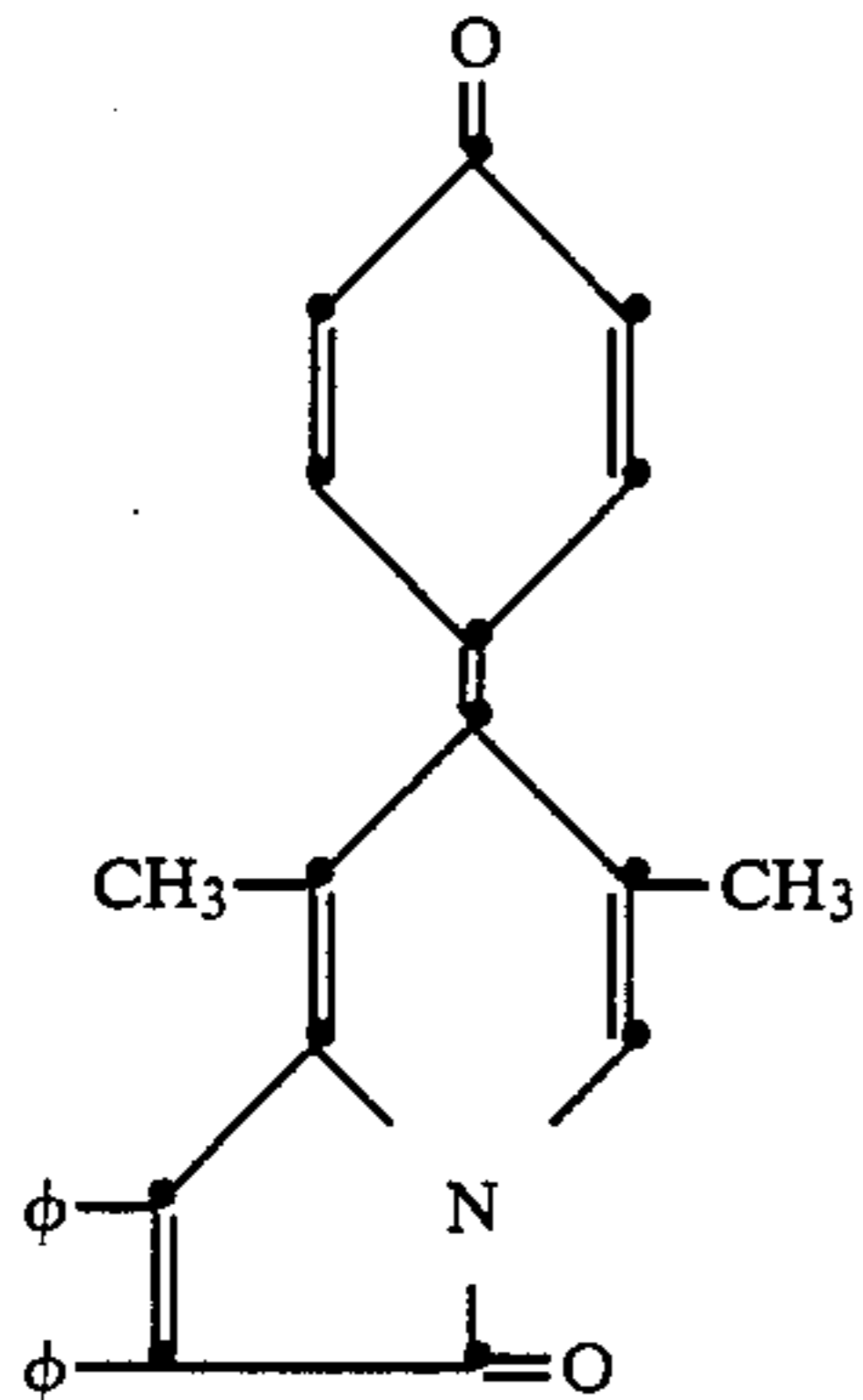
2,3-diphenyl-6-methylaminocarbonyl-7-(4-oxo-1-phenylidene)-1(7H)-indolizine
