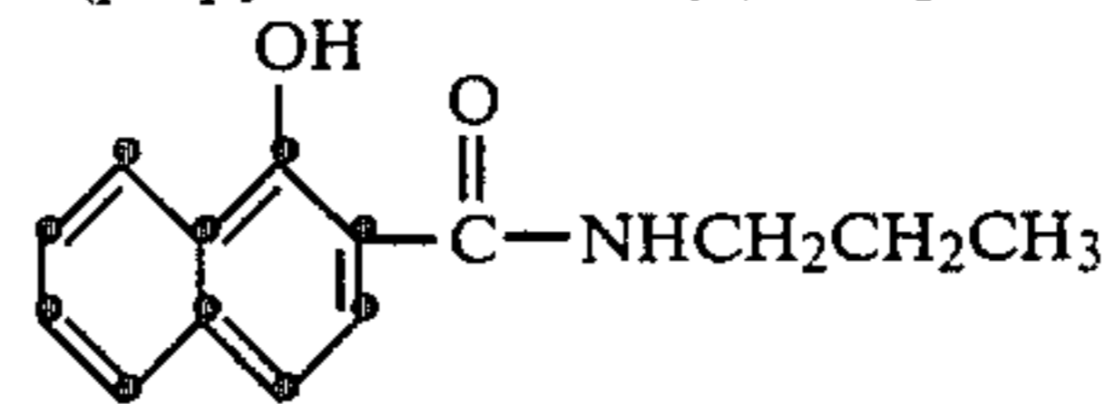
2-(propylaminocarbonyl)-1-naphthol
