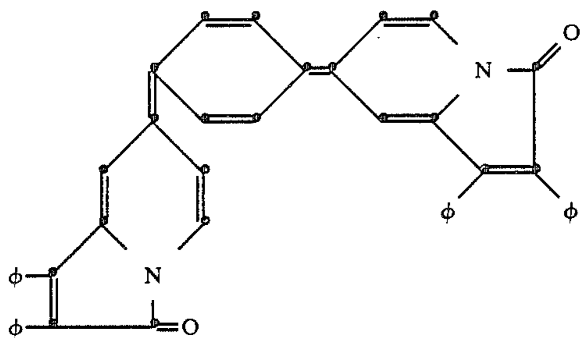
1,4-bis[7-(1,2-diphenyl-3(7H)-indolizinonylidene)]-2,3-benzo-2,5-cyclohexadiene
