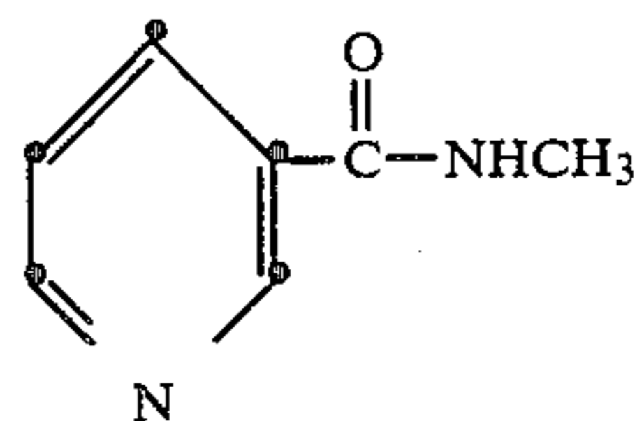
N-methylnicotinamide:
