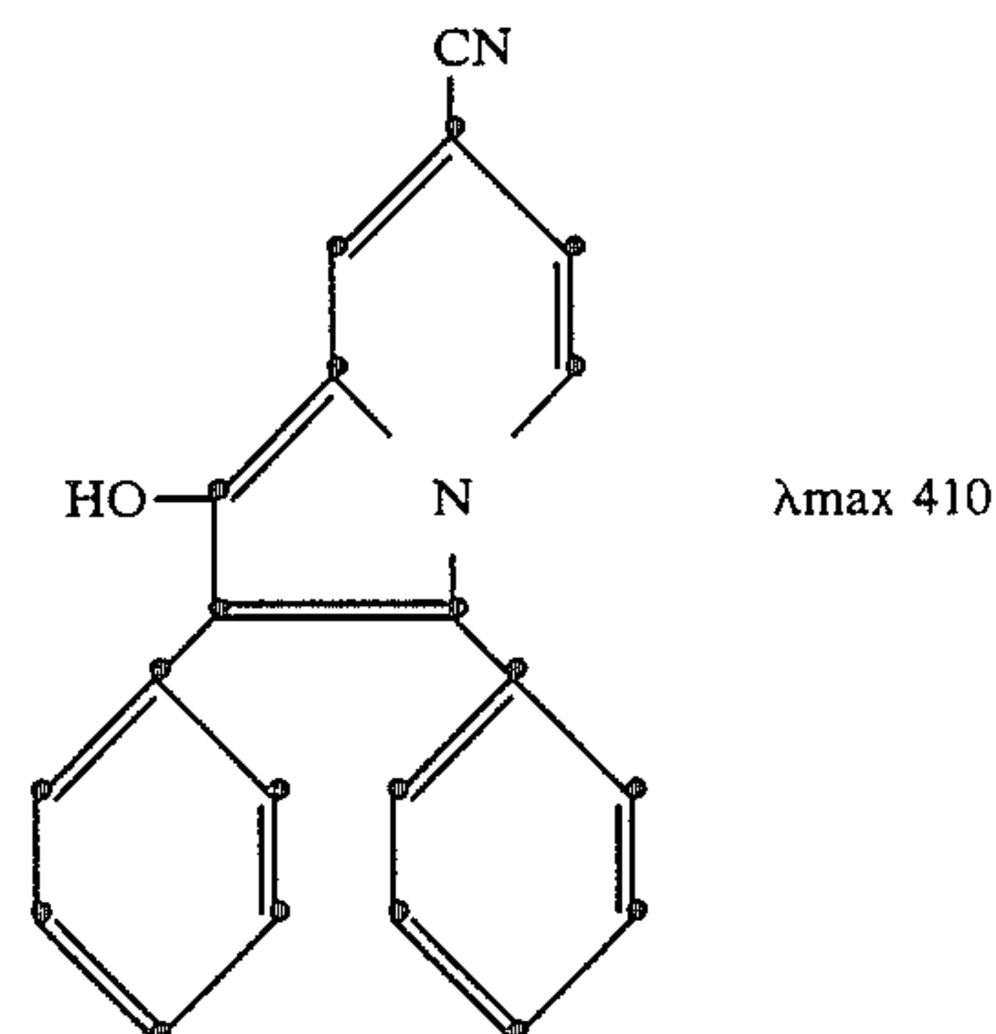
7-cyano-2,3-diphenyl-1-indolizinol
