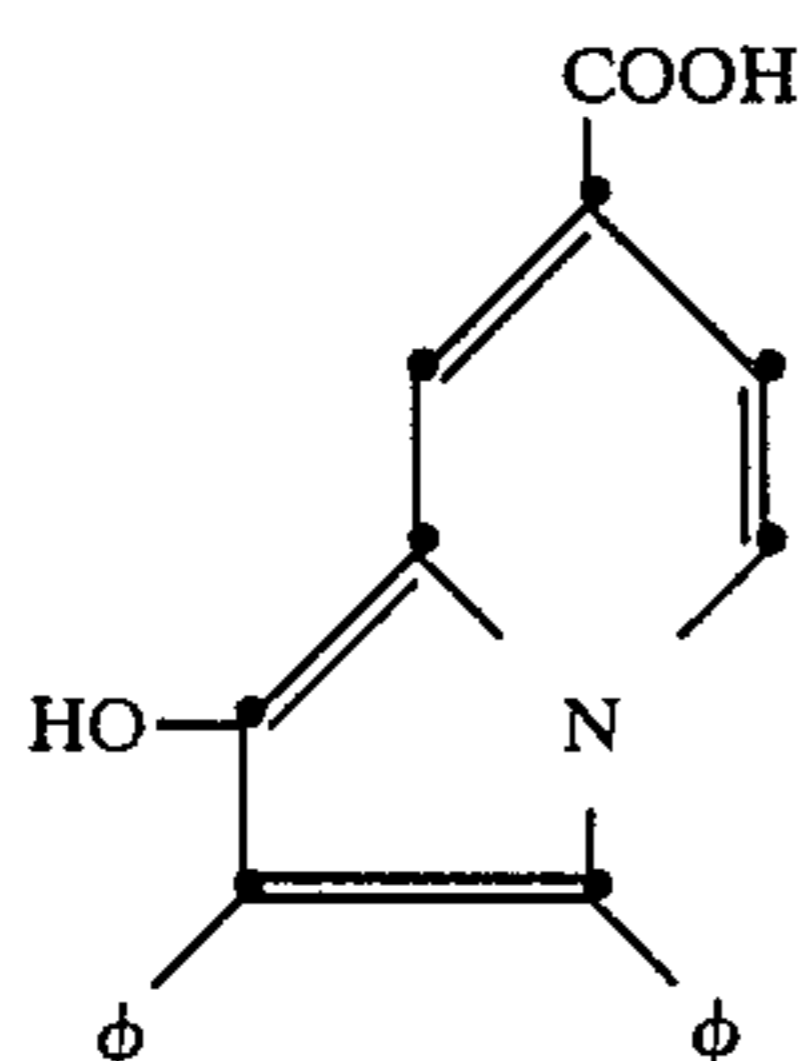
7-carboxy-2,3-diphenyl-1-indolizinol
