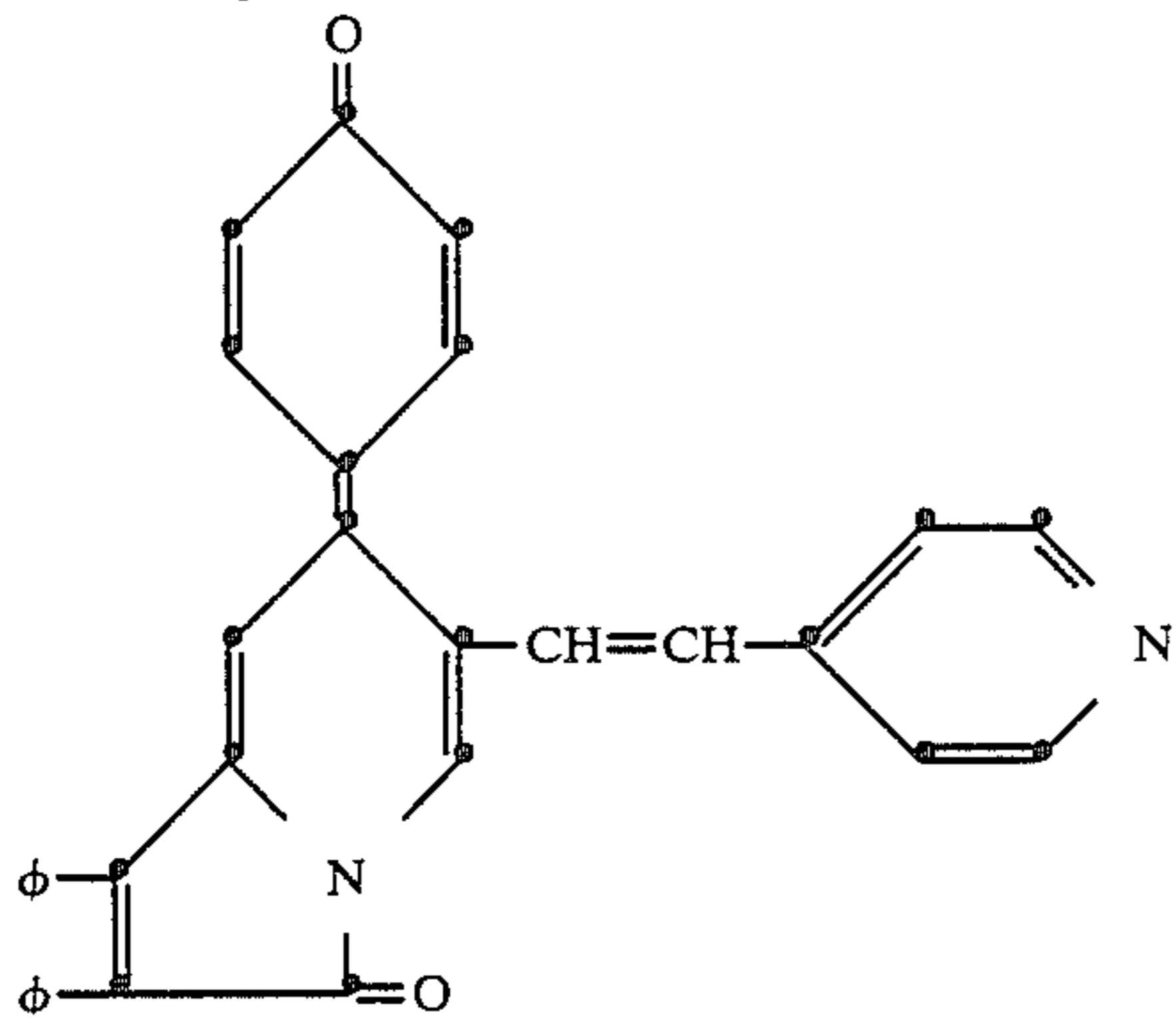
2,3-diphenyl-7-(2-hydroxy-4-oxo-3-pival-amido-1-phenylidene)-1(7H)-indolizinone
