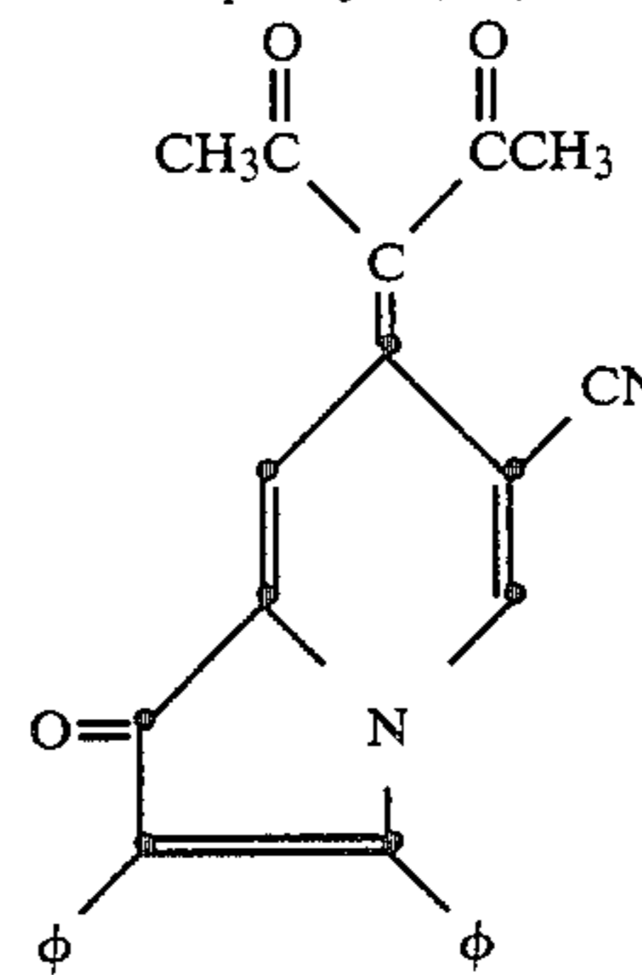
6-cyano-7-(diacetylmethylidene)-2,3-diphenyl-1(7H)-indolizinone
