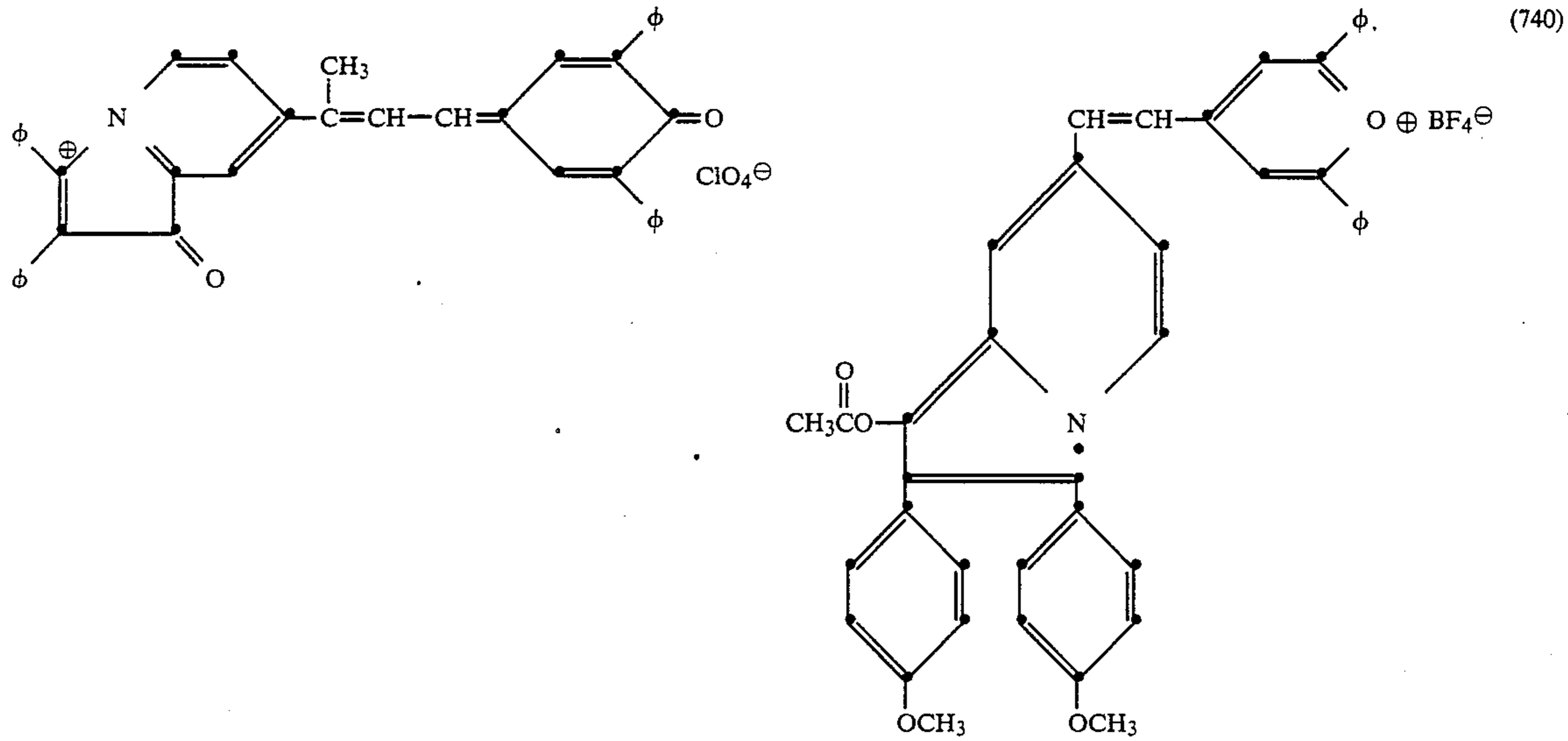
2,3-diphenyl-7-4-(2,6-diphenyl-4(4H)-pyran-5-ylidene)-2-(2-but-3-enyl)-1-indolizinium trifluoromethane sulfonate
