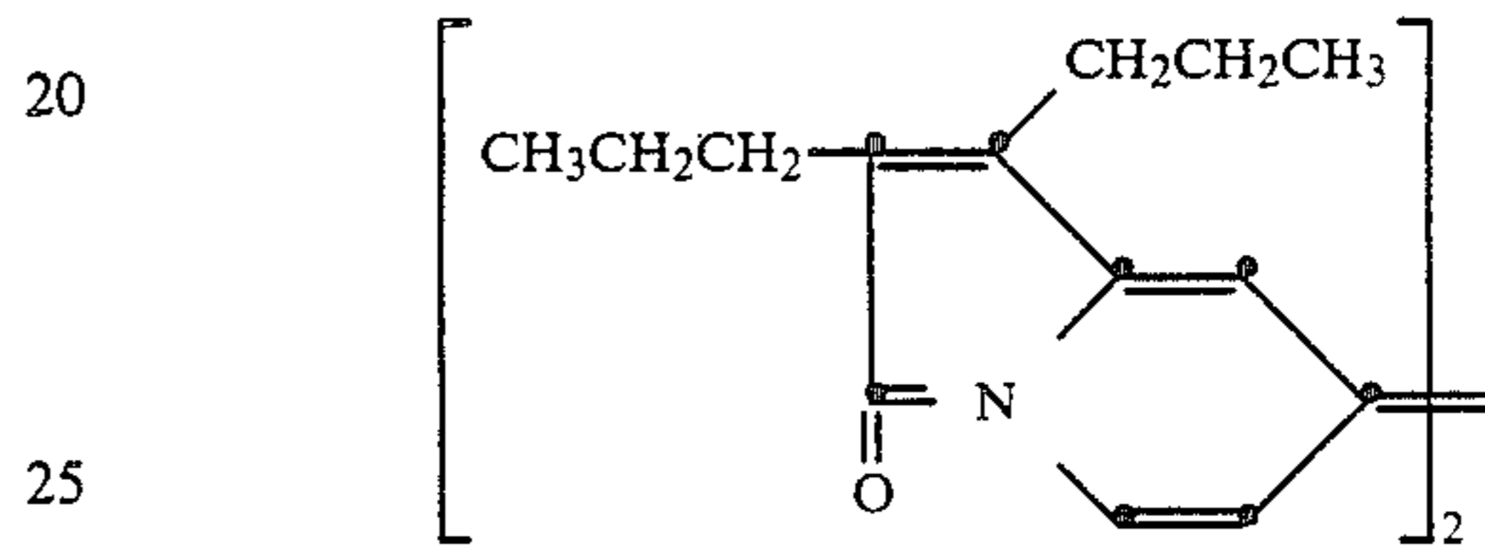
7,7'-bis[1,2-pentamethylene-3(7H)-indolizinonylidene]
