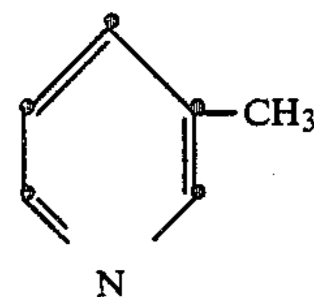
3-Picoline:
