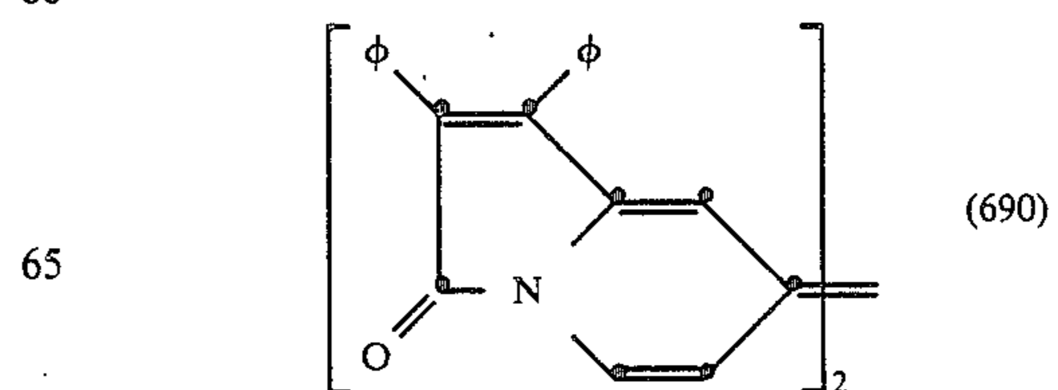
1,4-bis[7-(1,2-diphenyl-3(7H)-indolizinonylidene)]-2,3-benzo-2,5-cyclohexadiene
