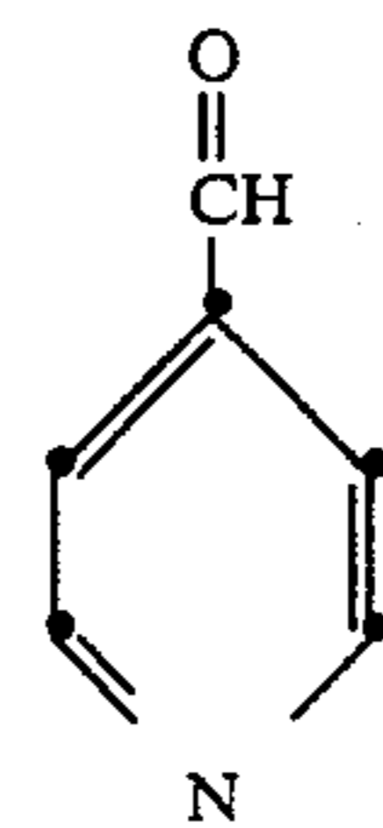
4-Formylpyridine (also known as 4-pyridine-carboxaldehyde):
