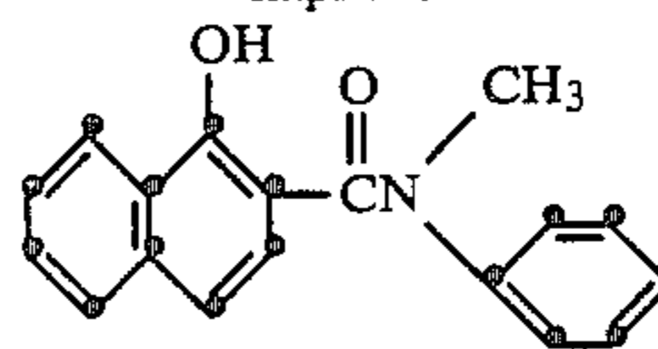
2-(N-methylanilino-carbonyl)-1-naphthol
