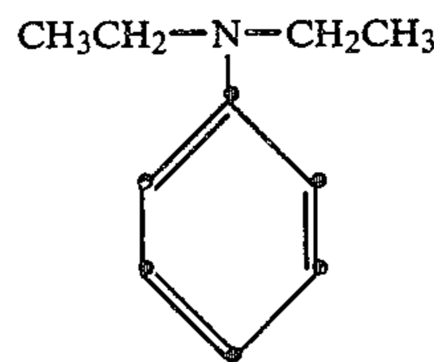
N,N—diethylaniline AN-3
