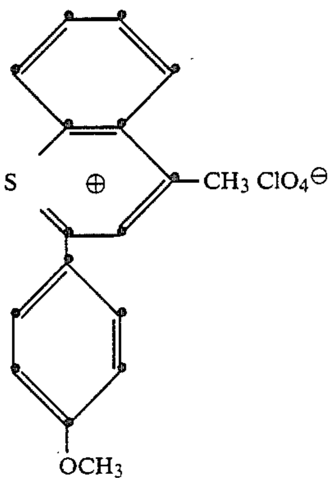
2-(4-methoxyphenyl)-4-methylthioflavylium perchlorate
