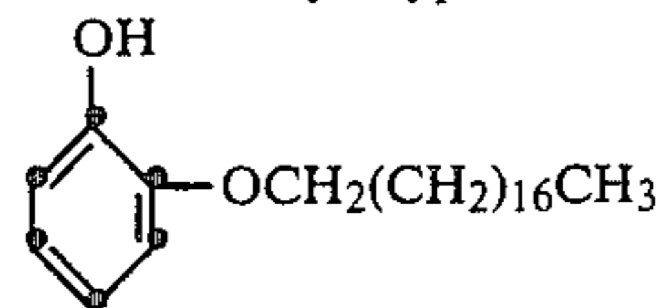
2-octadecyloxyphenol
