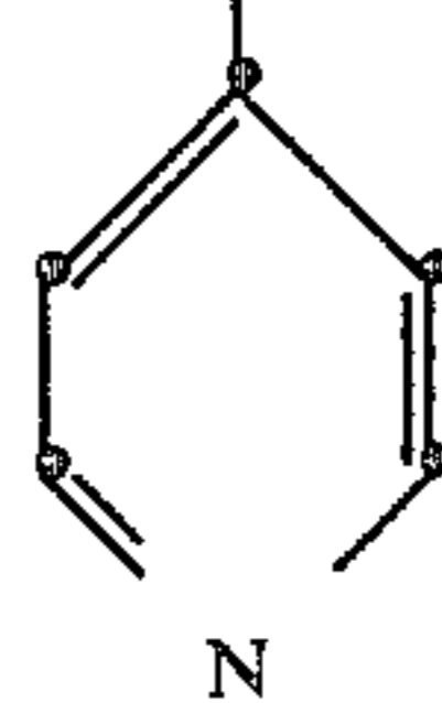
Ethyl 3-pyridylacetate:
