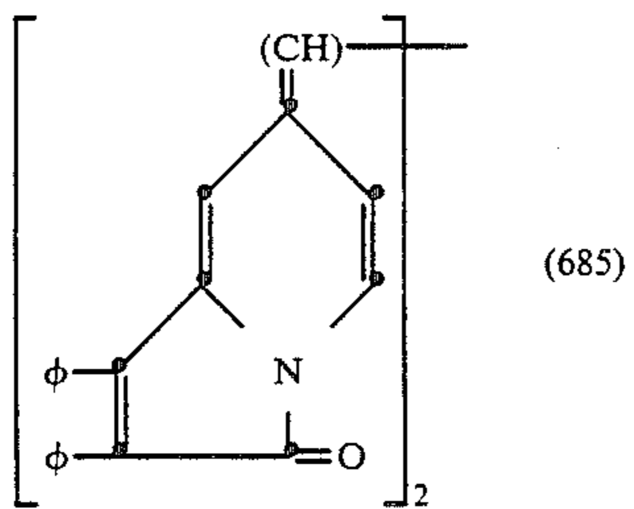
1,4-bis[7-(1,2-diphenyl-3(7H)-indolizinonylidene)]-2,5-cyclohexadiene
