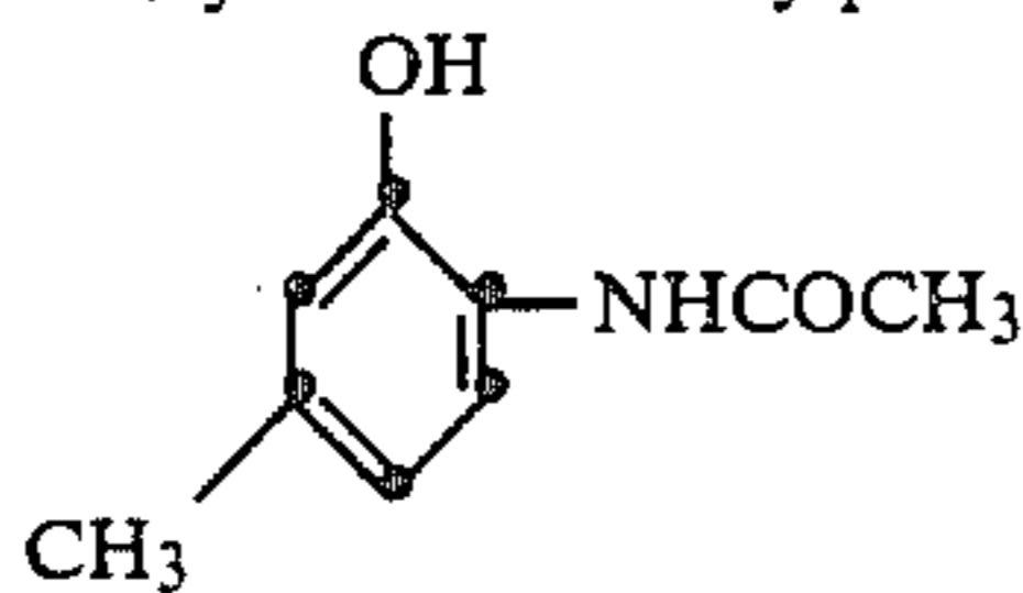
2-Acetylamino-5-methylphenol
