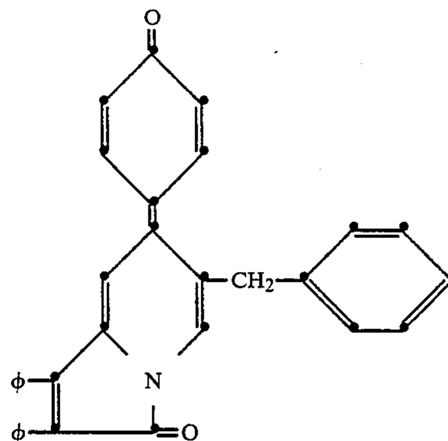
6-benzyl-1,2-diphenyl-7-(4-oxo-1-phenylidene)-3(7H)-indolizine
