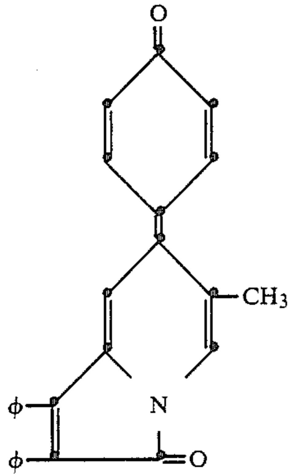
2,3-diphenyl-6-formyl-7-(4-oxo-1-phenylidene)-1(7H)-indolizinone
