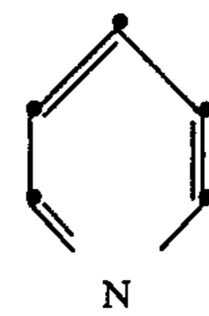
4-Picoline:
