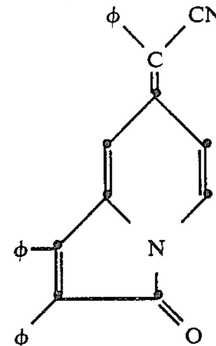
7-(1-cyano-1-phenylmethylidene)-1,2-diphenyl-3(7H)-indolizinone
