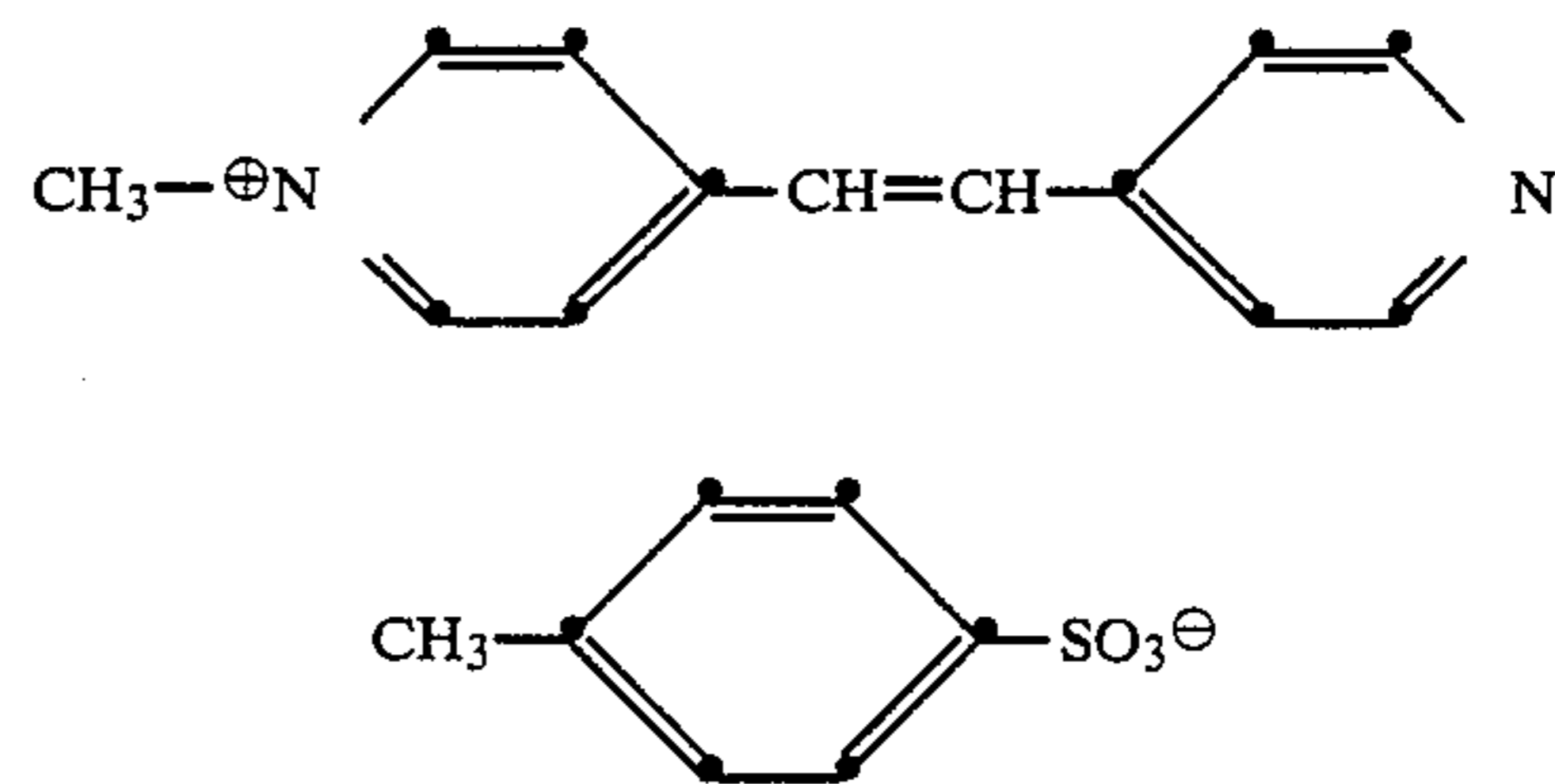
4-(4-Azasteryl)-1-methylpyridinium p-toluene sulfonate:
