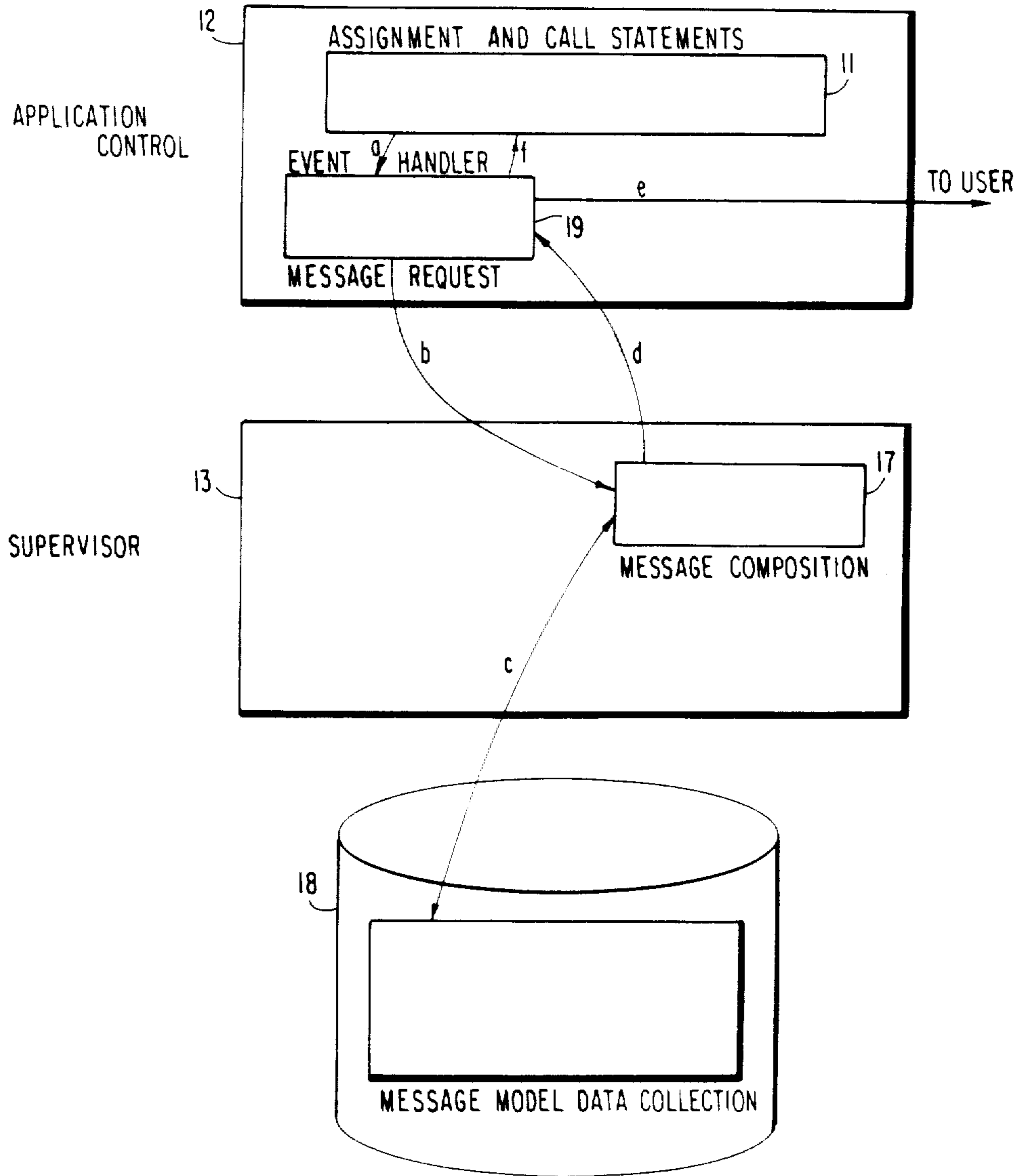
FIG. 5 APPLICATION CONTROL USE, CENTRAL COMPOSITION
