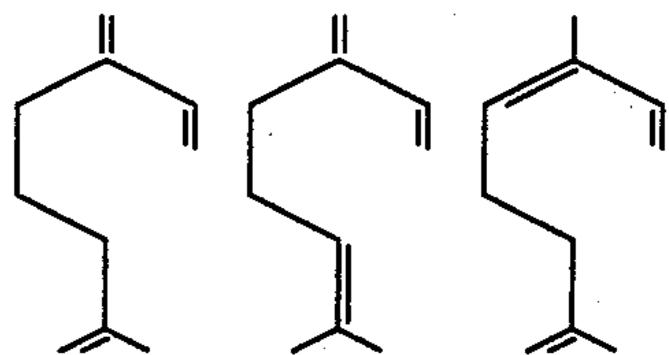
\alpha -Myrcene \beta -Myrcene cis- \alpha -ocimene
