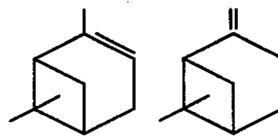
\alpha -Pinene \beta -Pinene
