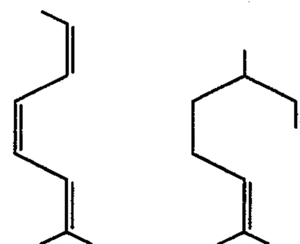
4-cis-6-cis- Alloocimene 1 Dihydromyrcene
