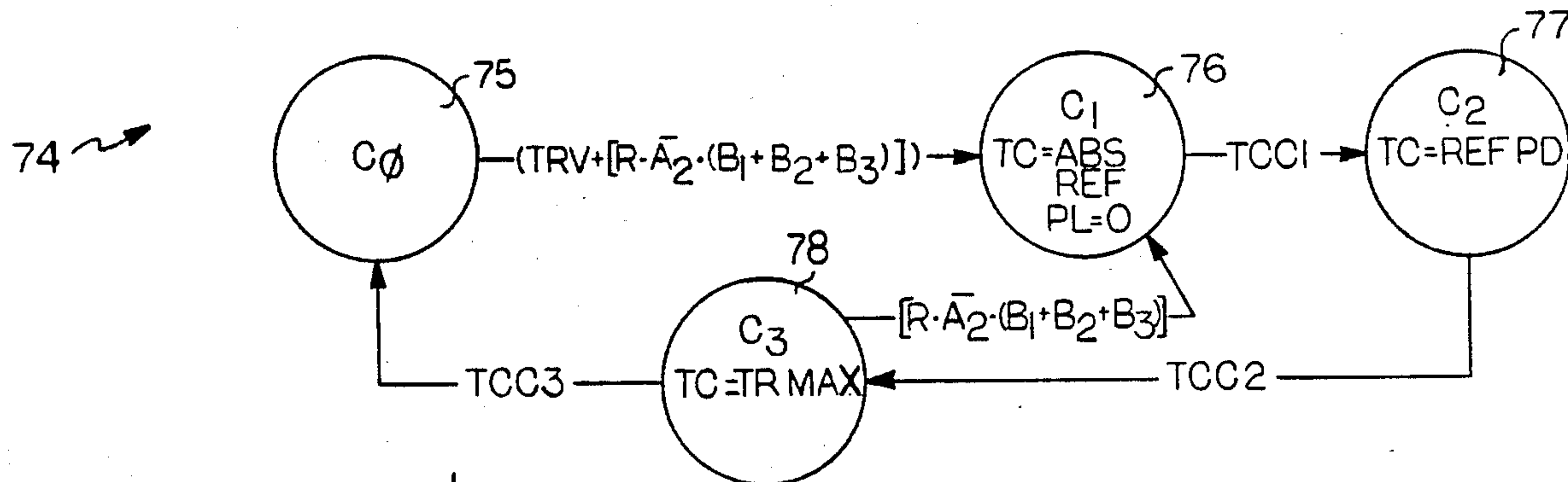
FIGURE 4 ('C' TIMER)
