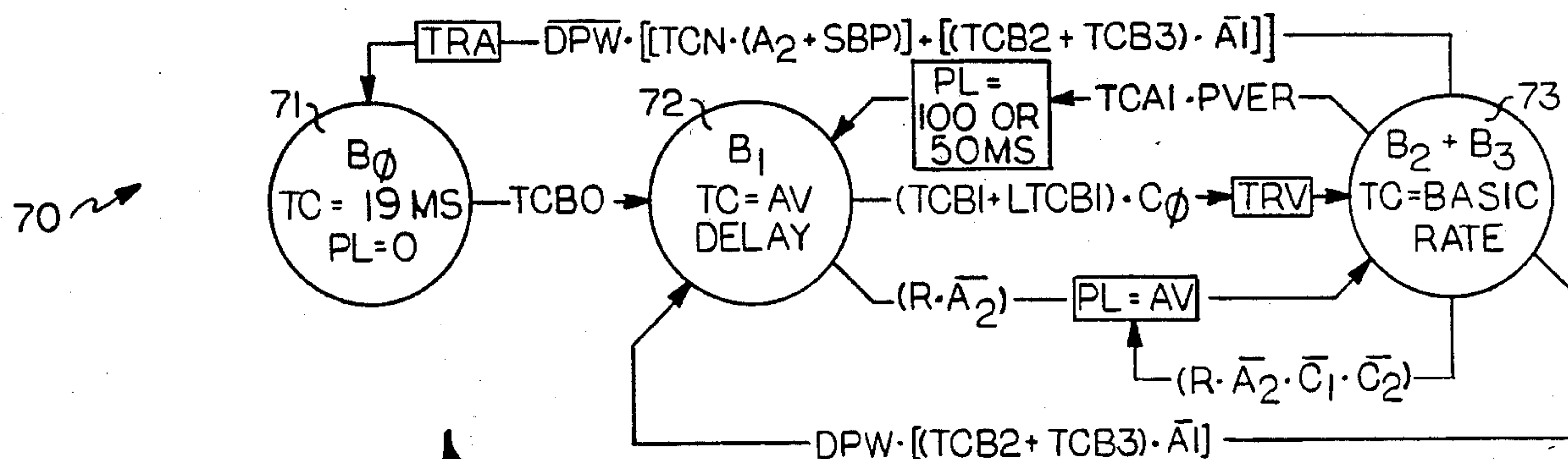
FIGURE 3 ('B' TIMER)
