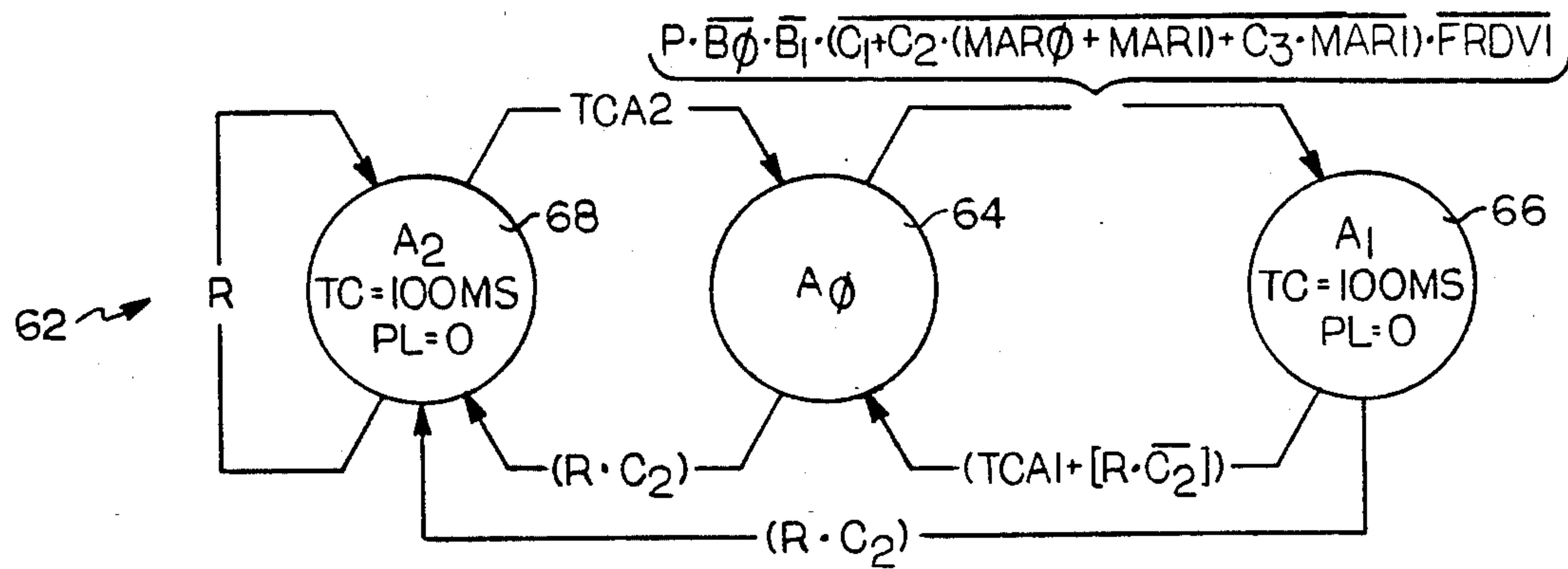
FIGURE 2 ('A' TIMER)
