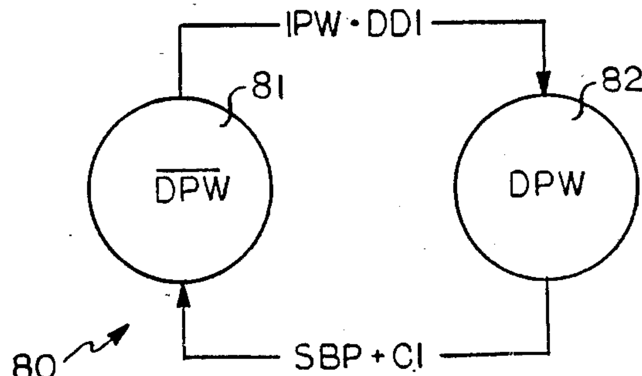
FIGURE 5B
