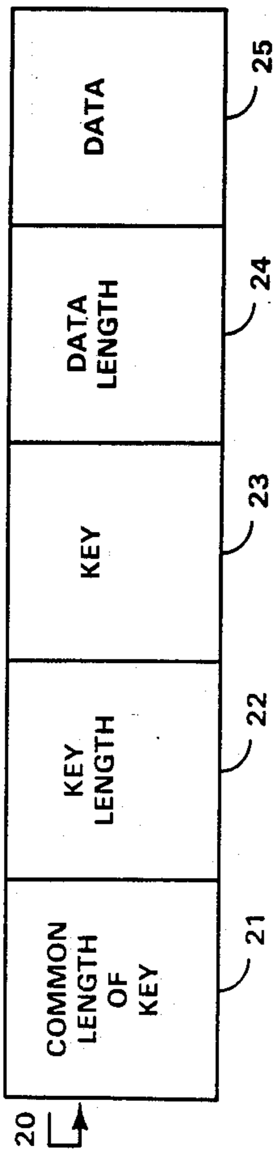
FIGURE 2. UNIVERSAL STORAGE ELEMENT
