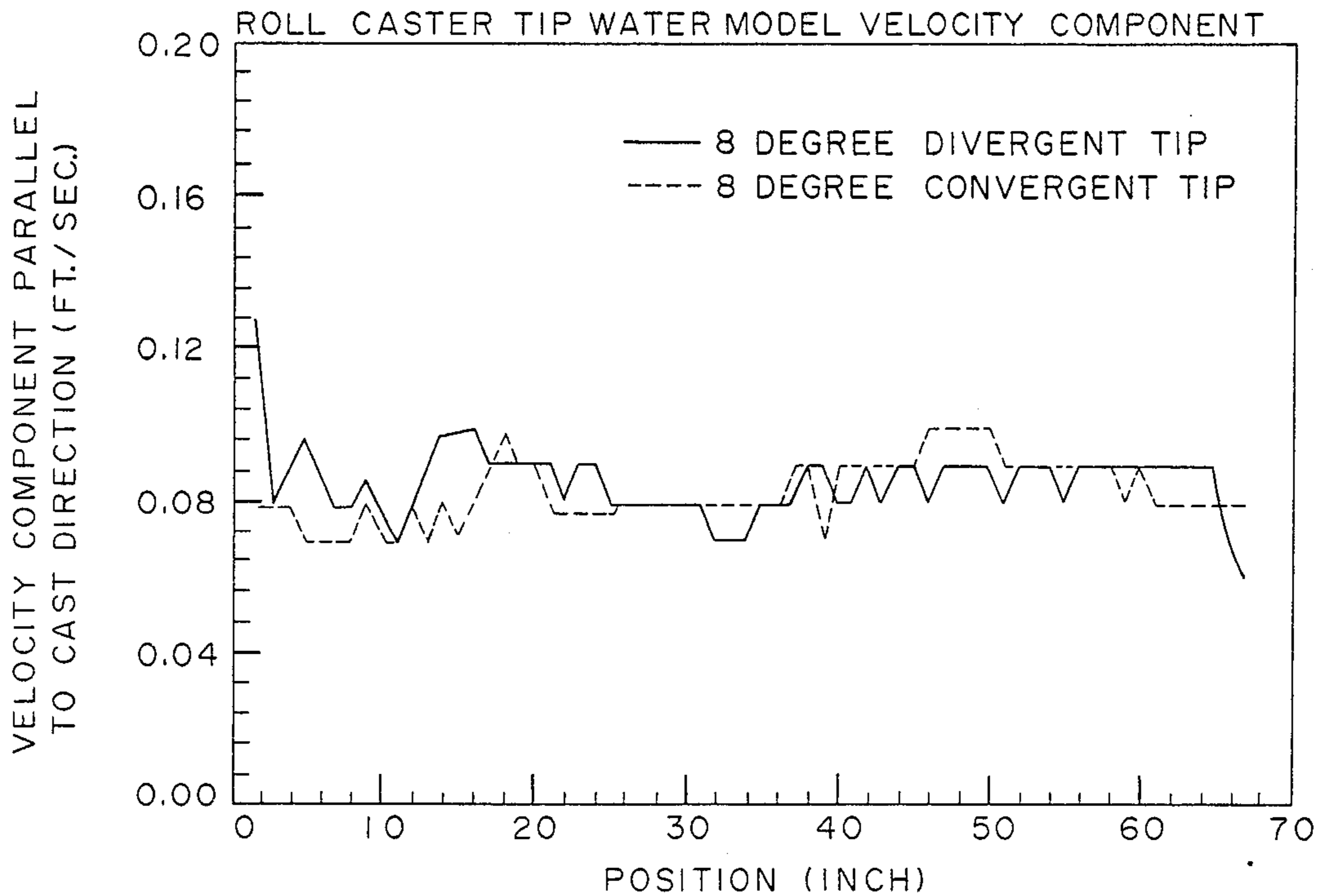
FIGURE 9 EQUIVALENT CASTING RATE 80 LBS./HR./INCH READINGS 7.5 INCHES FROM TIP DISCHARGE CASTING DIRECTION IS POSITION
