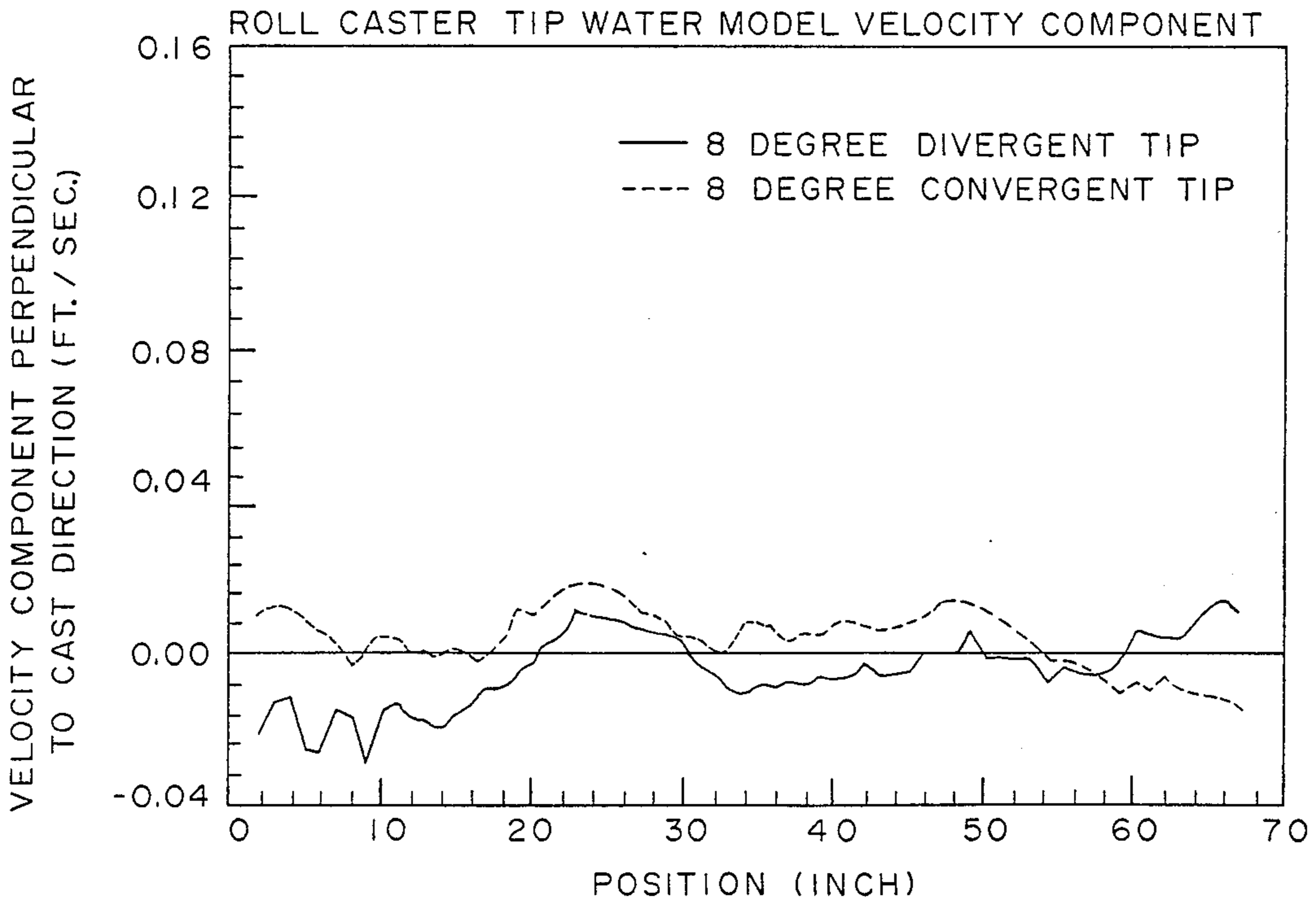
FIGURE 10 EQUIVALENT CASTING RATE 80 LBS./HR./INCH READINGS 7.5 INCHES FROM TIP DISCHARGE 90 DEG. COUNTER CLOCKWISE TO CASTING DIRECTION IS POSITIVE
