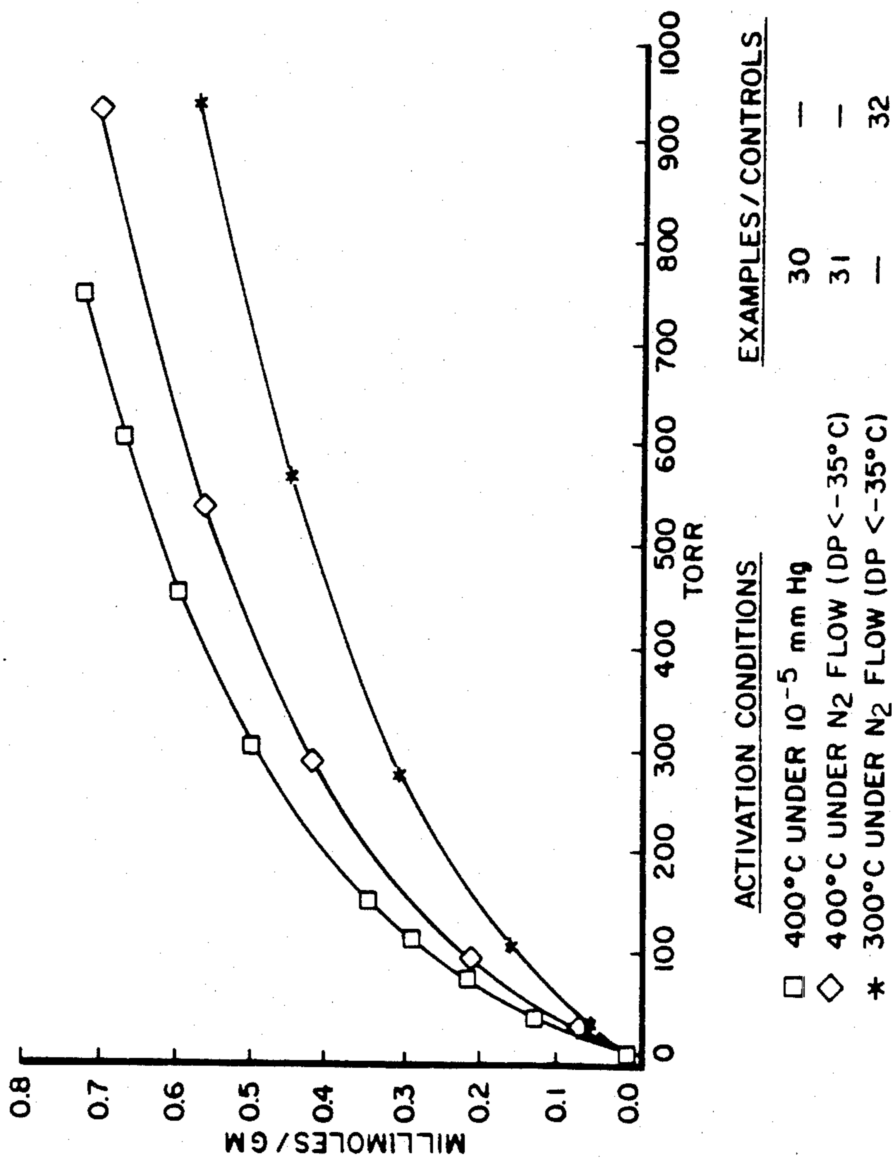
FIG. 3 NITROGEN ISOTHERMS FOR CaX
