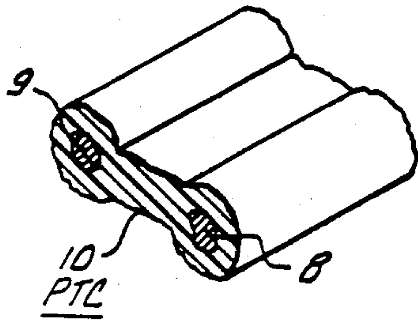
FIG. 5 (PRIOR ART)
