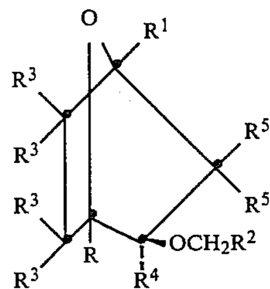
1S—exo-form
