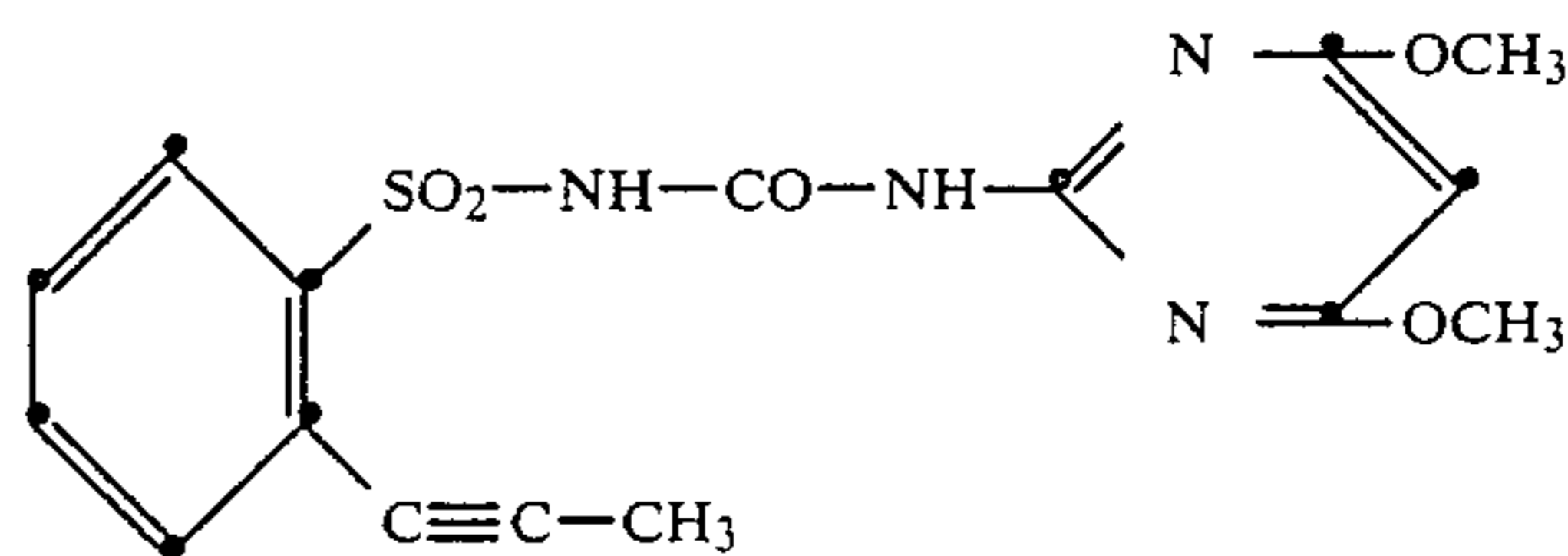
N-[2-(propyn-1-yl)phenylsulfonyl]-N'-(4,6-dimethoxypyrimidin-2-yl)urea (compound 5.1)
