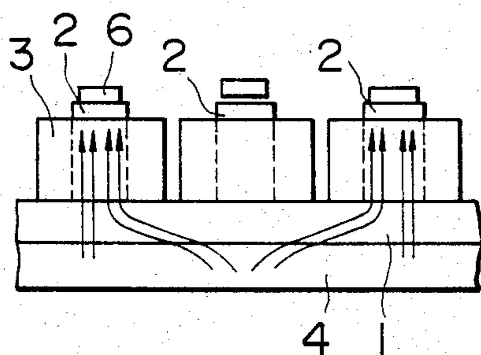
FIG. 2 (a) PRIOR INVENTION
