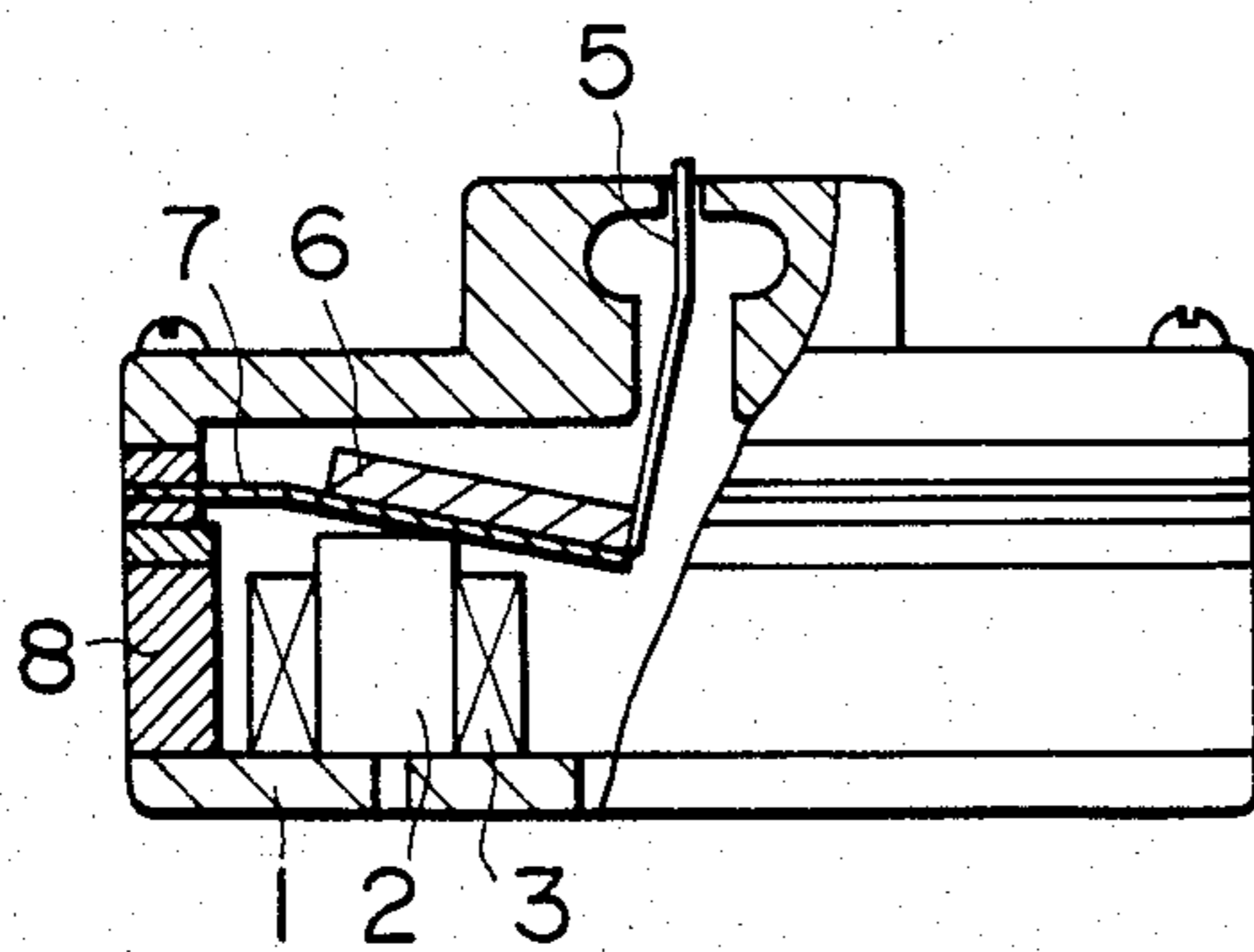
FIG. 4 PRIOR INVENTION
