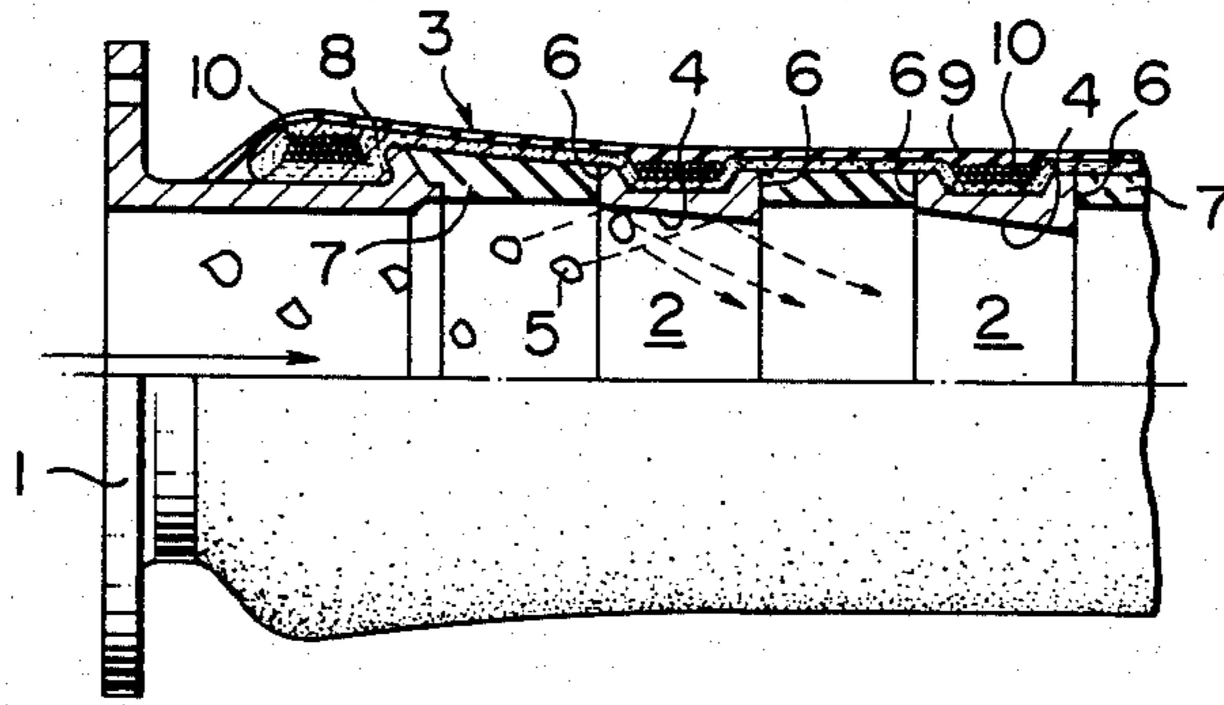
FIG. 1 PRIOR ART
