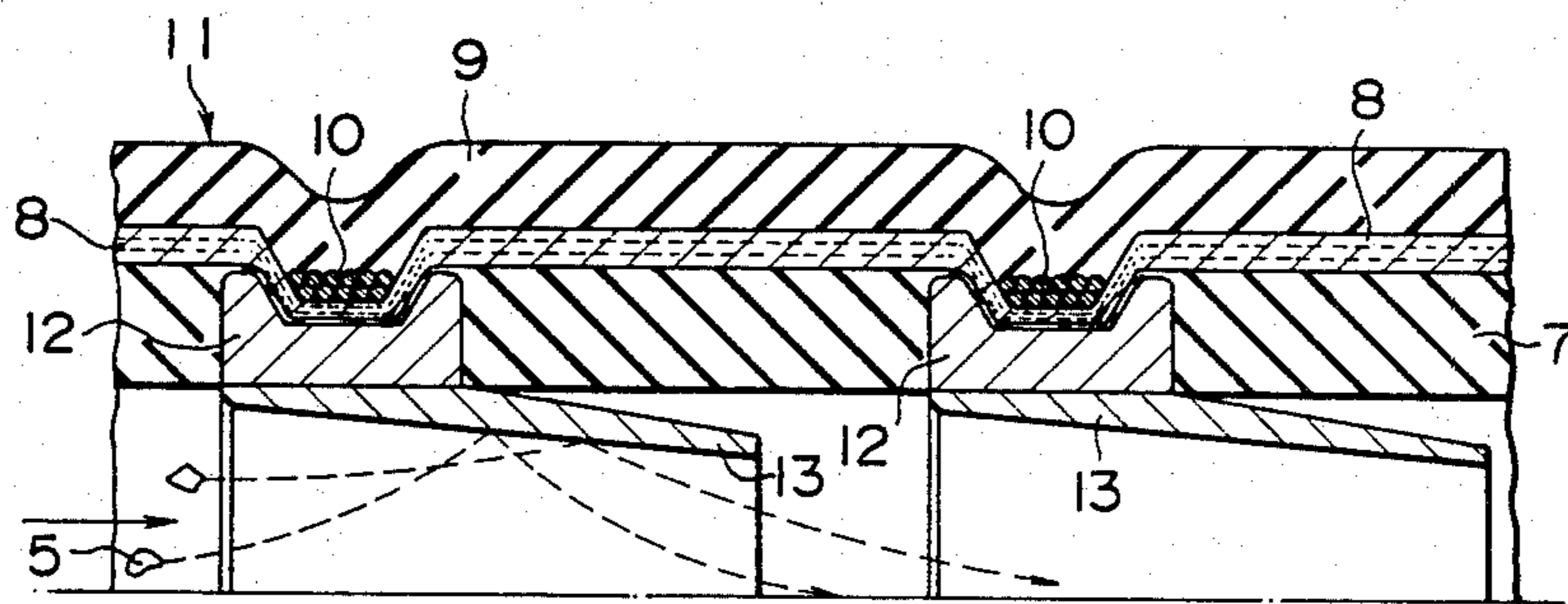
FIG. 2 PRIOR ART
