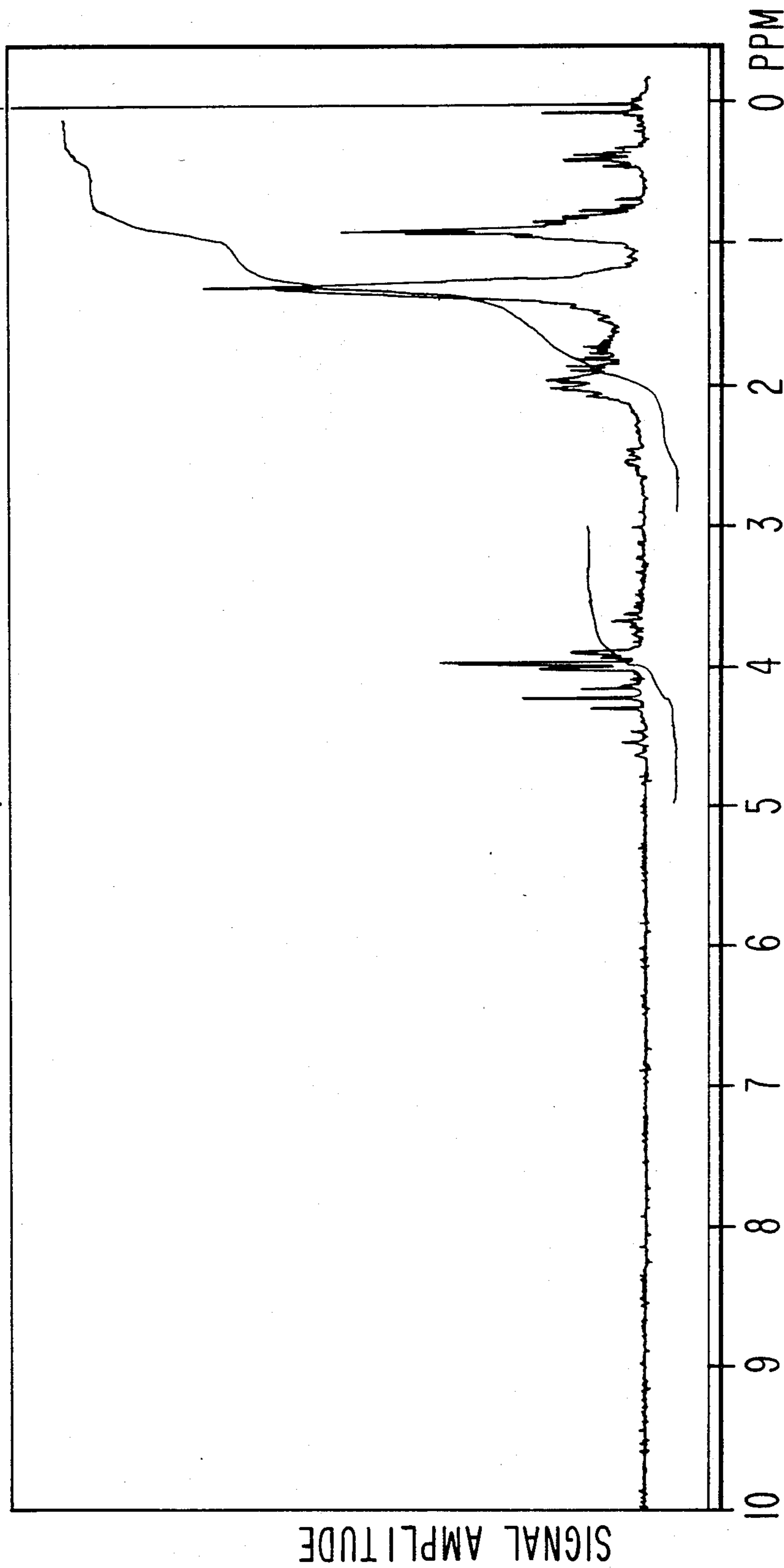
NMR SPECTRUM FOR PEAK 12 OF FIG.1A, EXAMPLE I.
