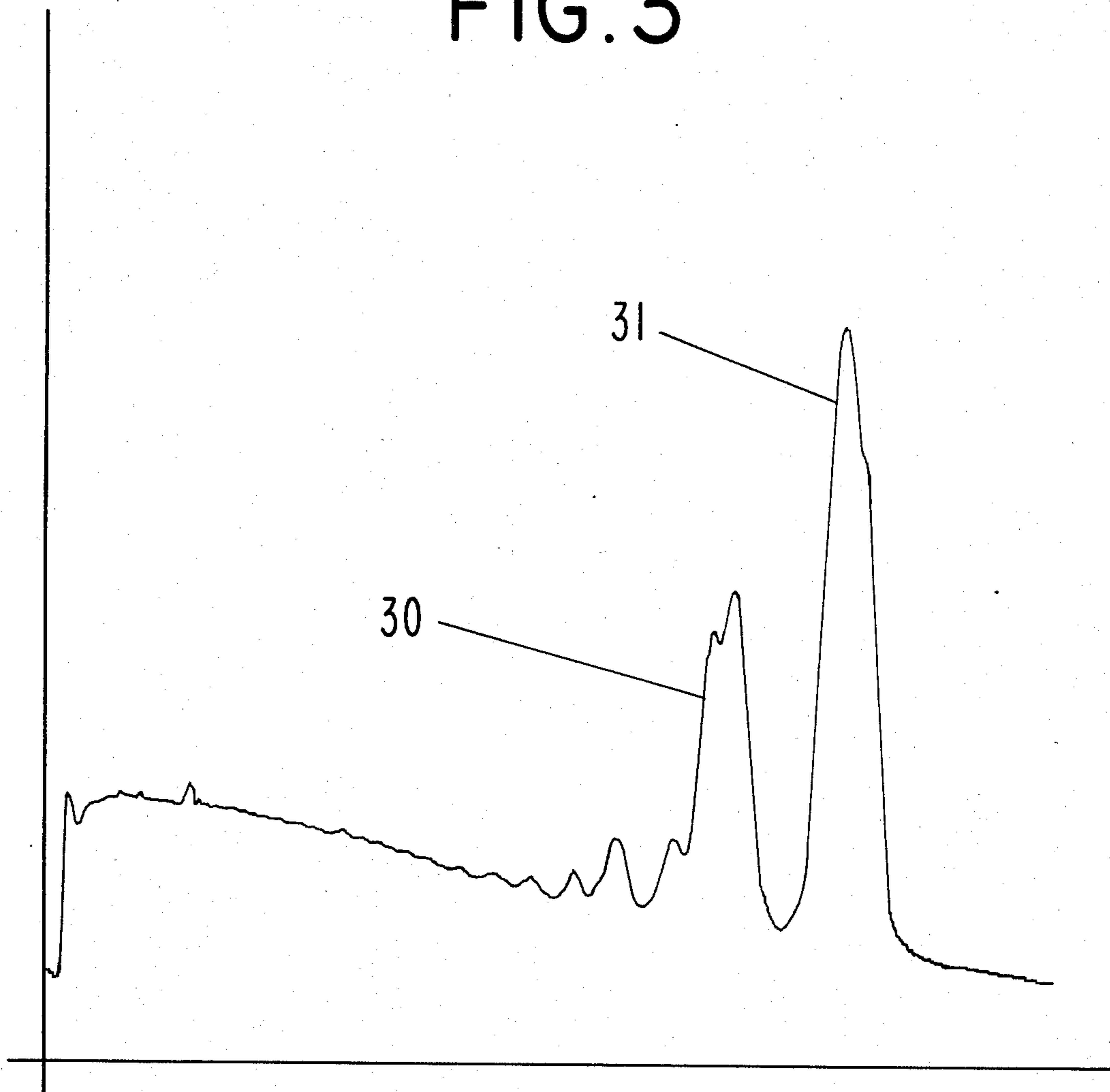
GLC PROFILE FOR EXAMPLE II . FIRST DISTILLATION PRODUCT .
