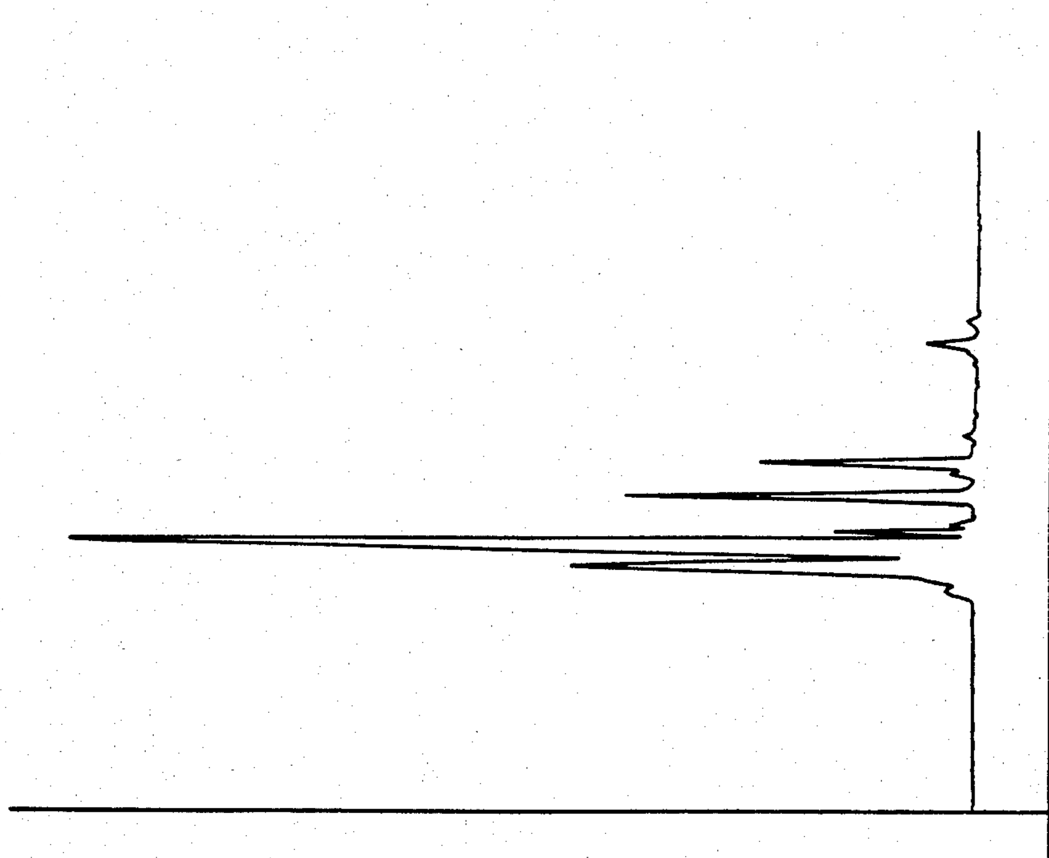
GLC PROFILE FOR FRACTION 4 OF EXAMPLE IV . 1 ST DISTILLATION
