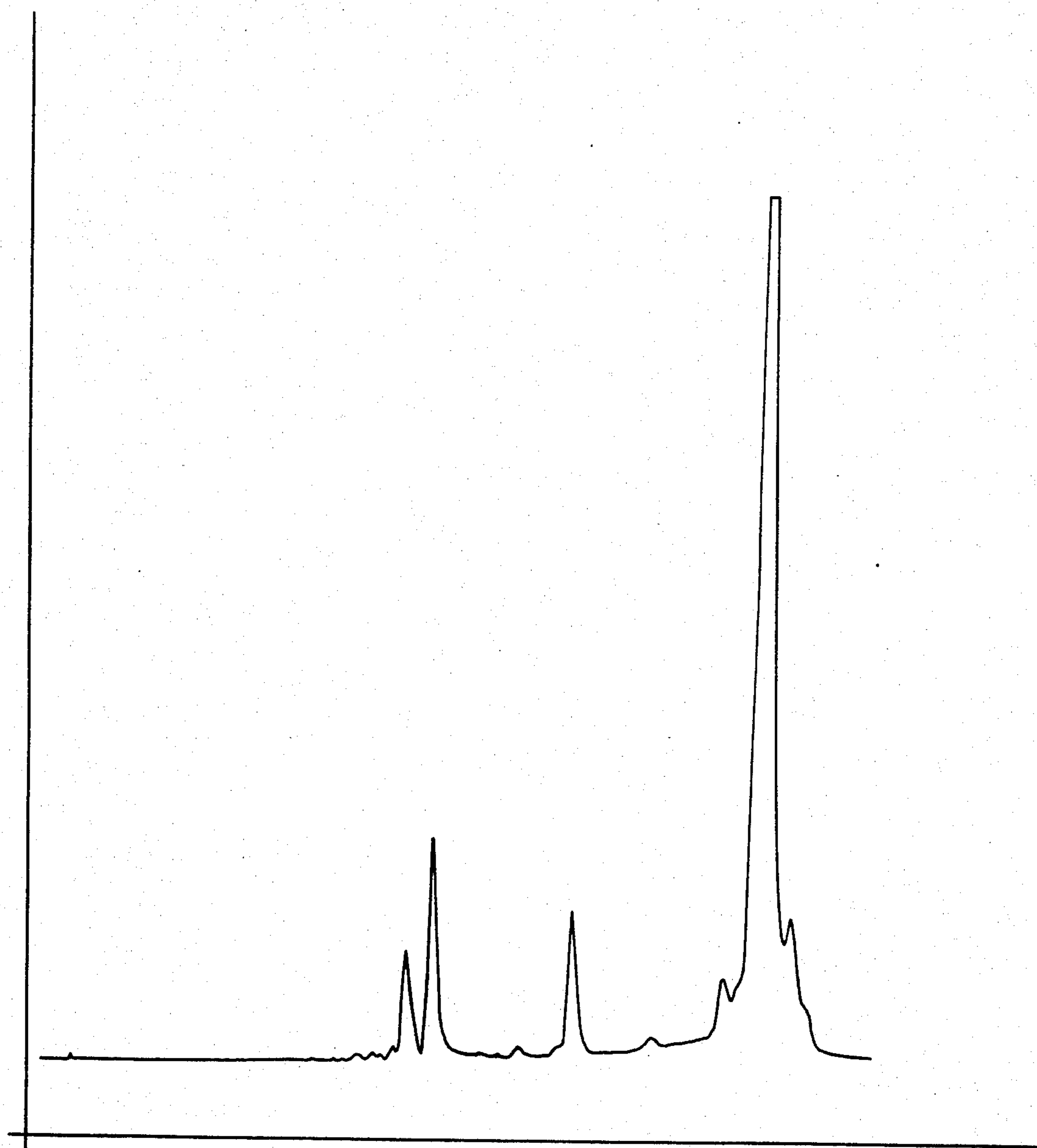
GLC PROFILE FOR FRACTION 3 OF EXAMPLE III.
