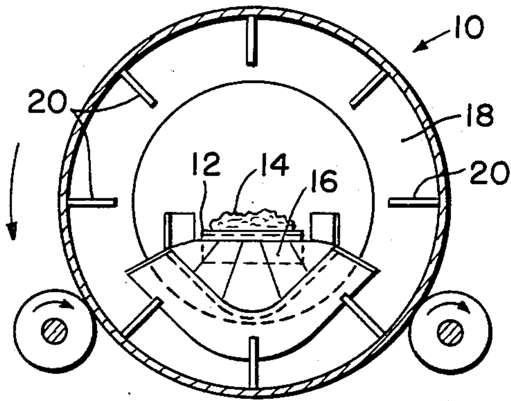
FIG-2 CHARGING END
