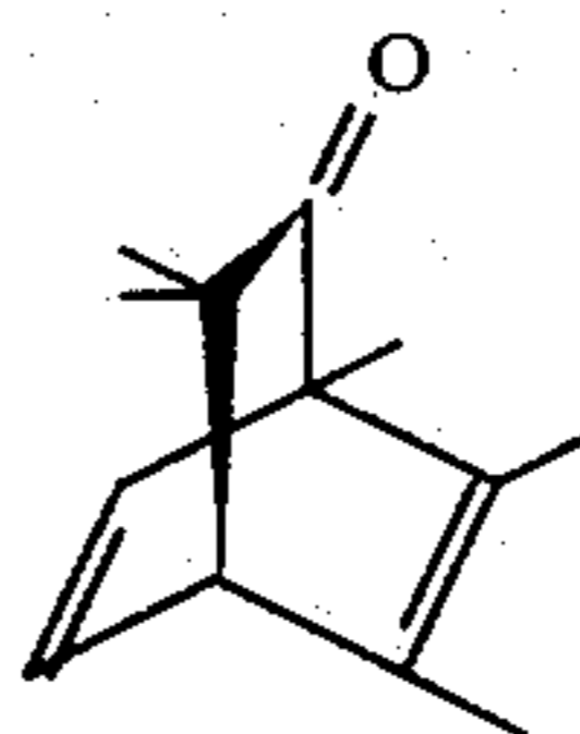
FIG. 5 is the GLC profile for the reaction product of Example II. The peak indicated on FIG. 5 by reference numeral "501" is the peak for the compound having the structure:
