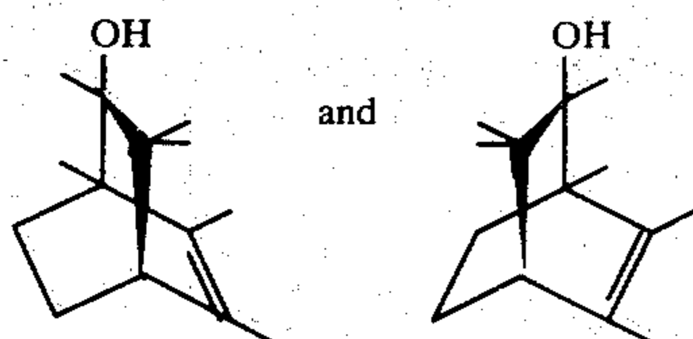
FIG. 25 is the GLC profile for the reaction product of Example XX containing the isomers defined according to the structures:
