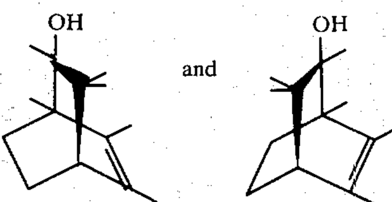
The peaks indicated by reference numerals "901" and "902" are the peaks for the isomers defined according to the structures:
