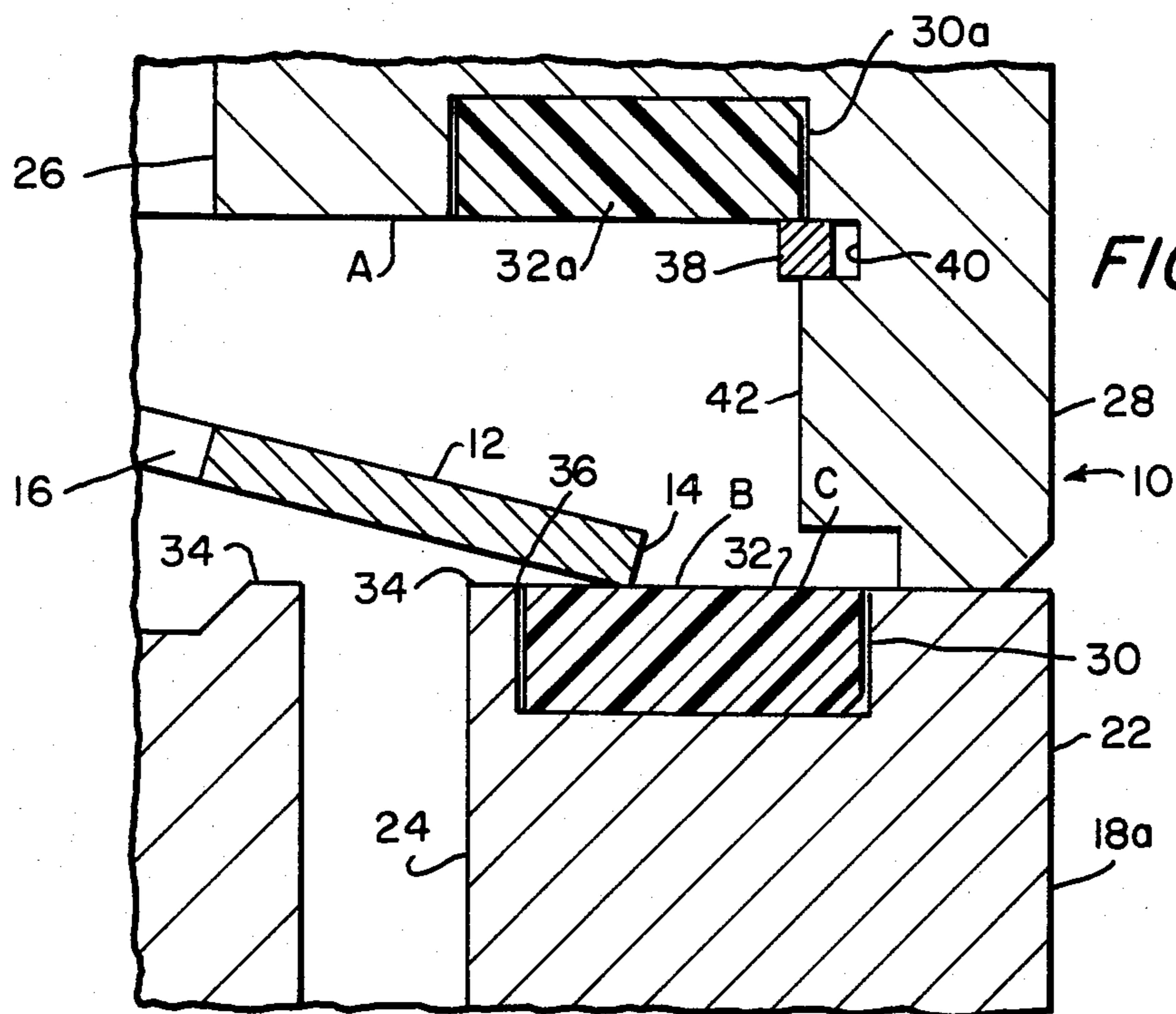
PRIOR ART FIG. 2B
