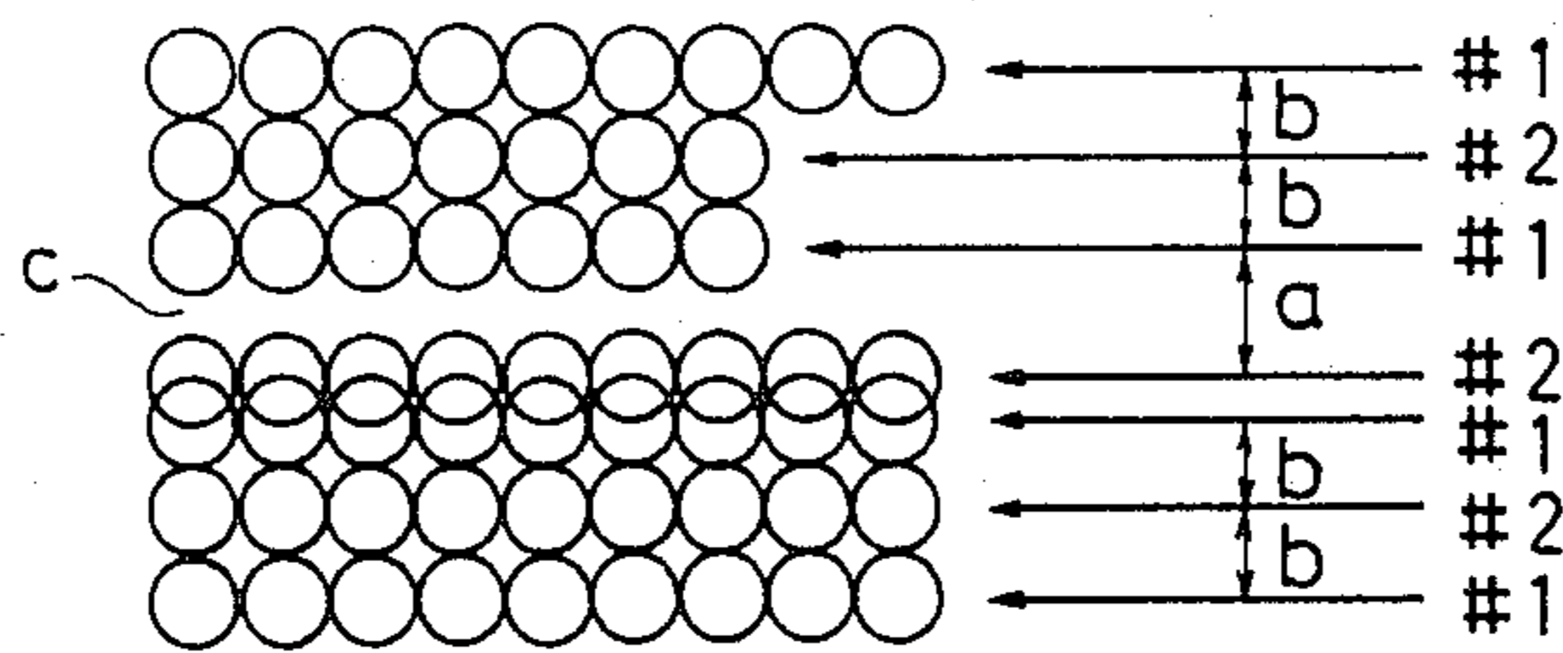
FIG. 2 PRIOR ART
