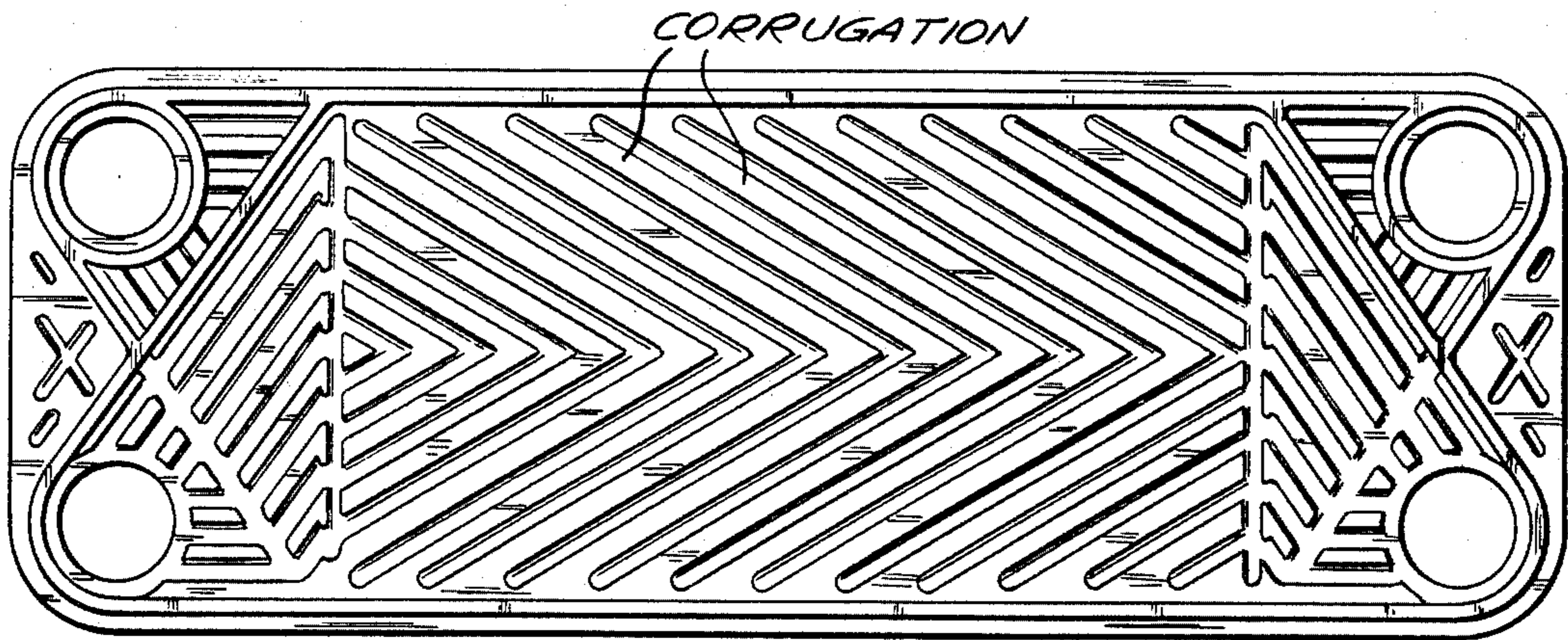
Fig. 1 (PRIOR ART)
