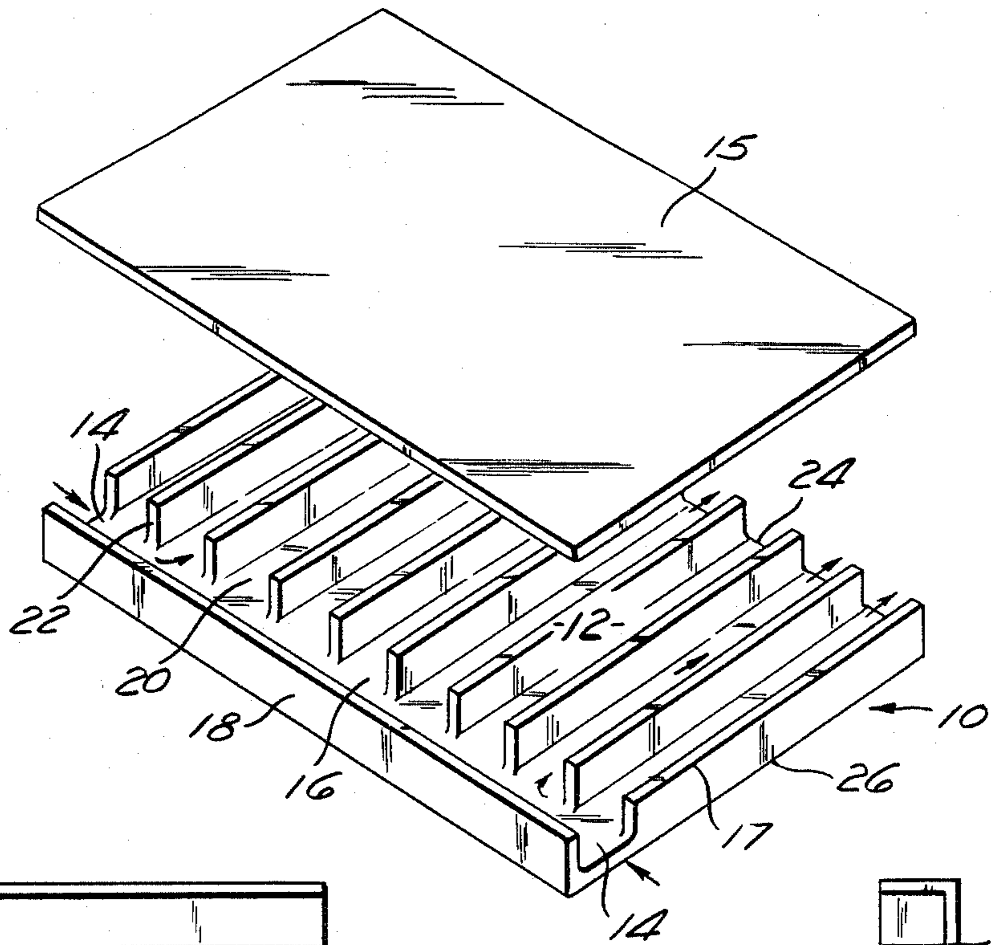
Fig. 1 (PRIOR ART)
