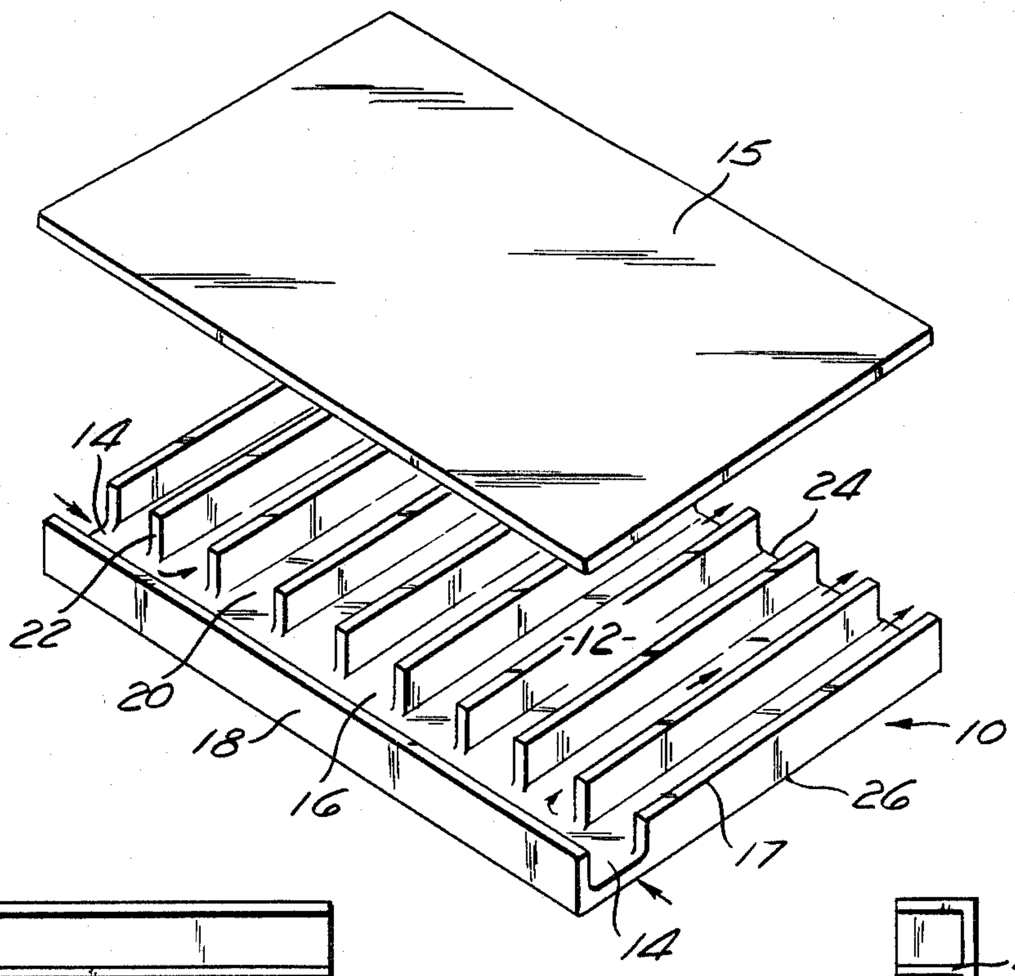
Fig. 1 (PRIOR ART)
