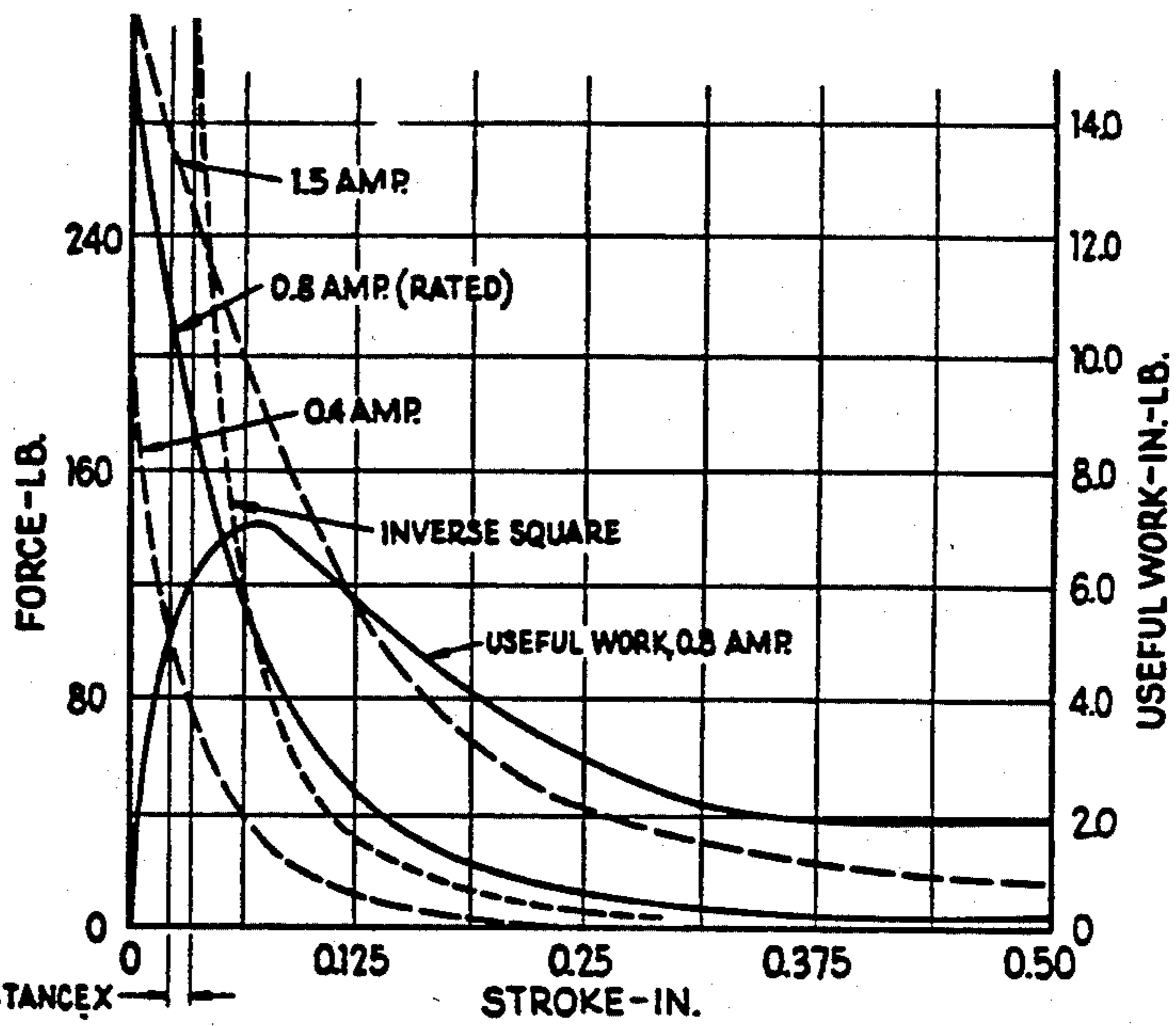
FLAT-FACED PLUNGER MAGNET AND ITS FORCE-STROKE CURVES
