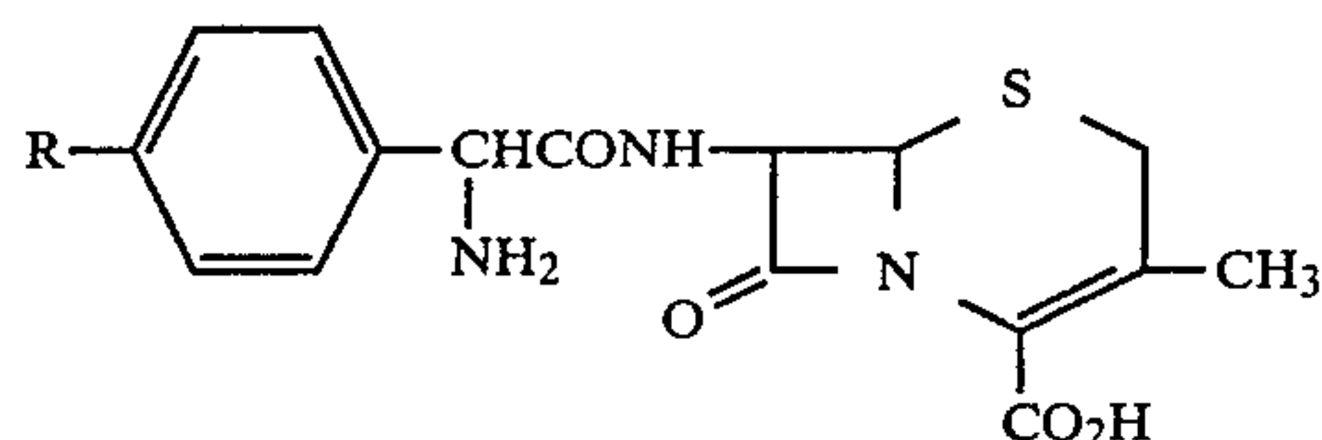
R=H cephalexin IX R=OH cefadroxil X
