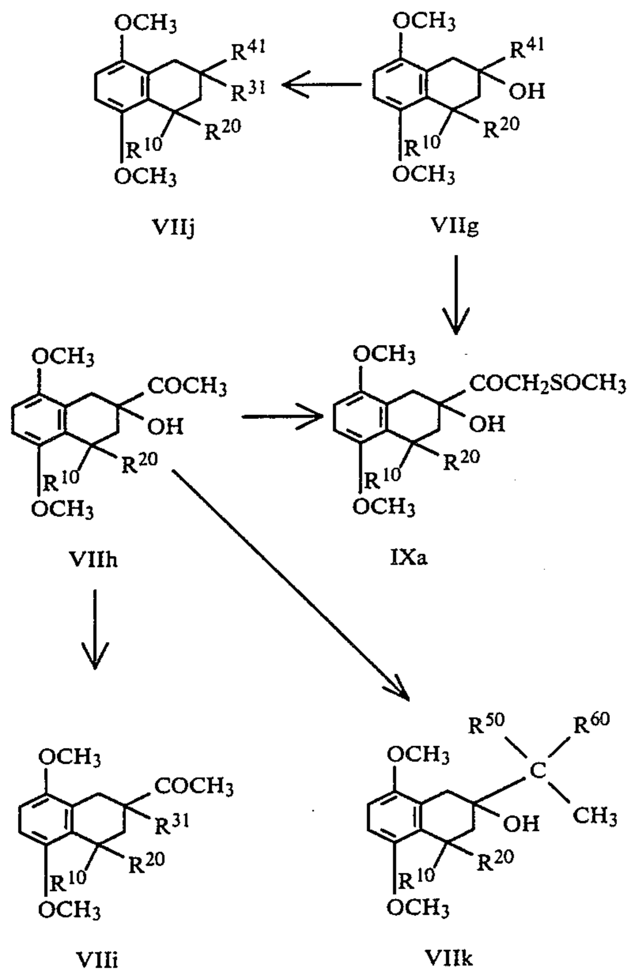
-continued Formula Scheme II
