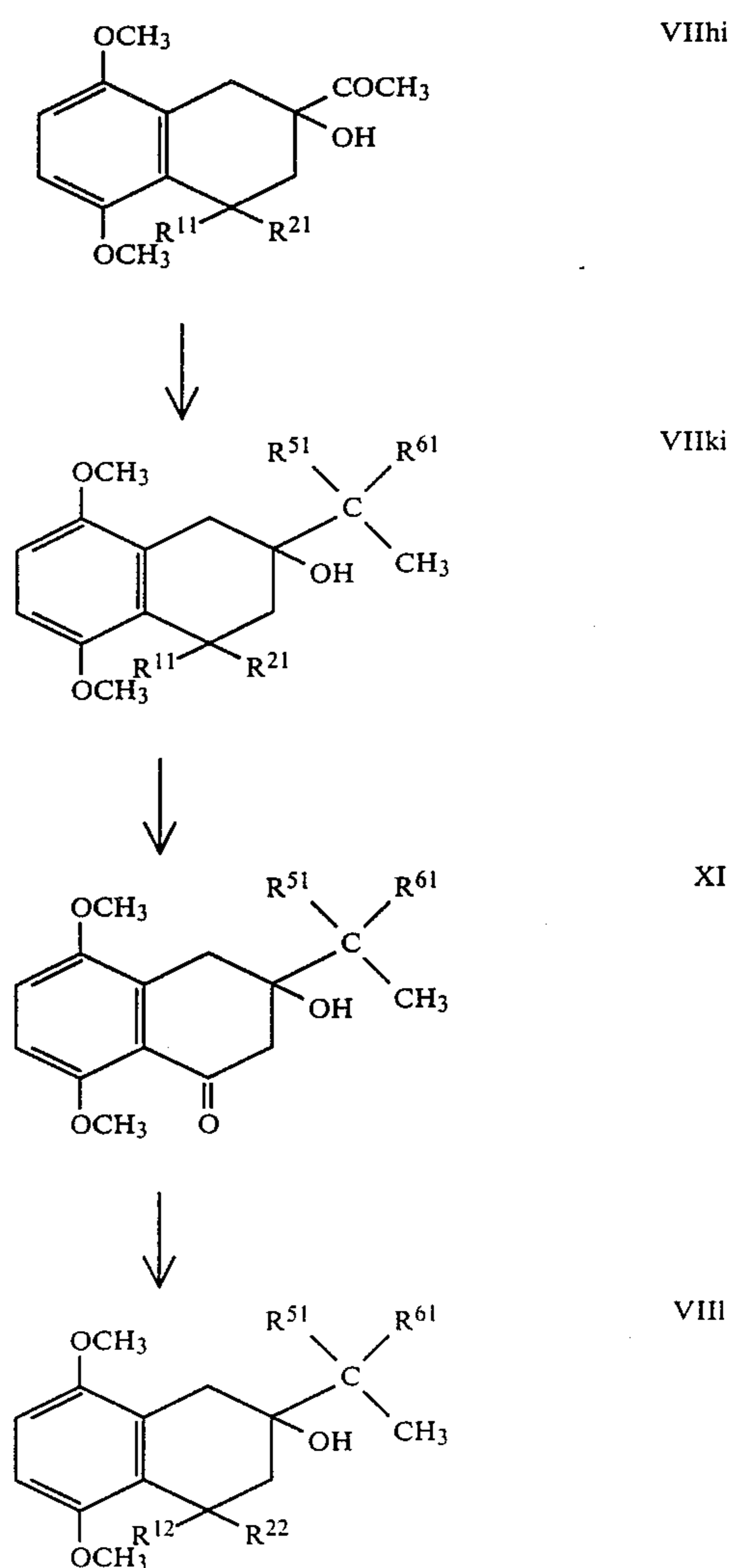
Formula Scheme III
