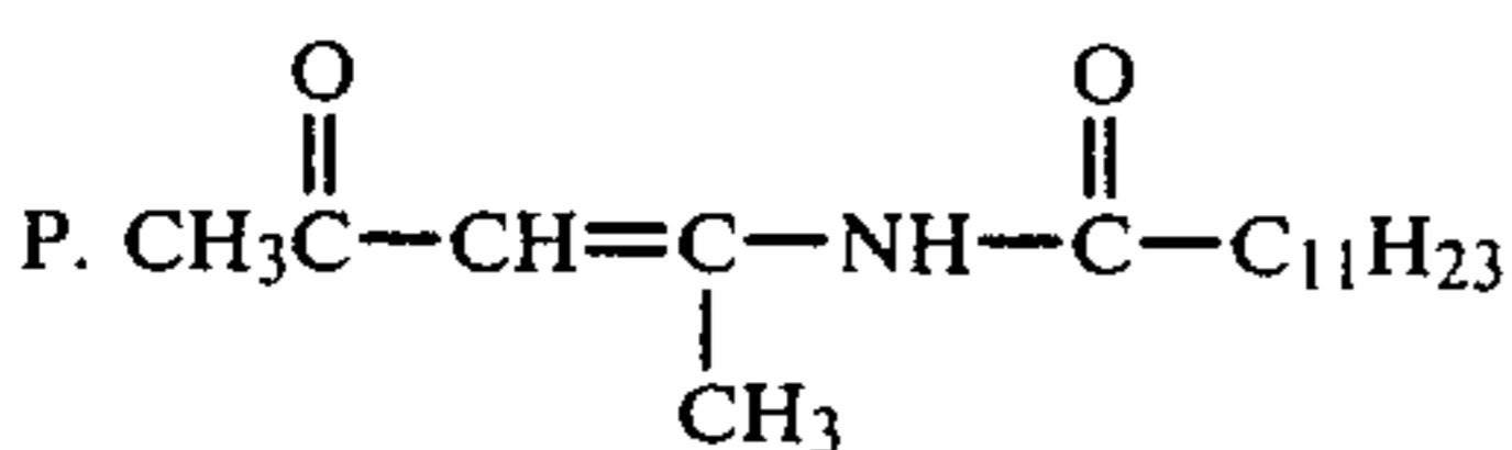
4-dodecanoylamino-3-pentene-2-one
