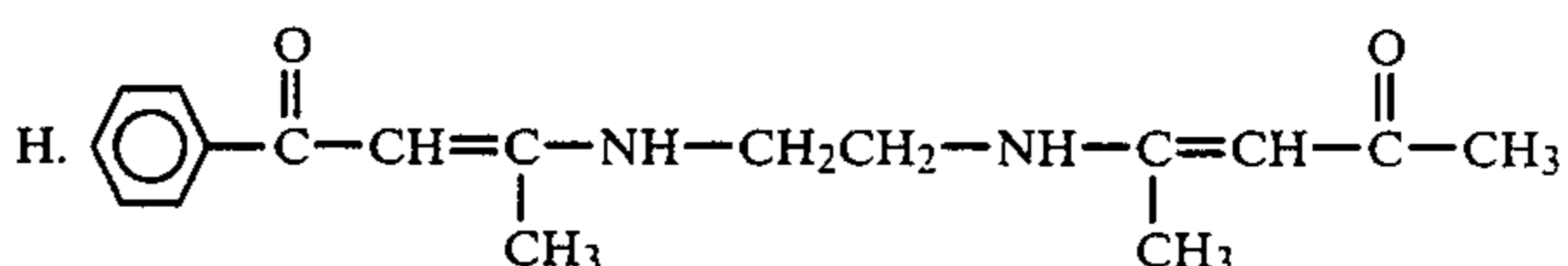
3-[2-(4'-amino-3'-pentene-2'-one)-ethylamino]-1-phenyl-2-butene-1-one
