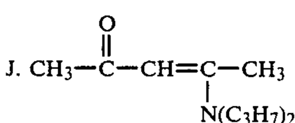
4-dipropylamino-3-pentene-2-one
