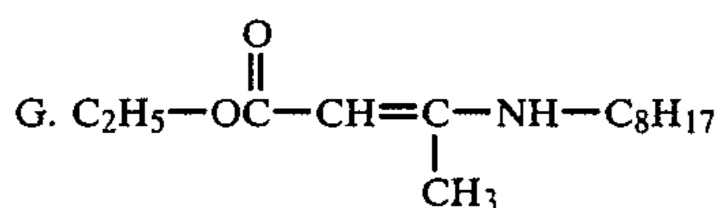
ethyl 3-octylamino-2-butenate
