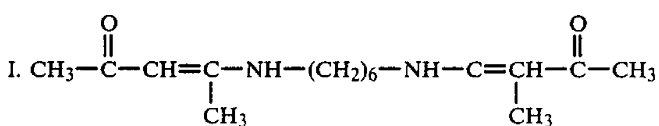
4-[6-(4'-amino-3'-pentene-2'-one)-hexylamino]-3-pentene-2-one
