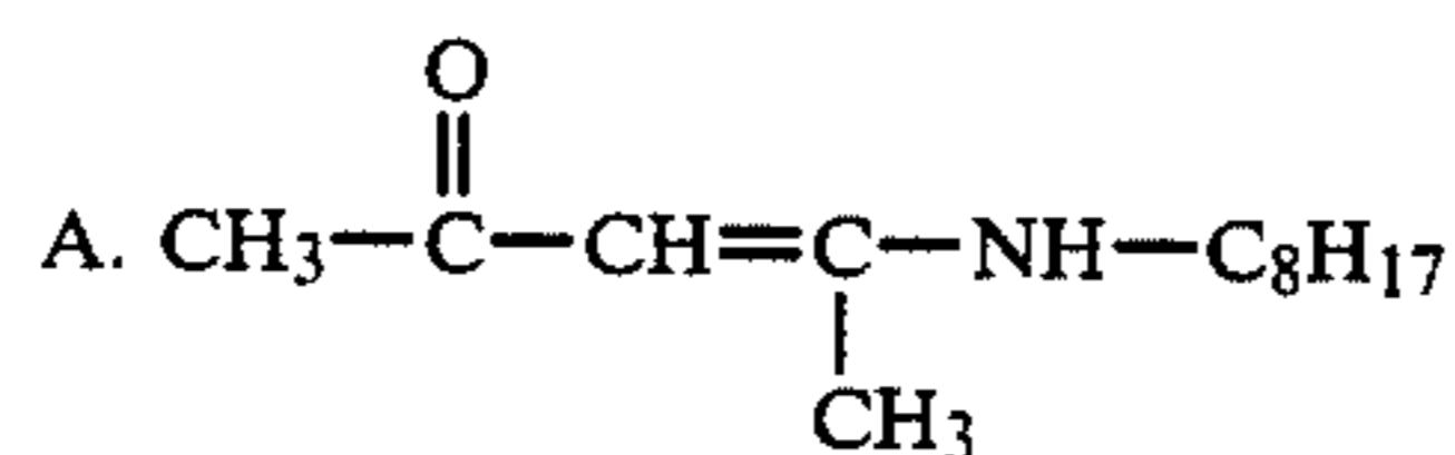
4-octylamino-3-pentene-2-one
