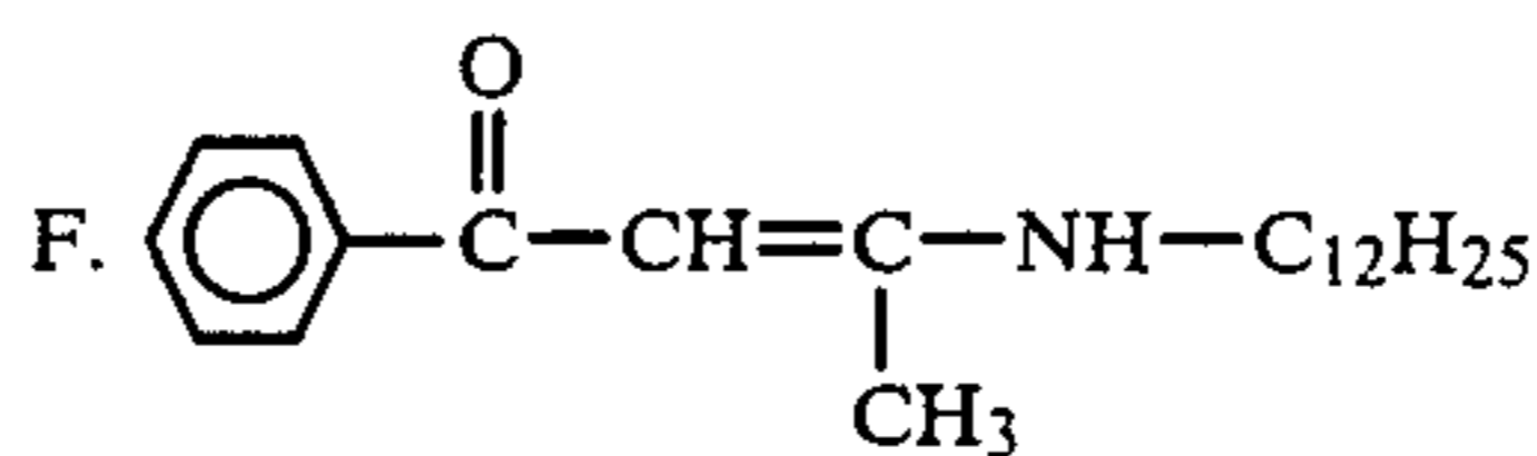
3-dodecylamino-1-phenyl-2-butene-1-one
