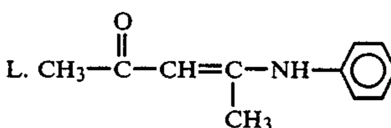
4-phenylamino-3-pentene-2-one
