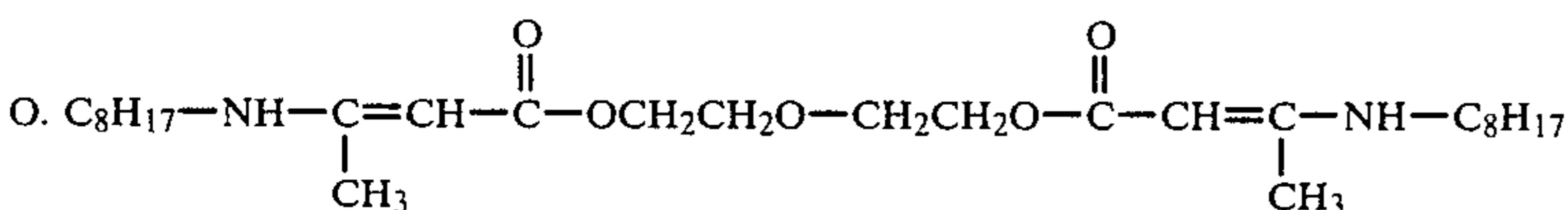
bis(3-octylamino-2-butenoyl)-B,B'-dioxyethylether
