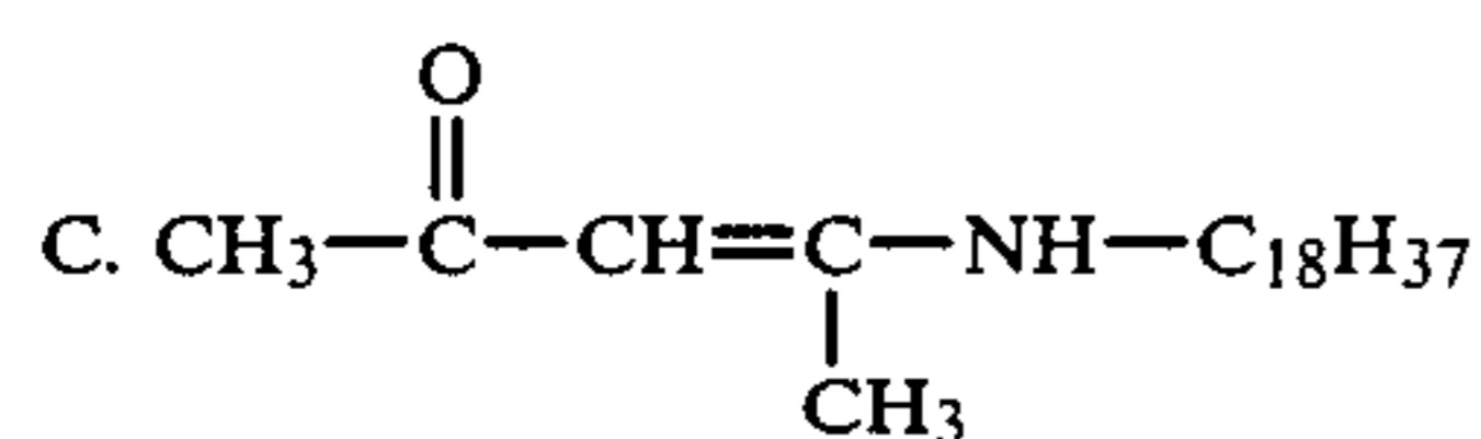
4-octadecylamino-3-pentene-2-one
