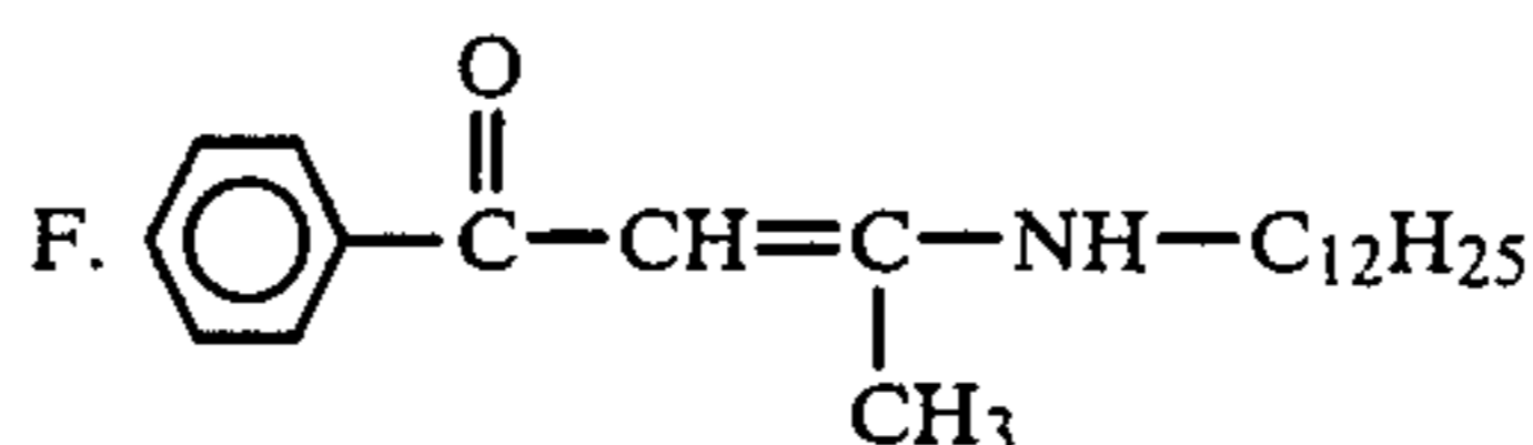
3-dodecylamino-1-phenyl-2-butene-1-one
