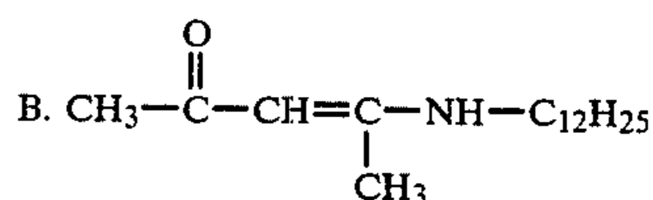
4-dodecylamino-3-pentene-2-one
