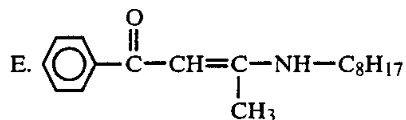
3-octylamino-1-phenyl-2-butene-1-one
