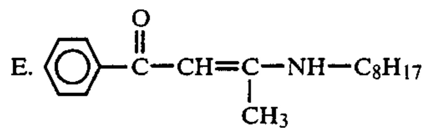
3-octylamino-1-phenyl-2-butene-1-one
