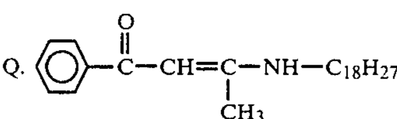
3-octadecylamino-1-phenyl-2-butene-1-one
