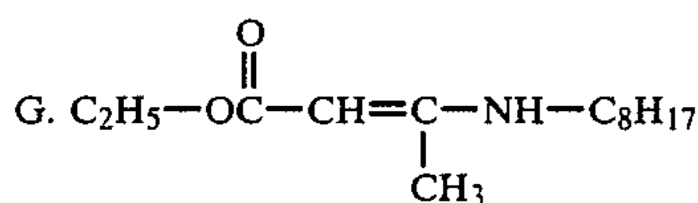
ethyl 3-octylamino-2-butenate
