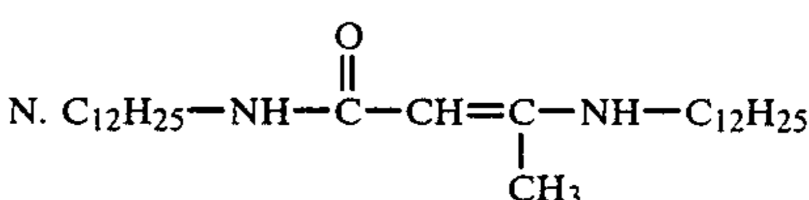
dodecyl 3-dodecylamino-2-butenamide
