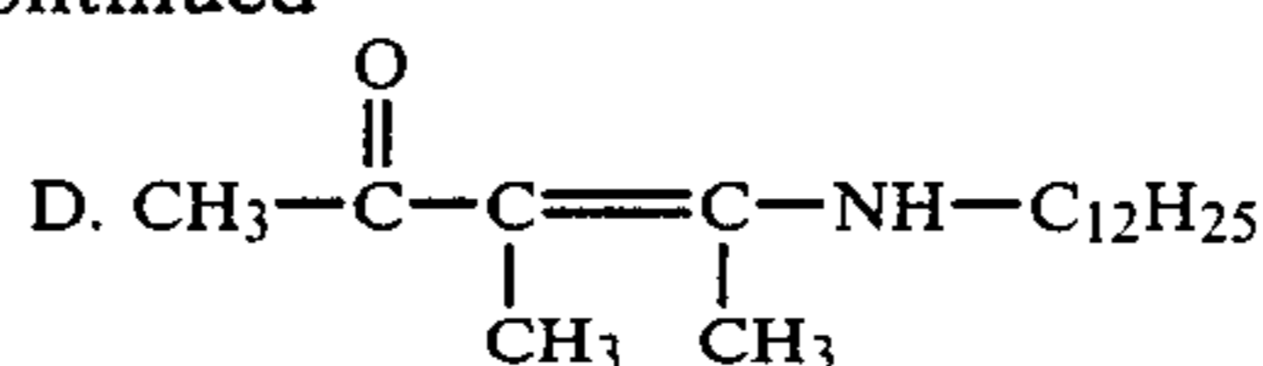
4-dodecylamino-3-methyl-3-pentene-2-one
