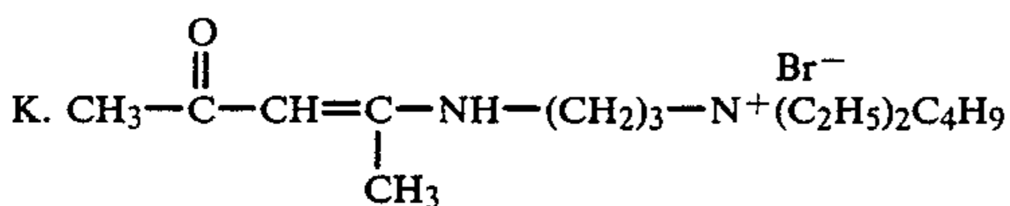
4-(3-butyl-diethylammonium)-propylamino-3-pentene-2-one bromide
