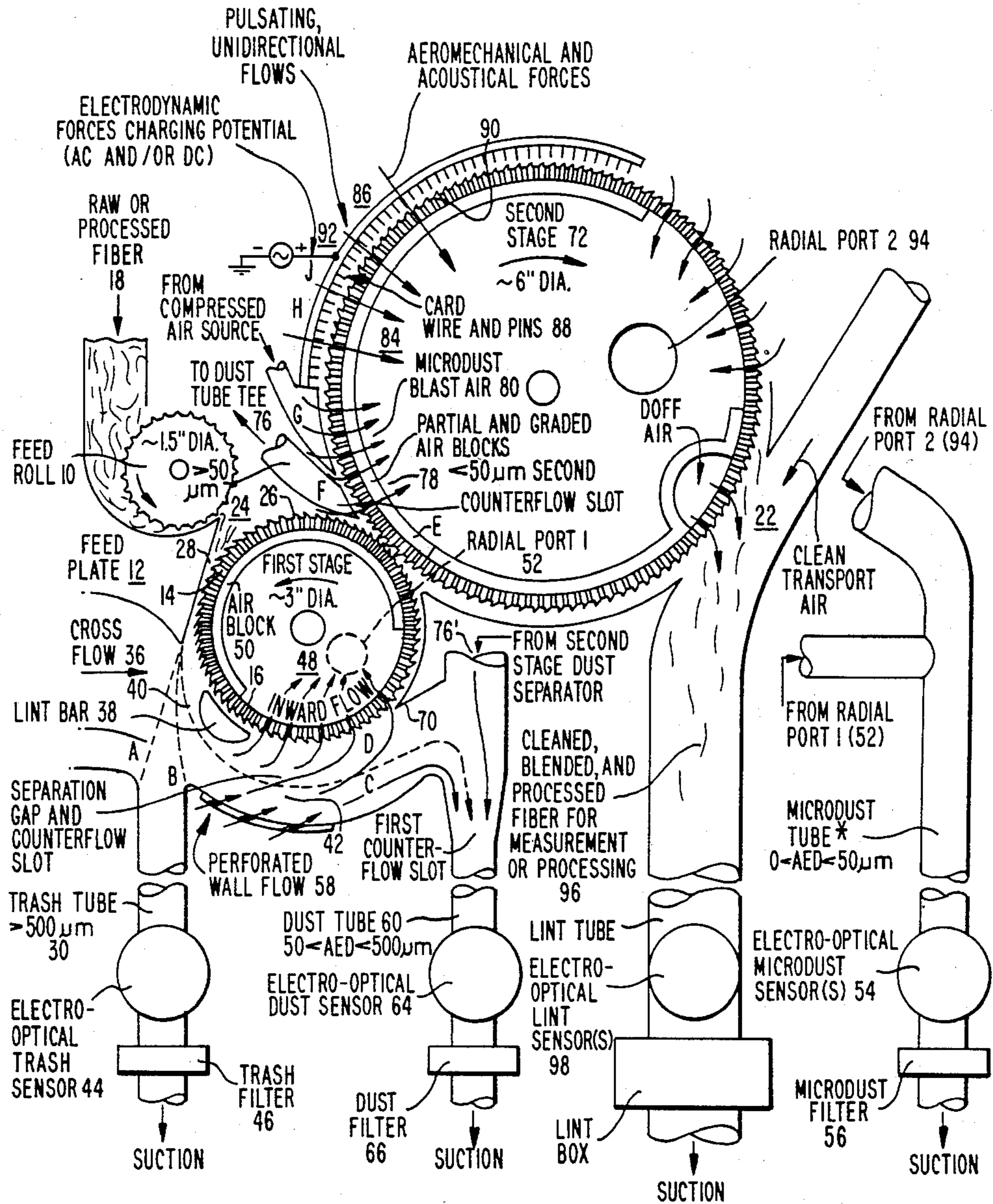
BASIC APPARATUS
