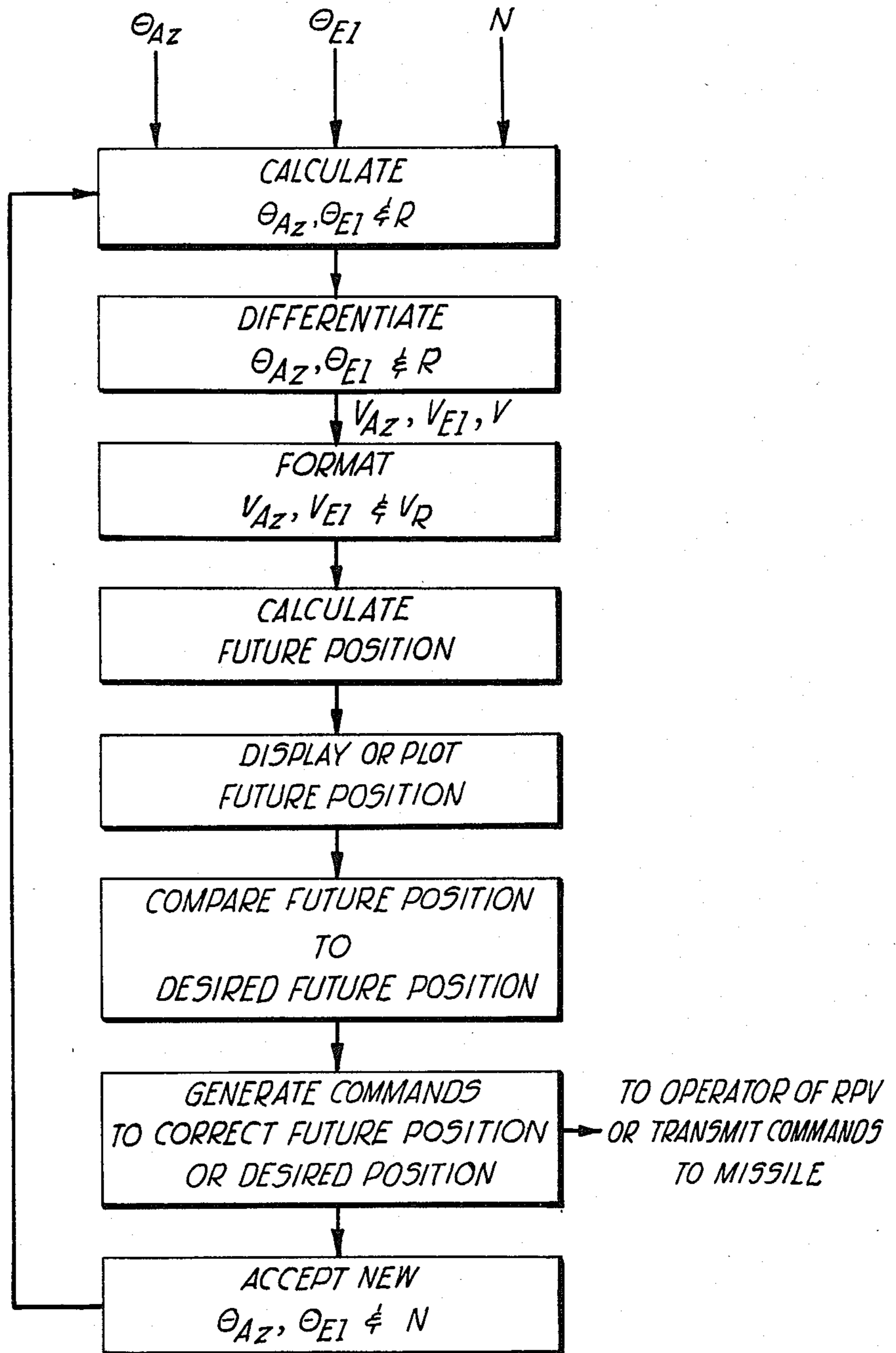
RPV or missile command guidance processor.
