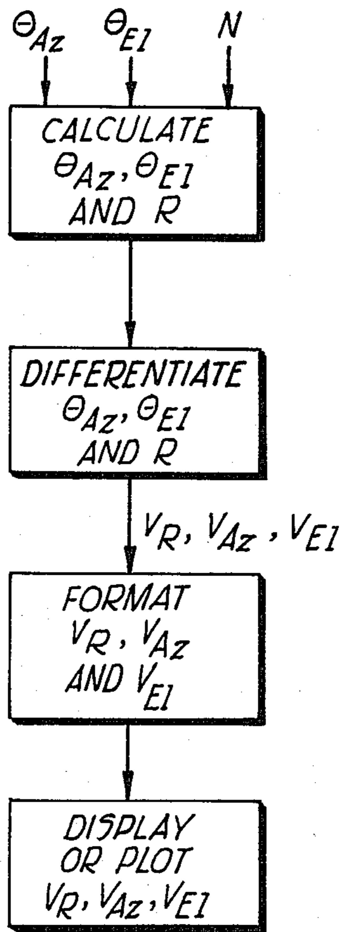
Simple target velocity vector processor.
