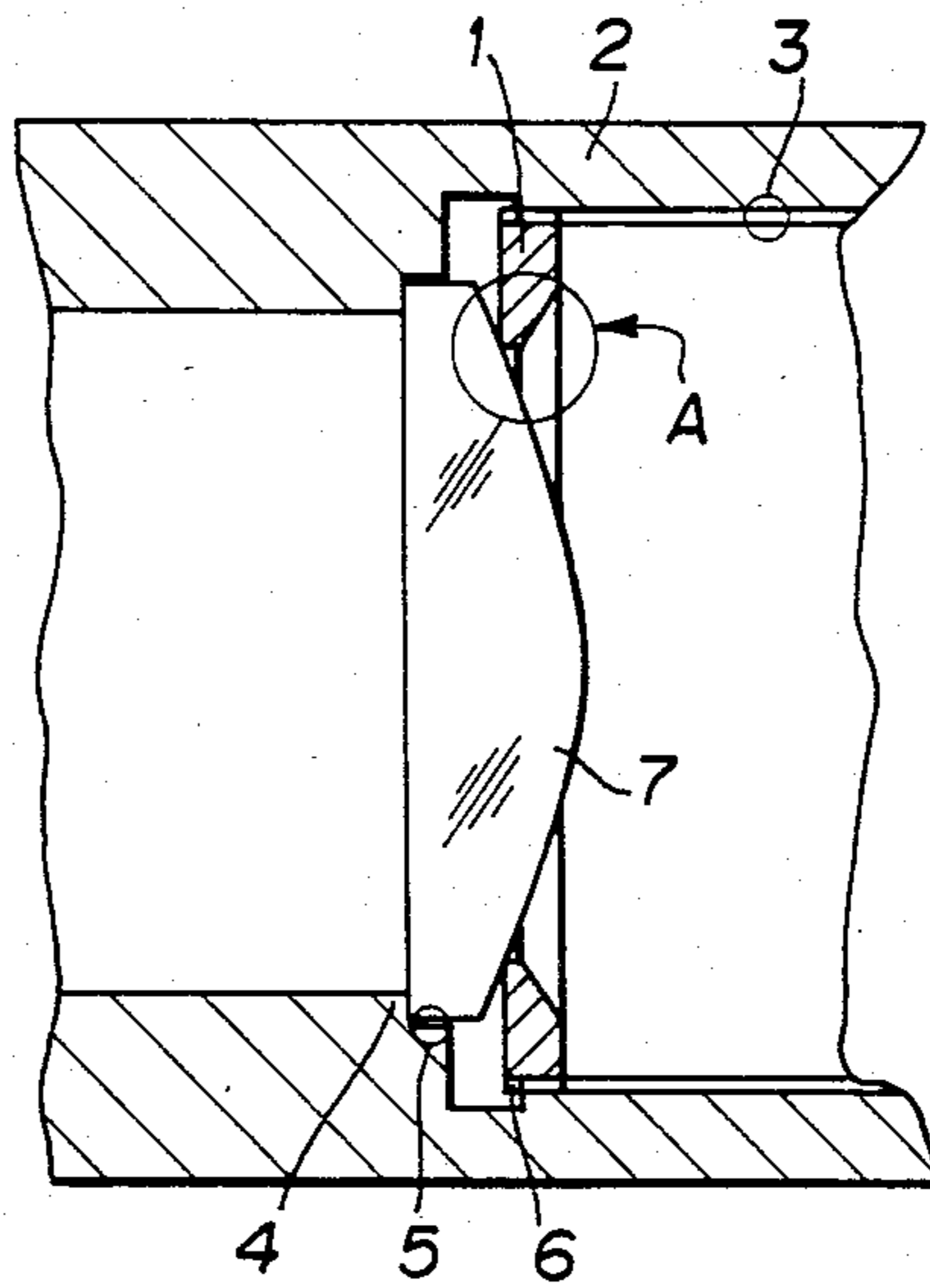
PRIOR ART FIG. 1(a)
