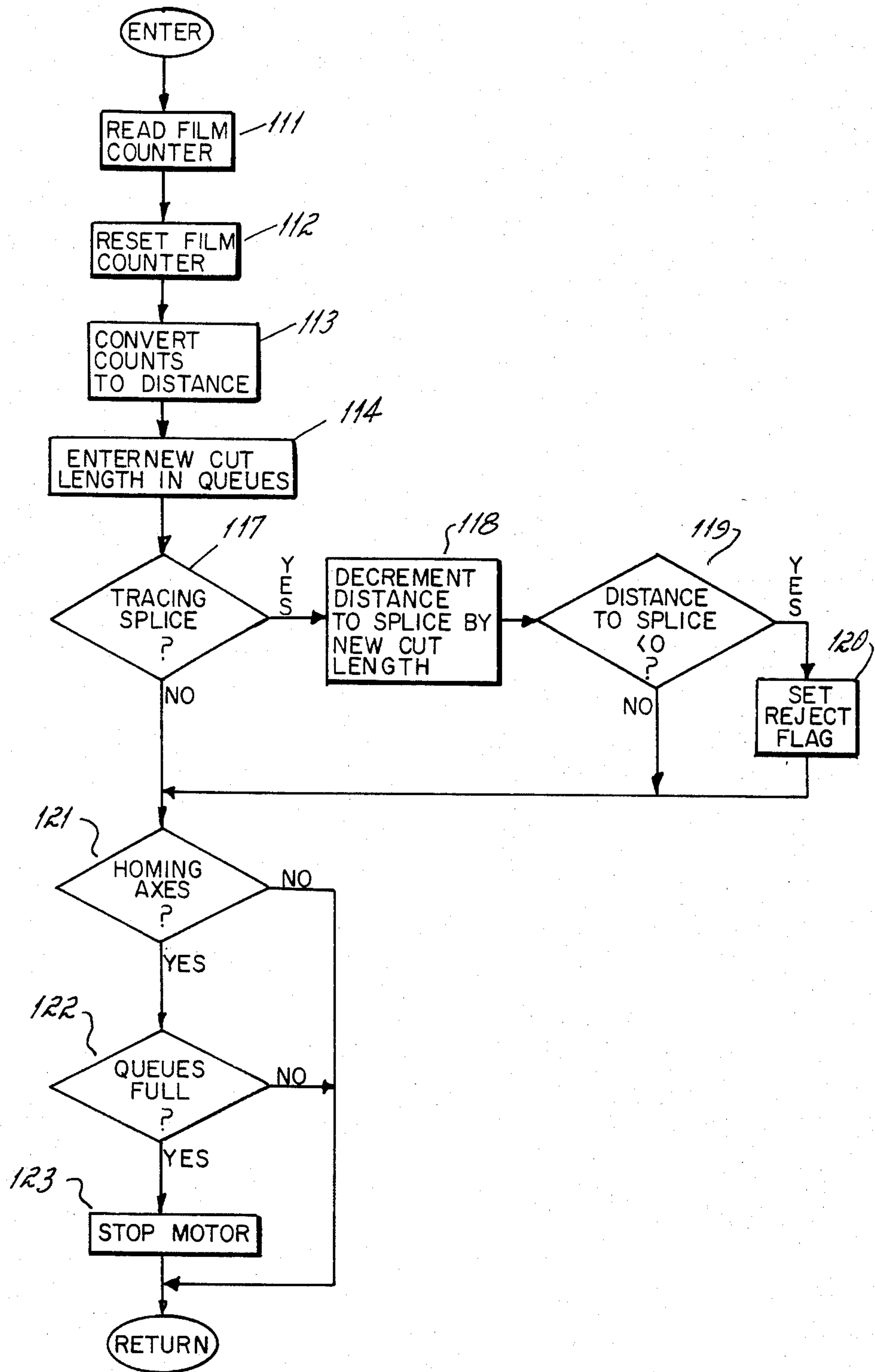
FILM FEED INTERRUPT ROUTINE
