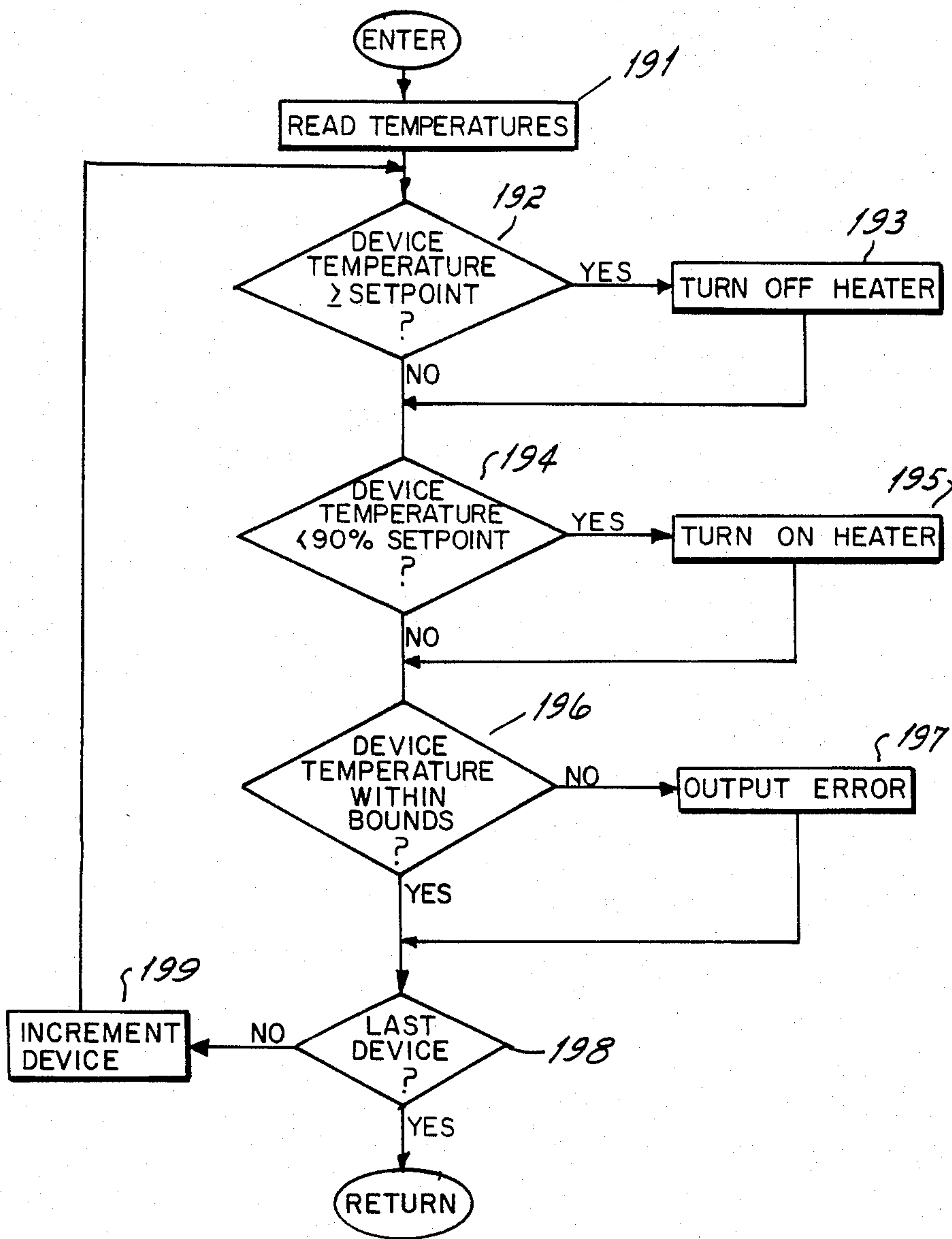
TEMPERATURE INTERRUPT ROUTINE
