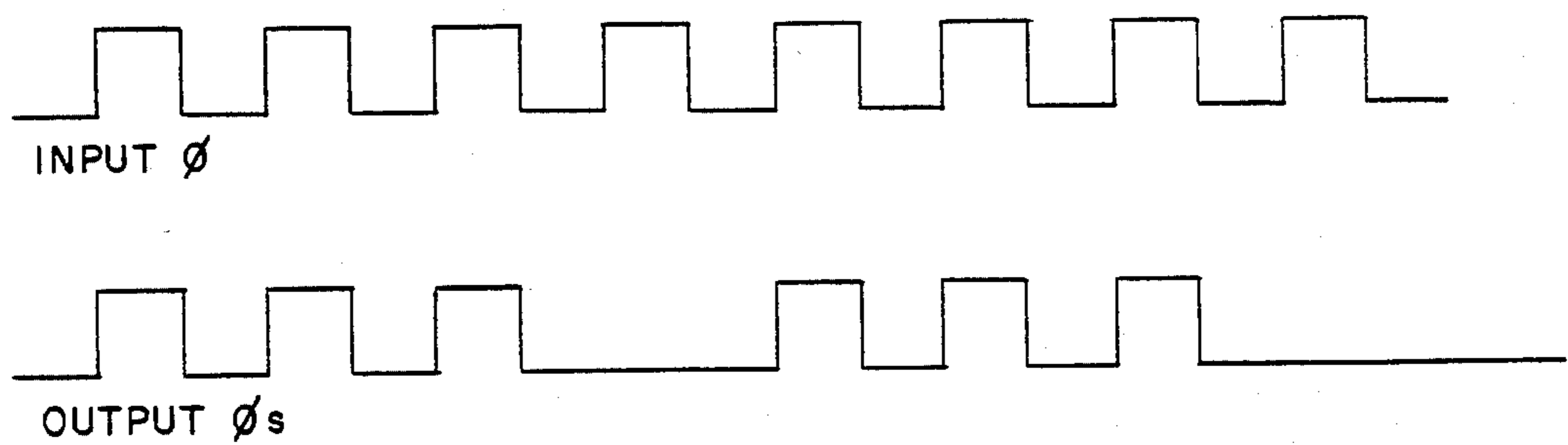
INPUT / OUTPUT OF A TWO STAGE BRM
