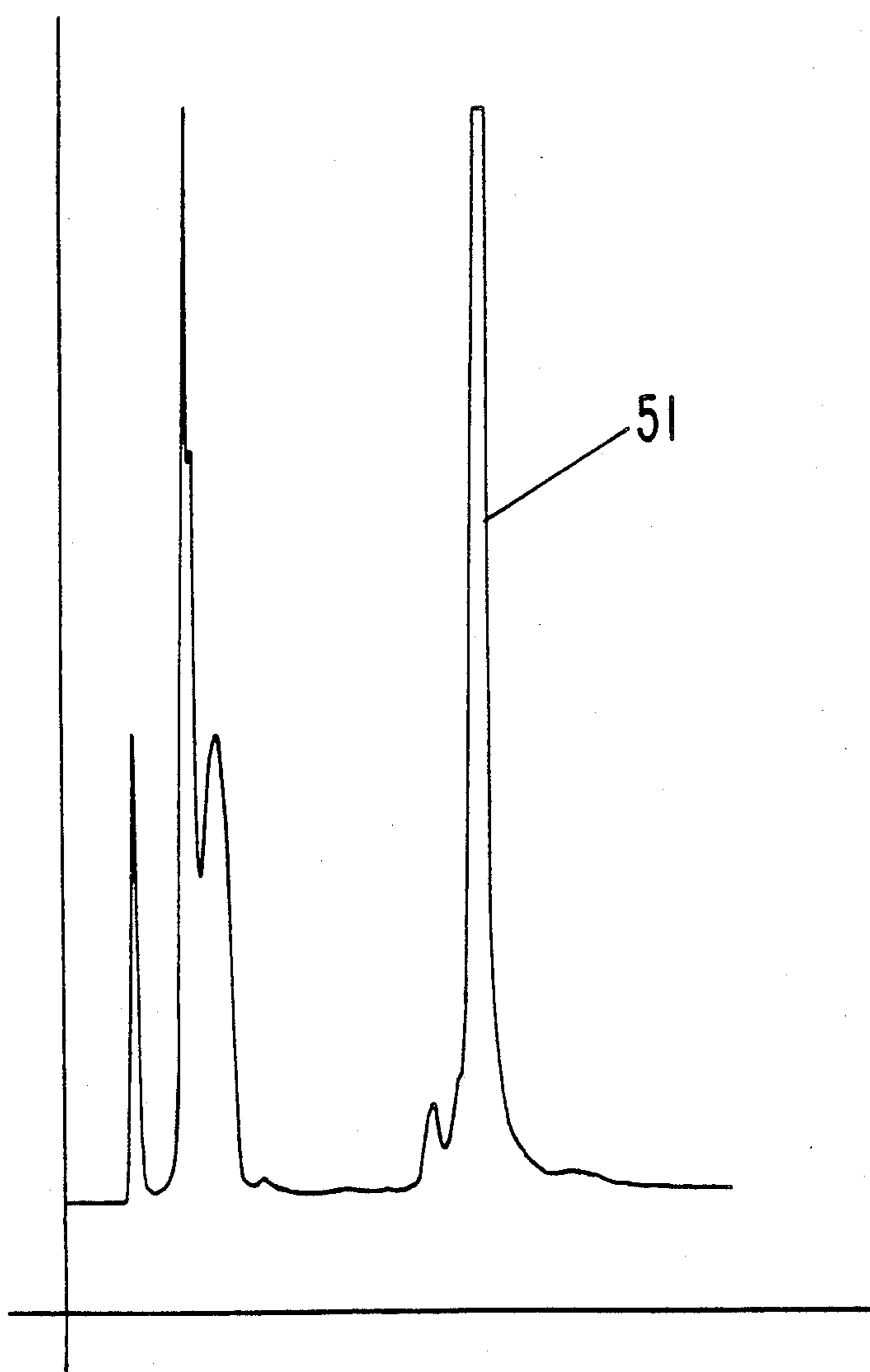
GLC PROFILE FOR EXAMPLE XI(B).
