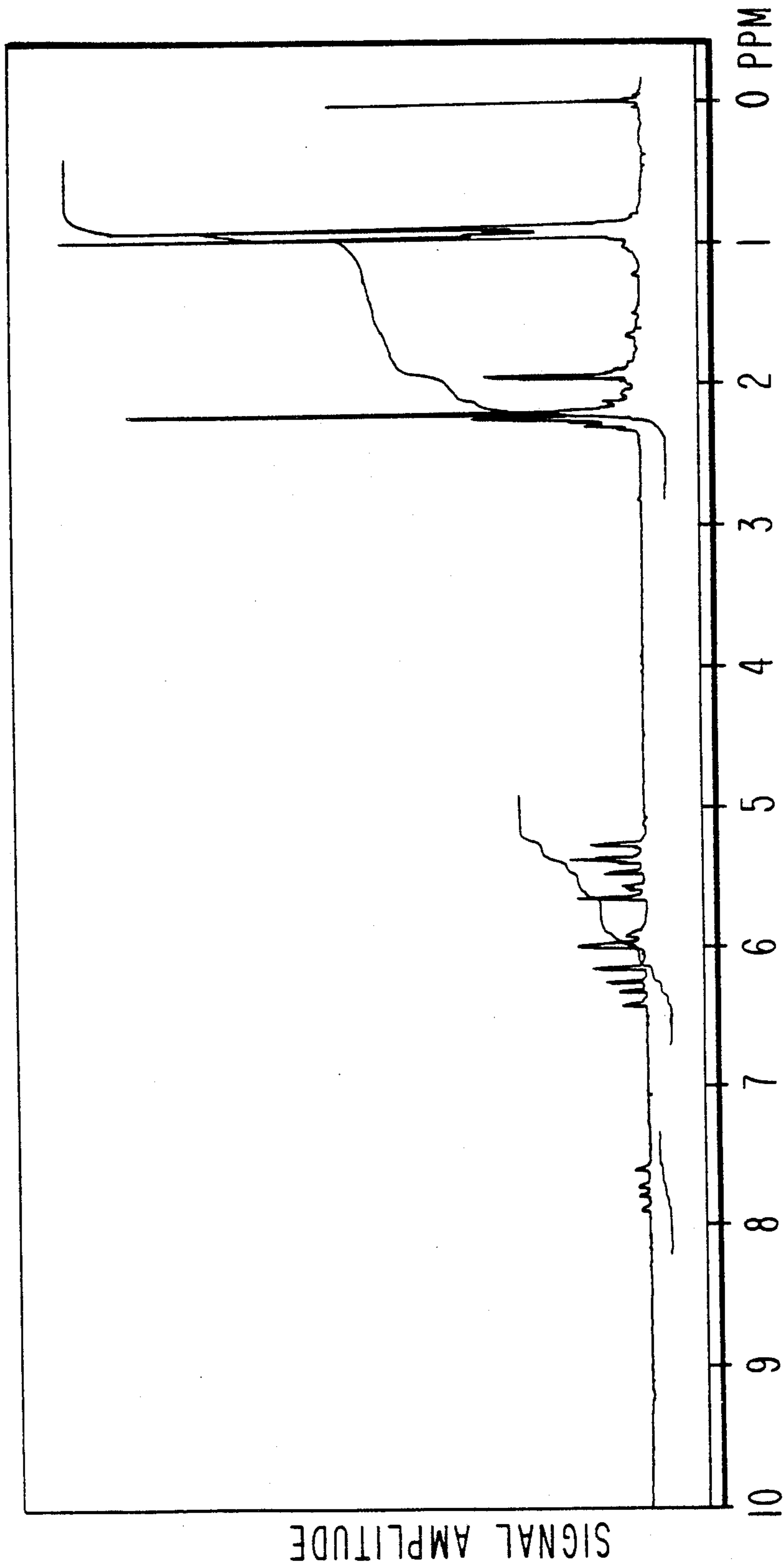
NMR SPECTRUM FOR EXAMPLE II.
