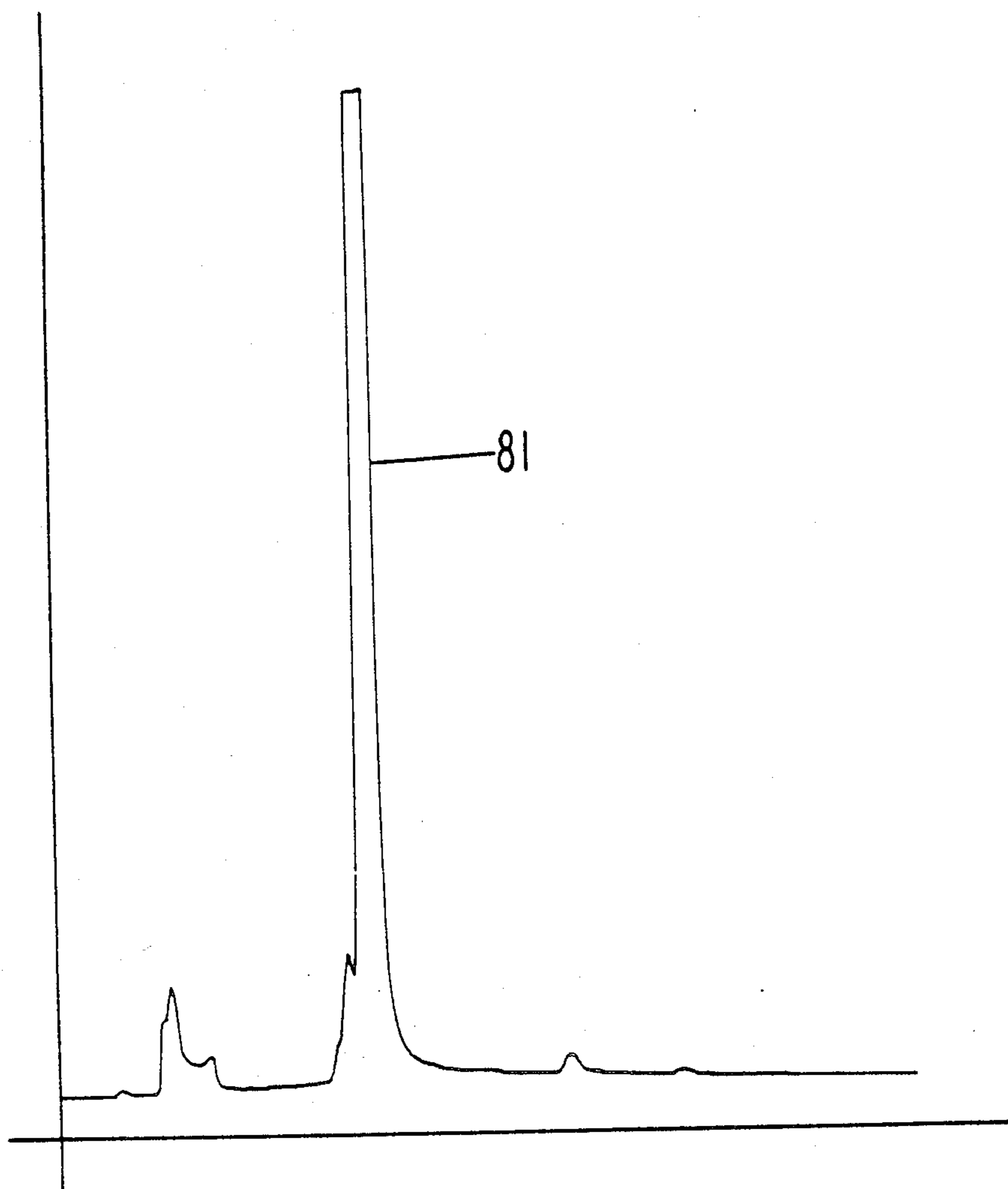
GLC PROFILE FOR EXAMPLE VII B .
