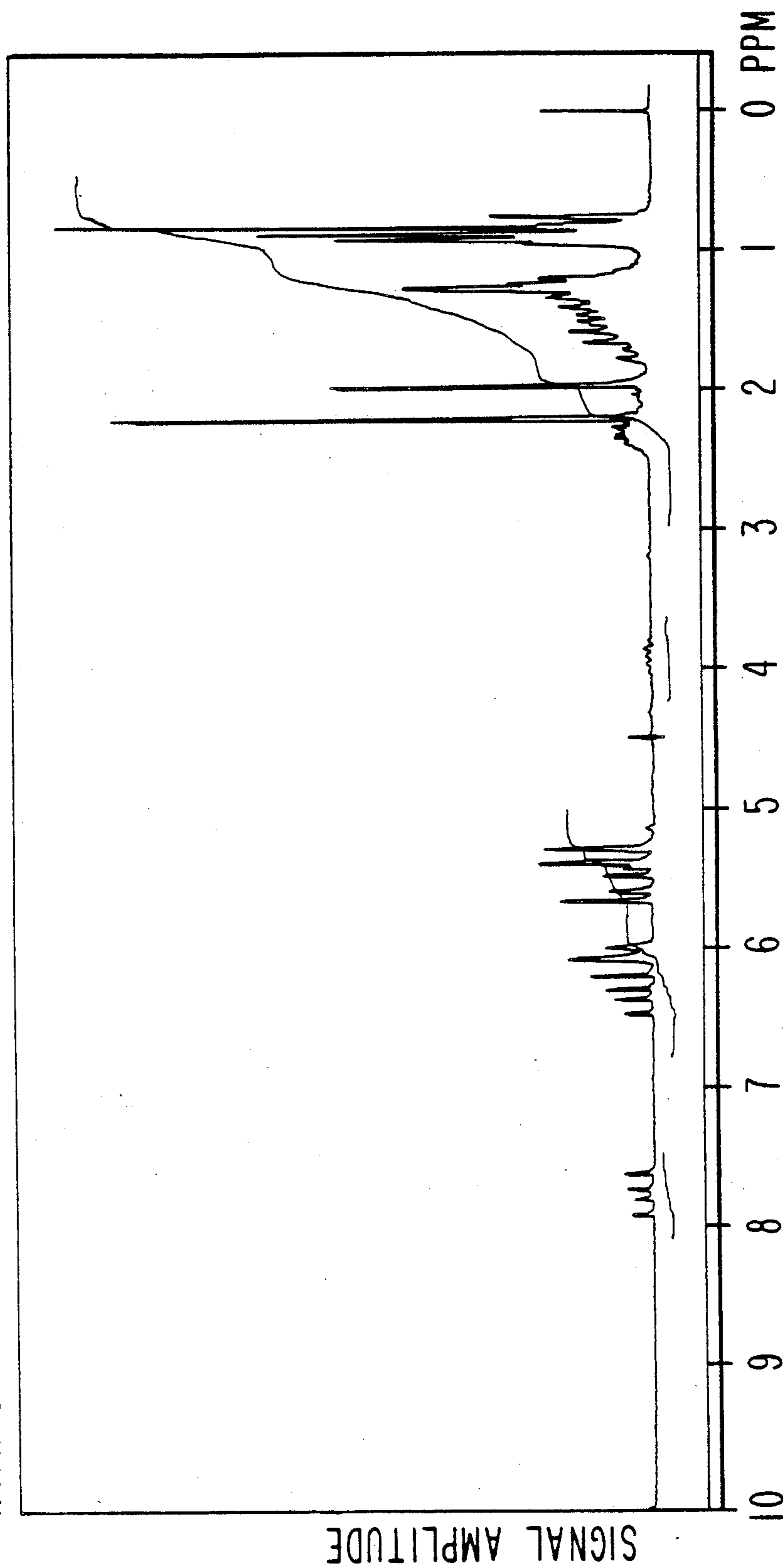
NMR SPECTRUM FOR EXAMPLE VII B.
