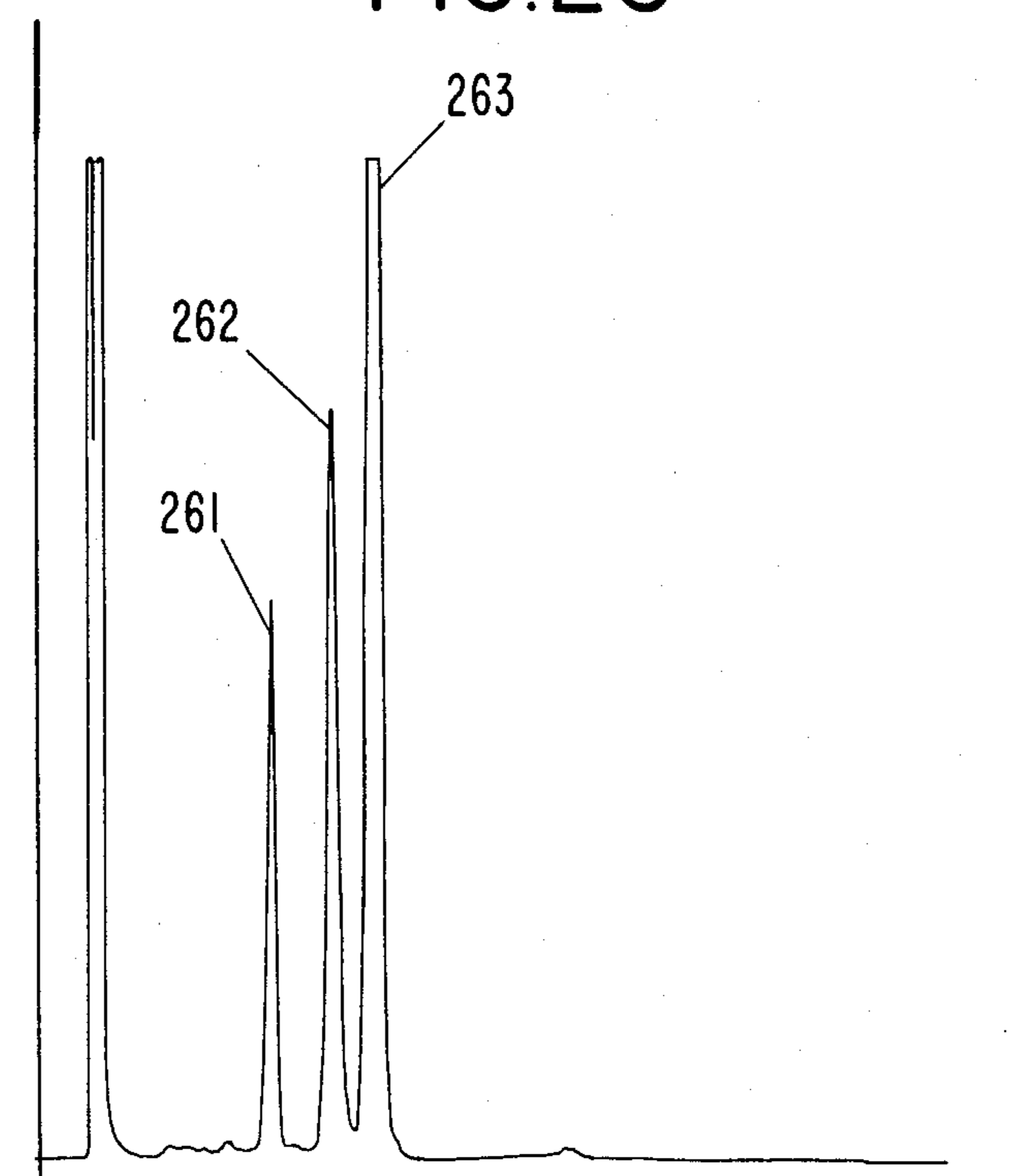
GLC PROFILE FOR EXAMPLE XX (A)
