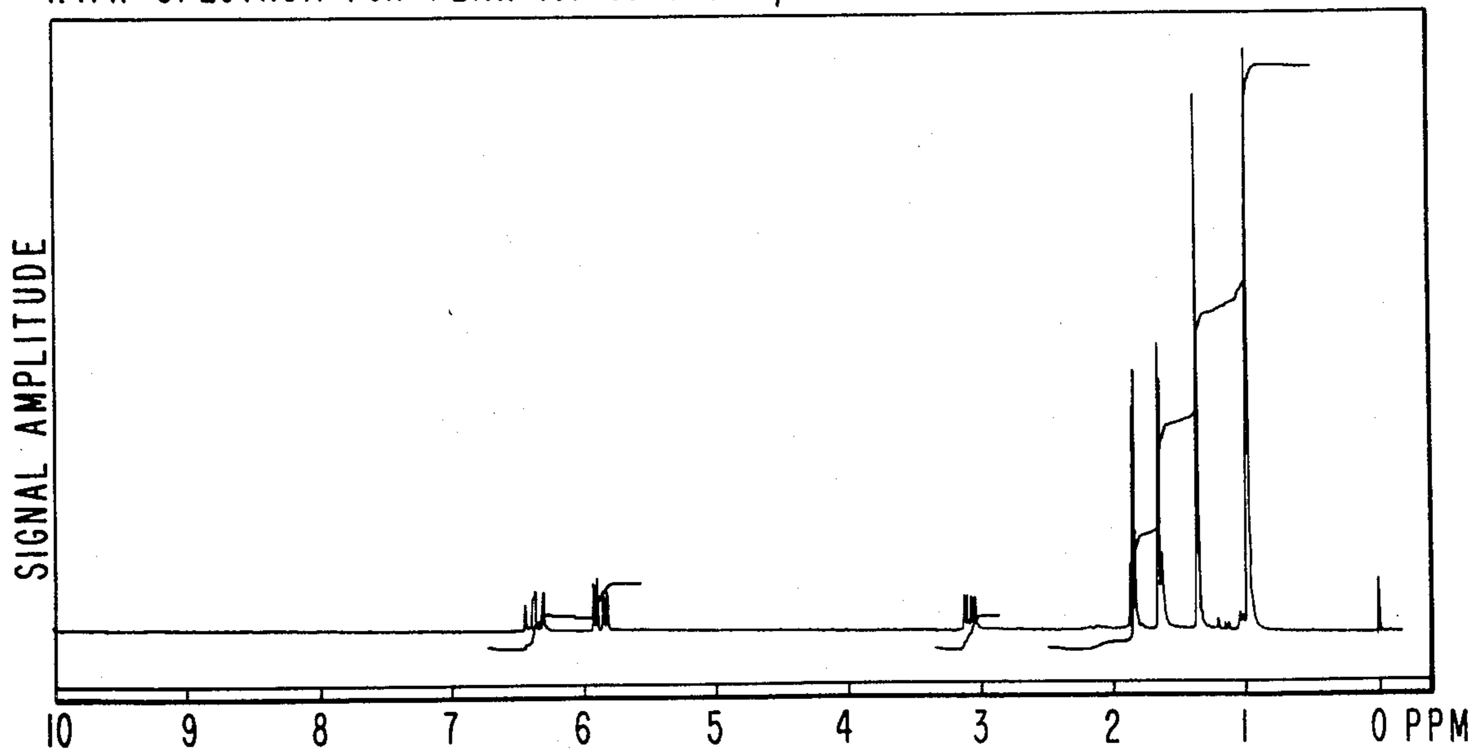
NMR SPECTRUM FOR PEAK 101 OF FIG.1 , EXAMPLE I.
