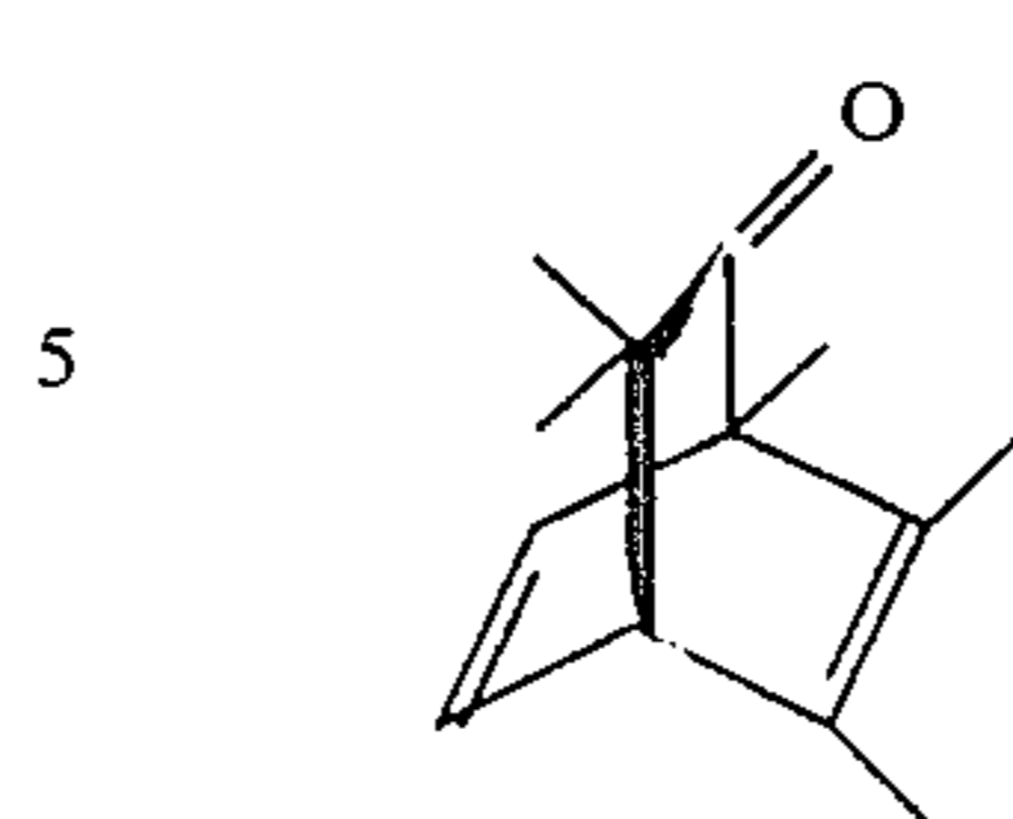
FIG. 5 is the GLC profile for the reaction product of Example II. The peak indicated on FIG. 5 by reference numeral "501" is the peak for the compound having the structure:
