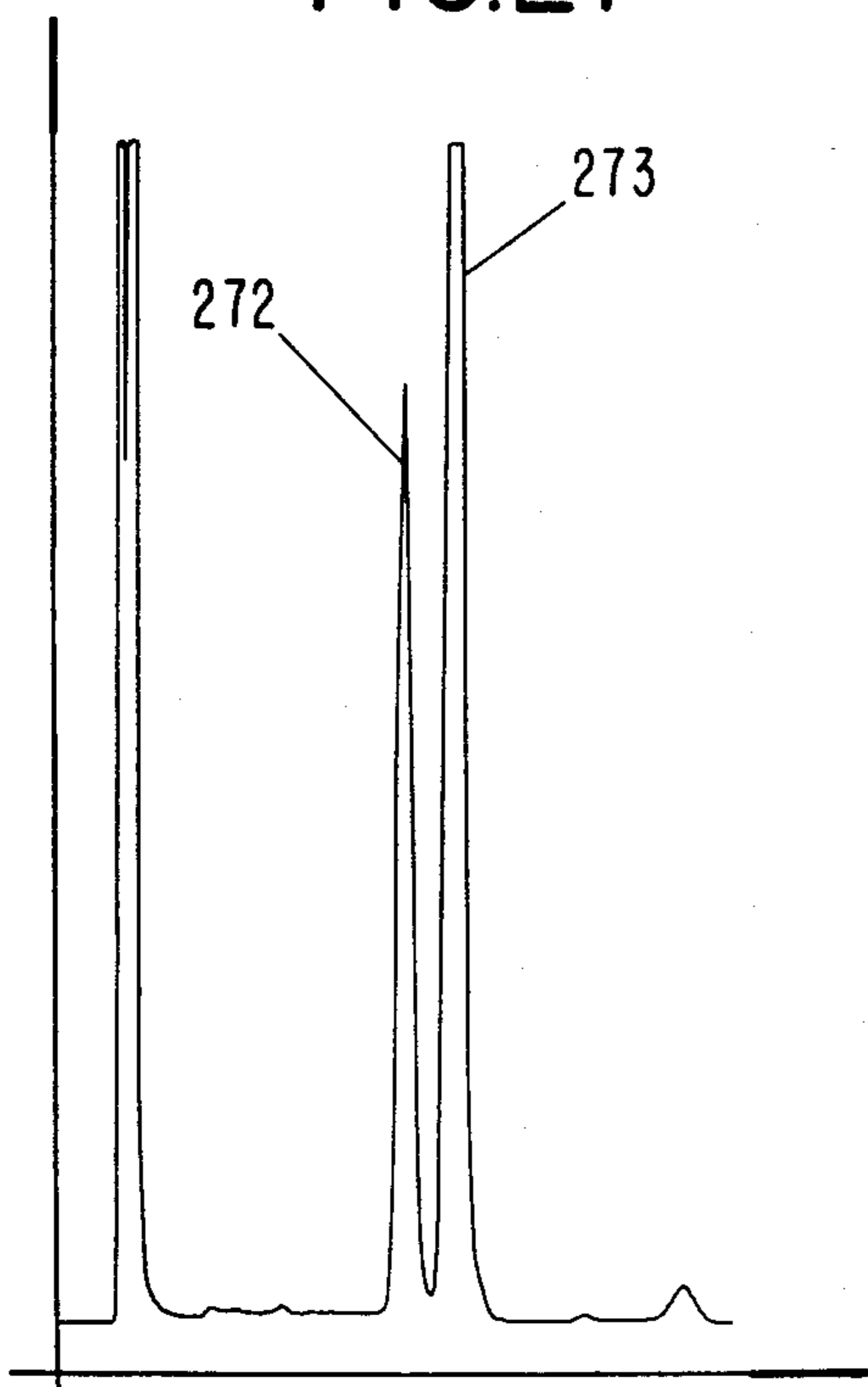
GLC PROFILE FOR EXAMPLE XX (B)
