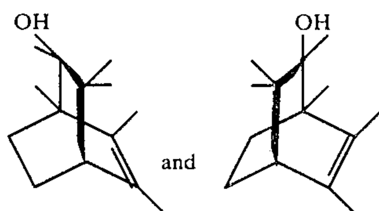
FIG. 26 is the GLC profile of the reaction product of Example XX(A) containing the isomers having the structures:
