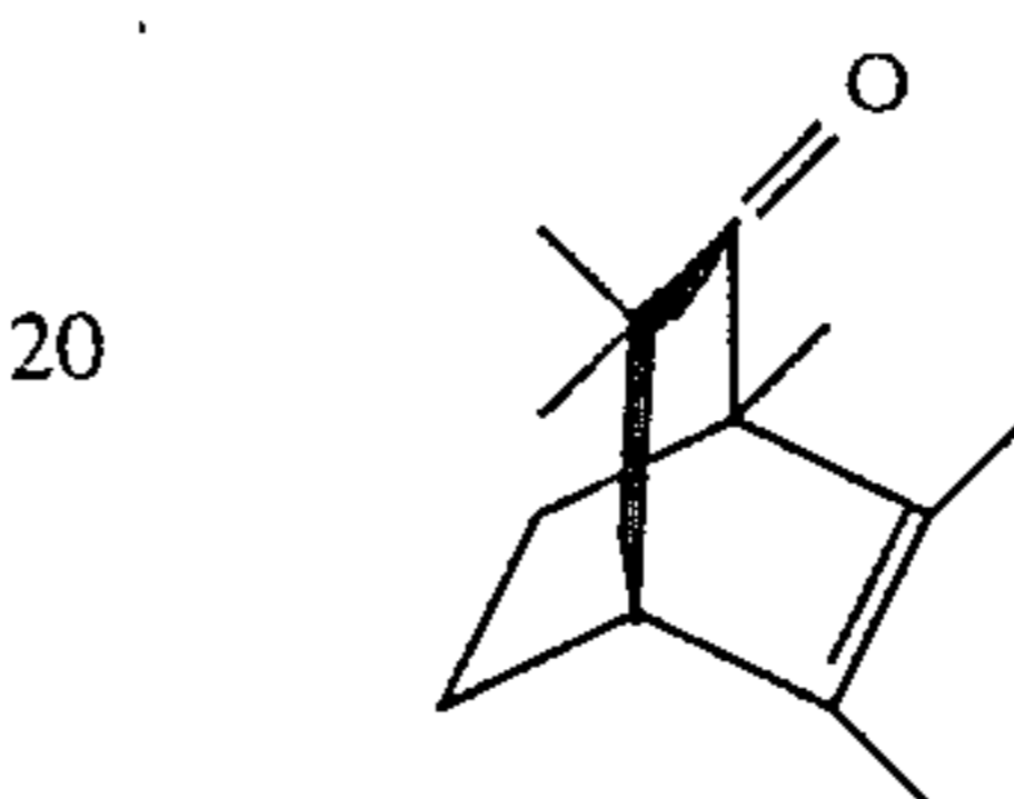
FIG. 9 is the GLC profile for fraction 2 of the distillation product of the reaction product of Example III containing the compounds defined according to the structures:
