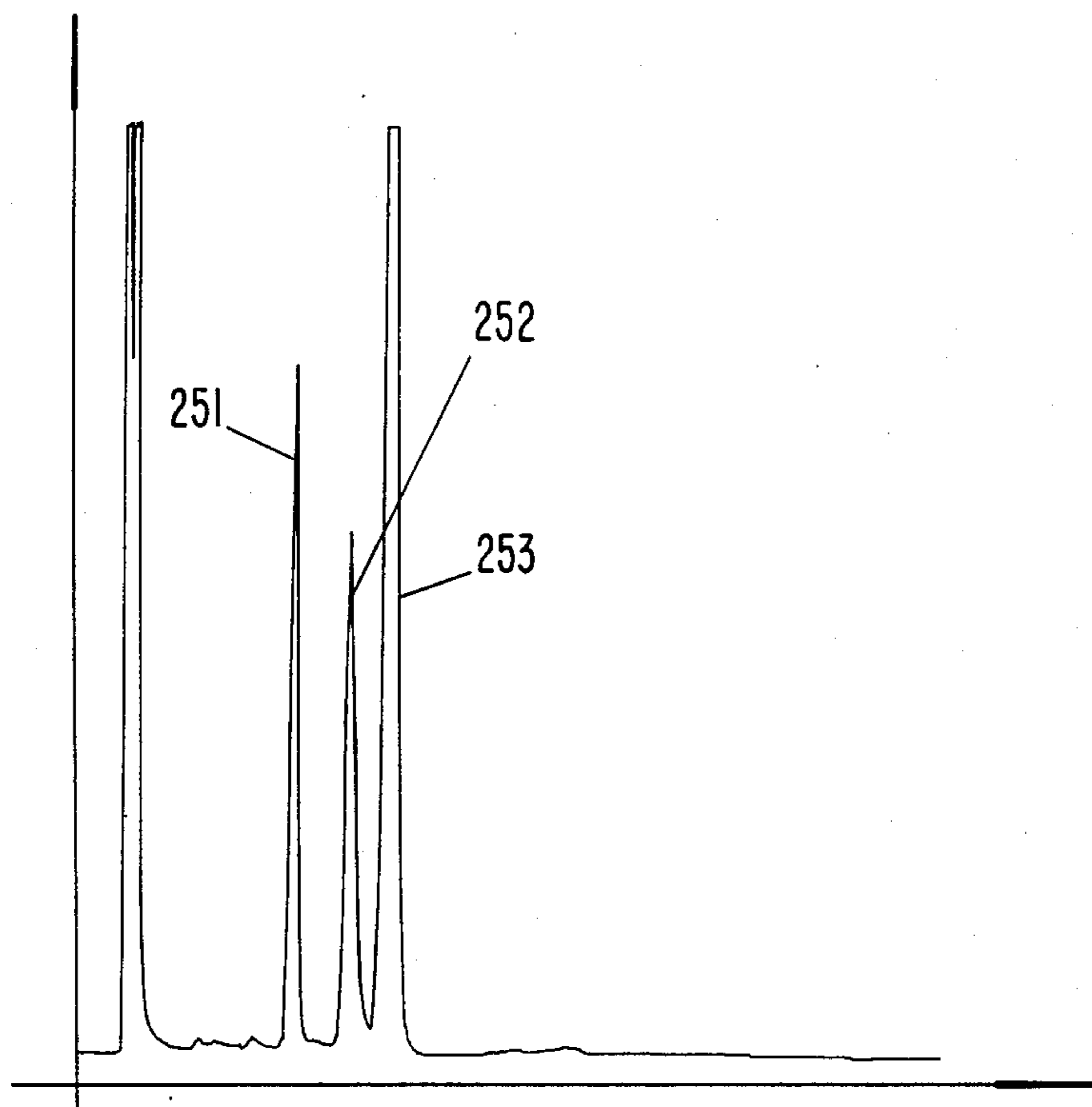
GLC PROFILE FOR EXAMPLE XX .
