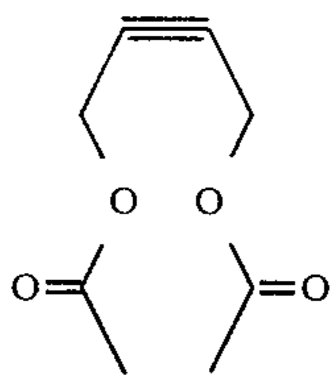
FIG. 20 is the GLC profile for the reaction product of Example V containing the compound having the structure:
