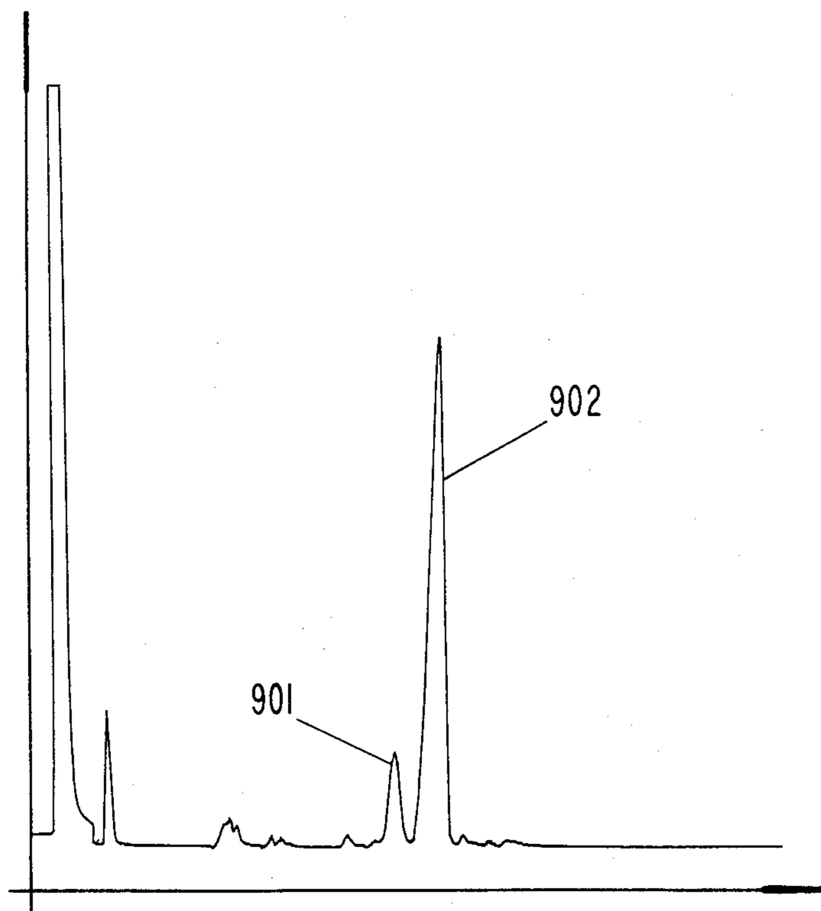
GLC PROFILE FOR EXAMPLE III.
