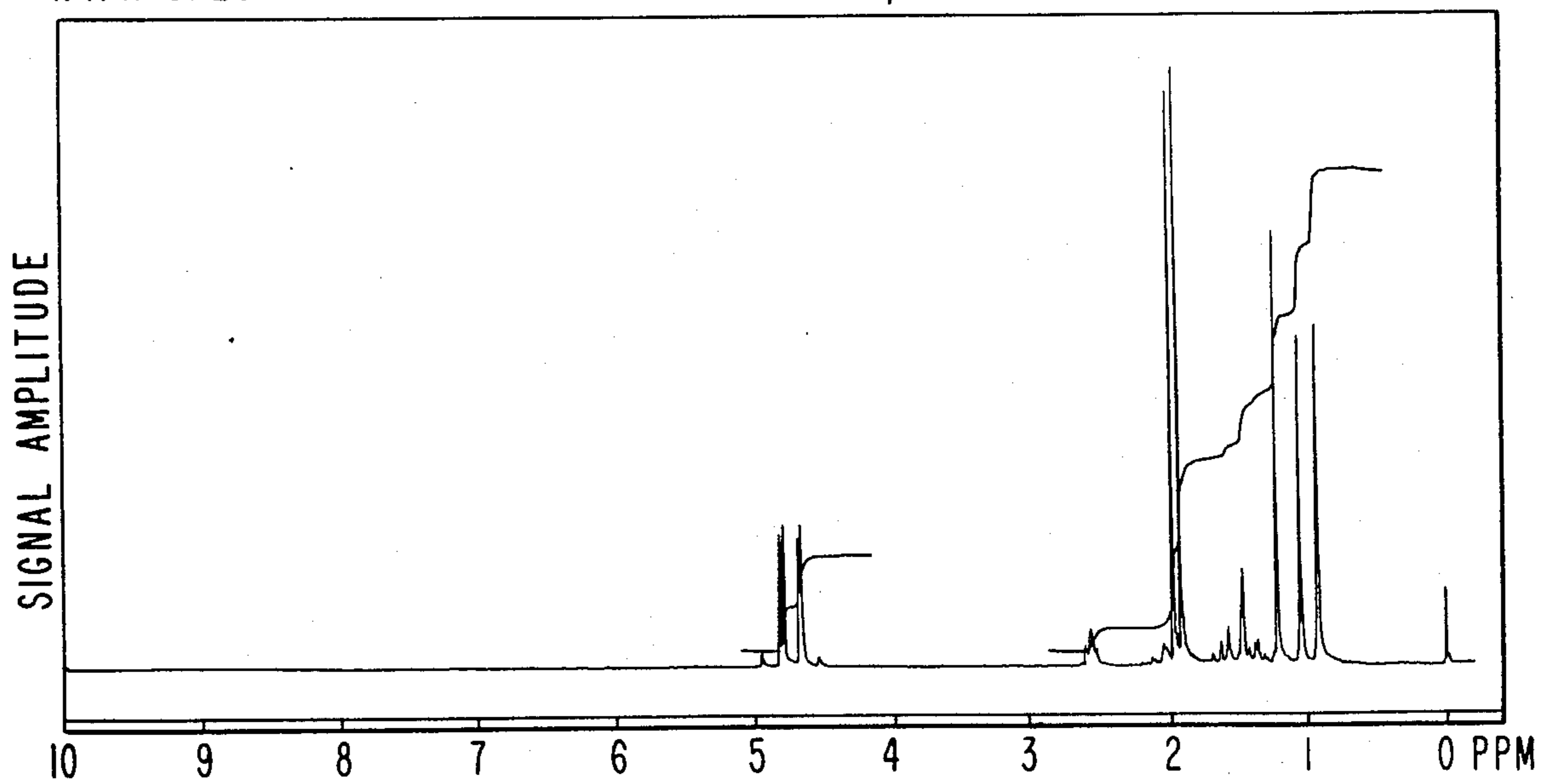
NMR SPECTRUM FOR PEAK 201 OF FIG. 20, EXAMPLE V.
