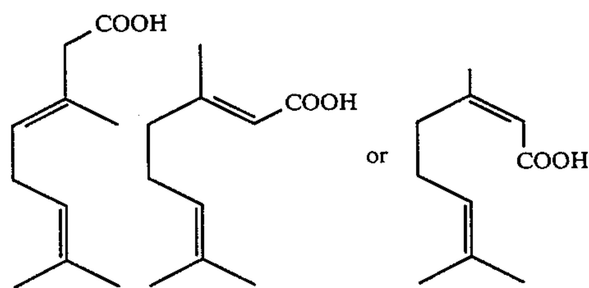
trans-isogeranic acid
