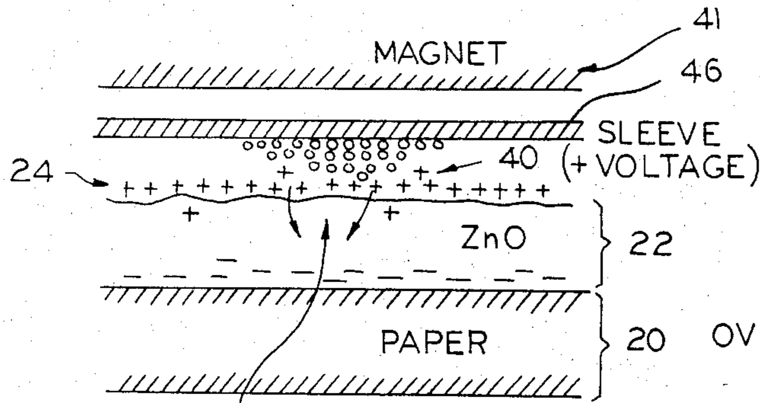
POSSIBLE NEUTRALISING CURRENT PATH FIG. 3
