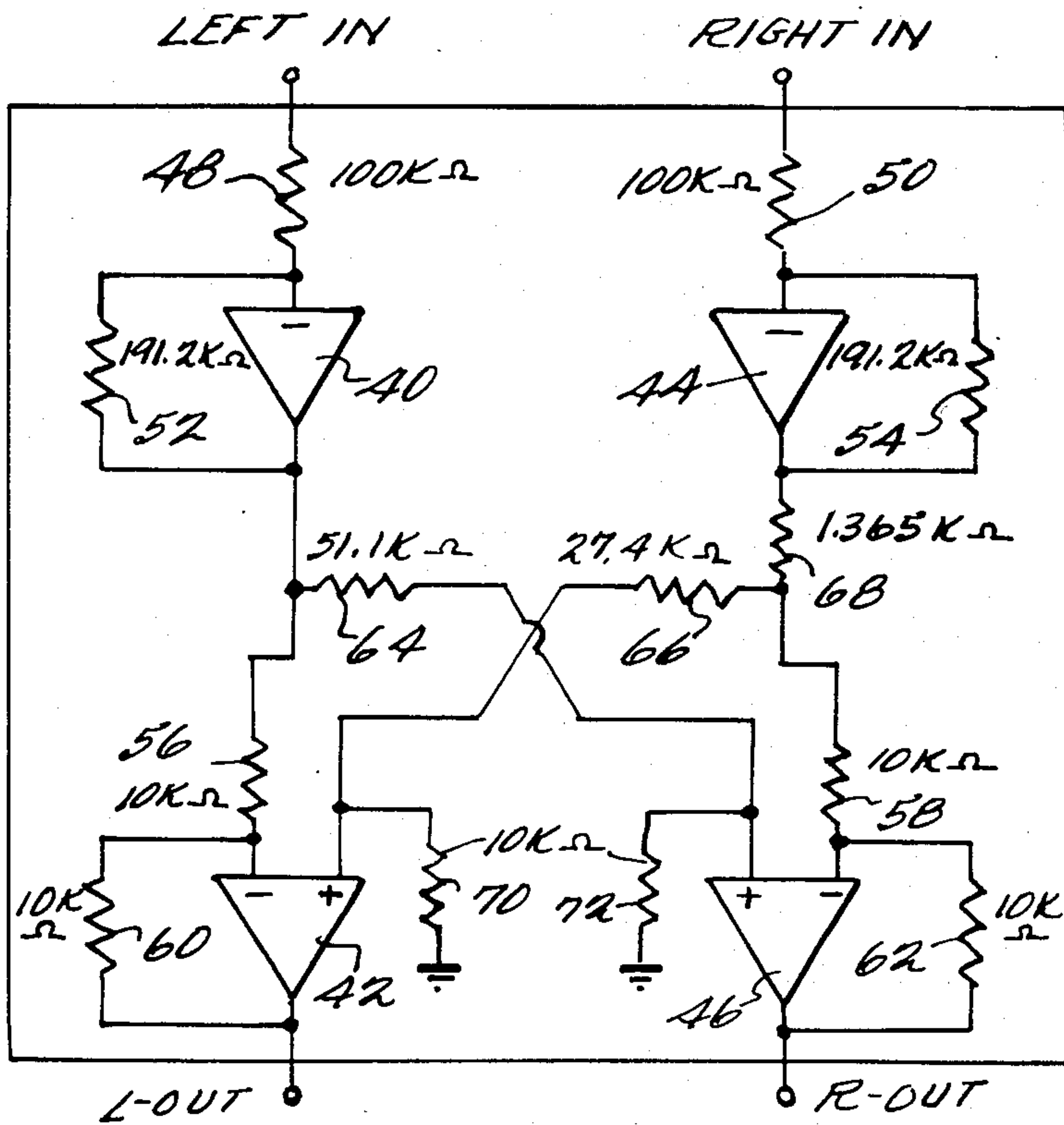
FIG. 3 TYPICAL RIGHT-HANDED ASYMMETRIC CROSS-FEED CIRCUIT
