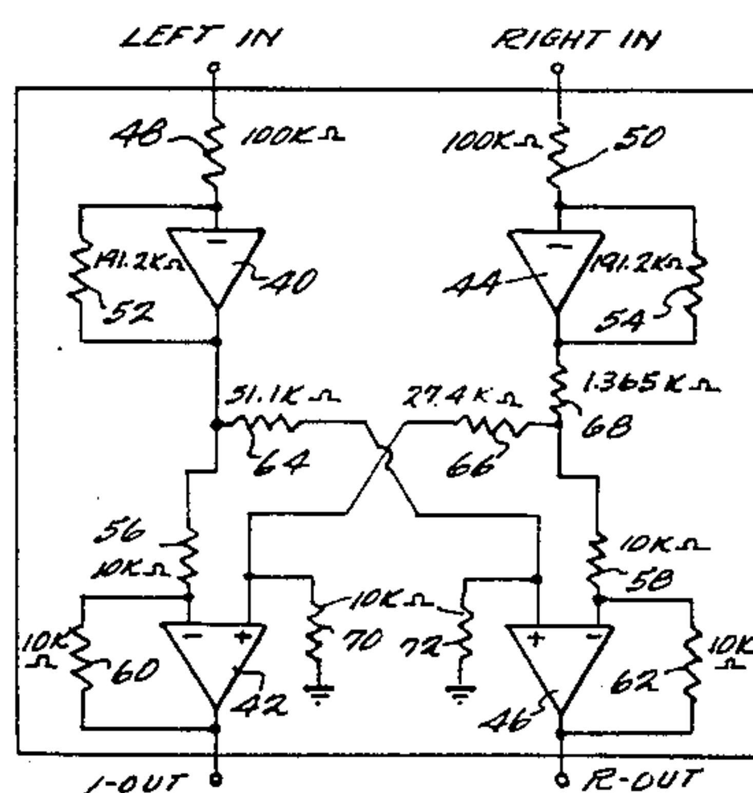
TYPICAL RIGHT-HANDED ASYMMETRIC CROSS-FEED CIRCUIT
