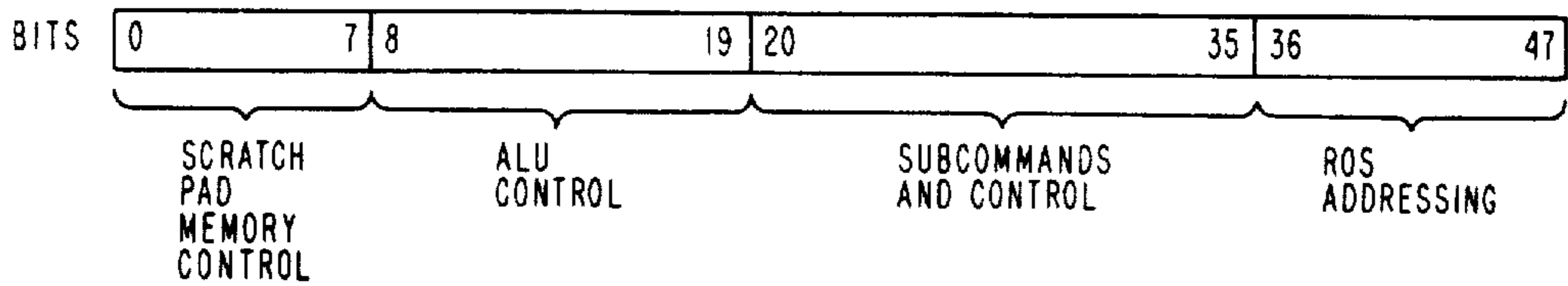
CPU FIRMWARE MICROINSTRUCTION WORD
