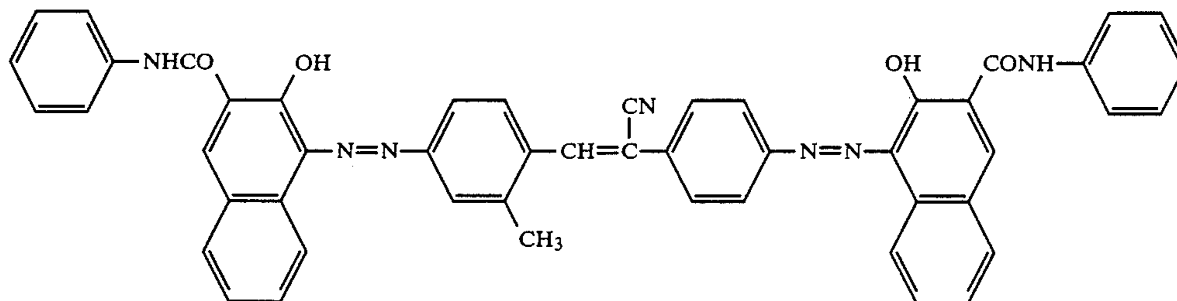
Illustrative bisazo compounds
