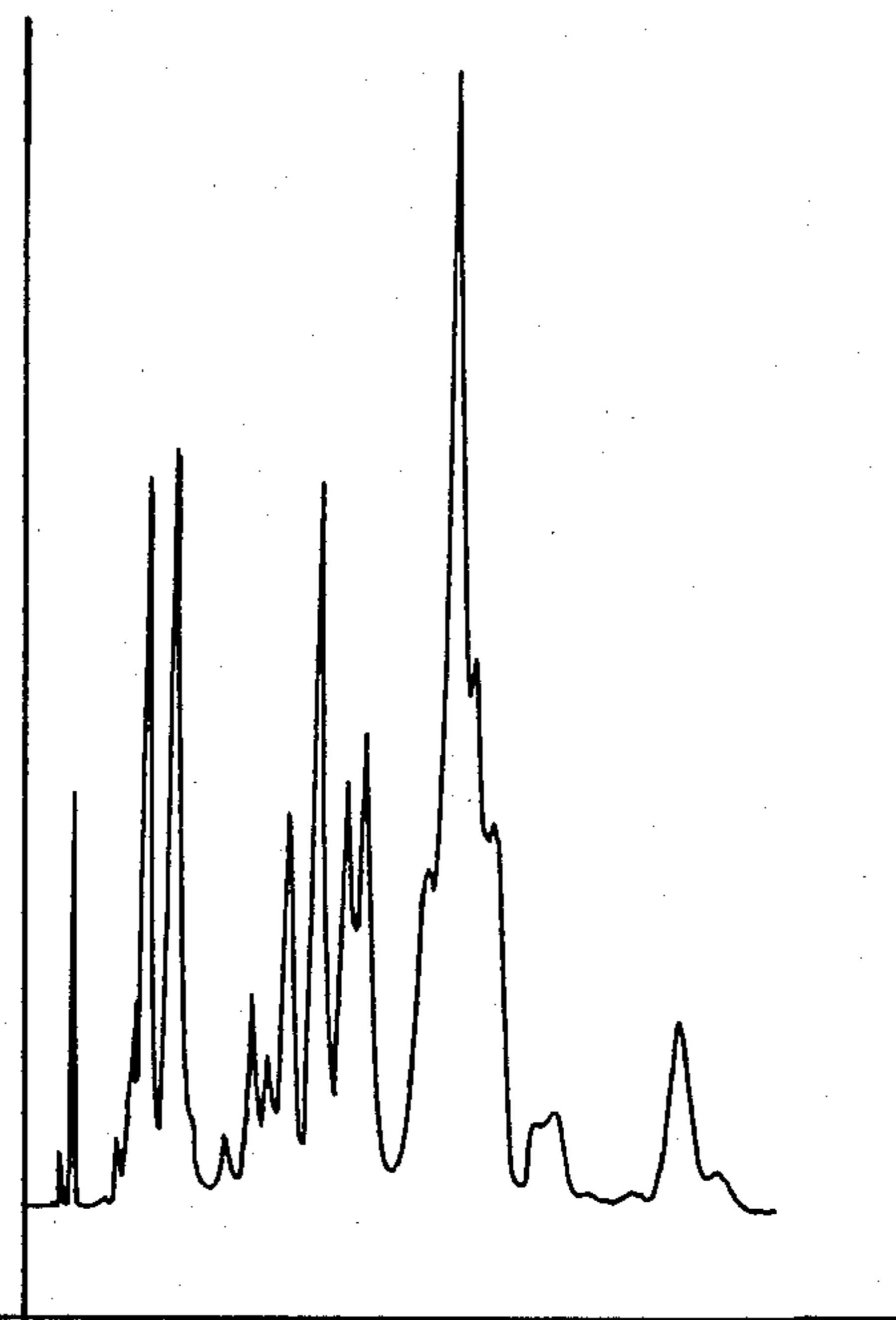
GLC PROFILE FOR EXAMPLE III.
