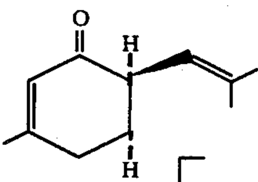
FIG. 13 is the infra-red spectrum for Peak 4A of the foregoing GLC profile having the structure:
