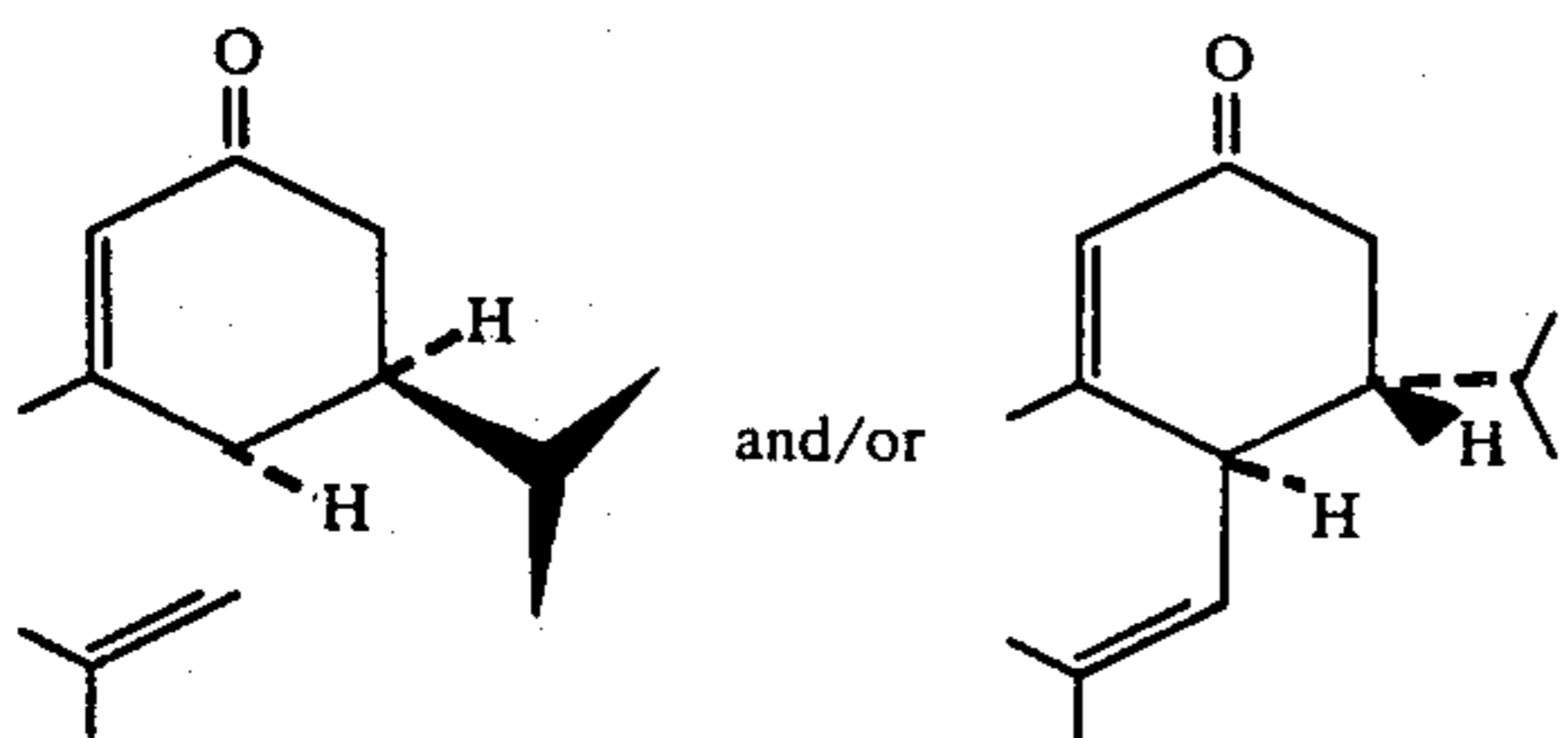
FIG. 14 is the NMR spectrum for Peak 4B of the foregoing GLC profile having the structure:
