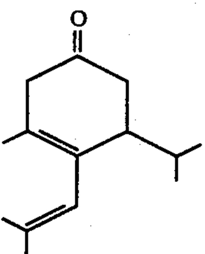
FIG. 11 is the infra-red spectrum for Peak 3 of the foregoing GLC profile having the structure:
