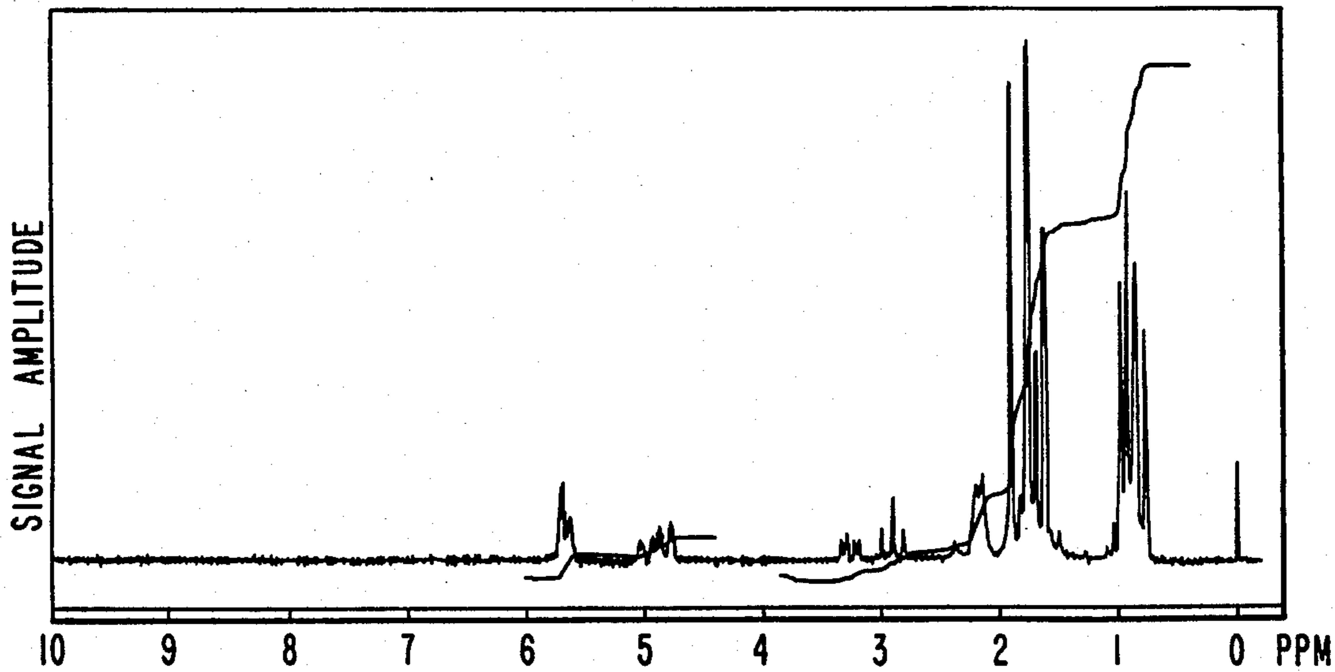
NMR SPECTRUM FOR PEAK 4A OF EXAMPLE I.
