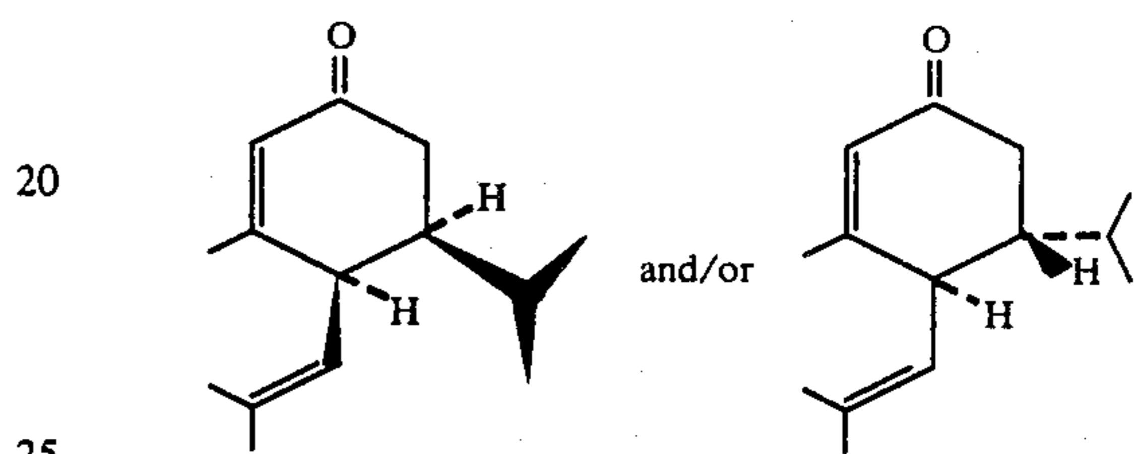
FIG. 17 is the infra-red spectrum for Peak 5 of the foregoing GLC profile having the structure:
