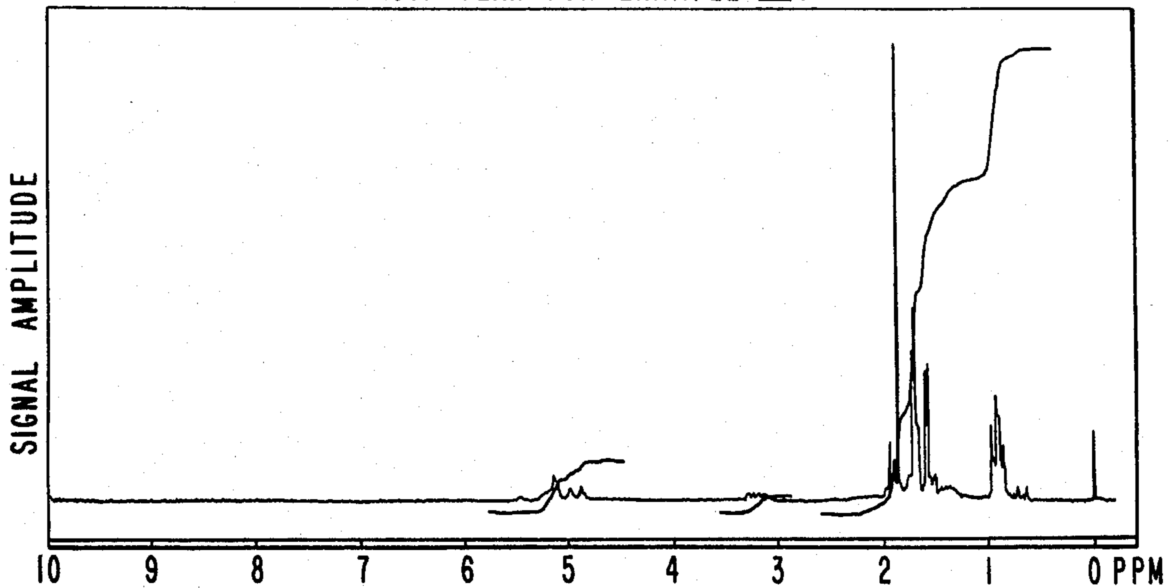
NMR SPECTRUM FOR MAJOR PEAK FOR EXAMPLE IV.
