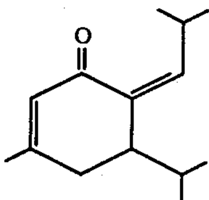
FIG. 10 is the NMR spectrum for Peak 3 of the foregoing GLC profile having the structure:
