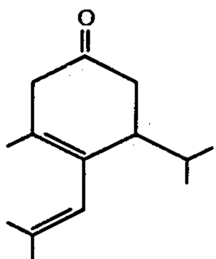
FIG. 12 is the NMR spectrum for Peak 4A of the GLC profile of FIG. 4 which signifies the compound having the structure:
