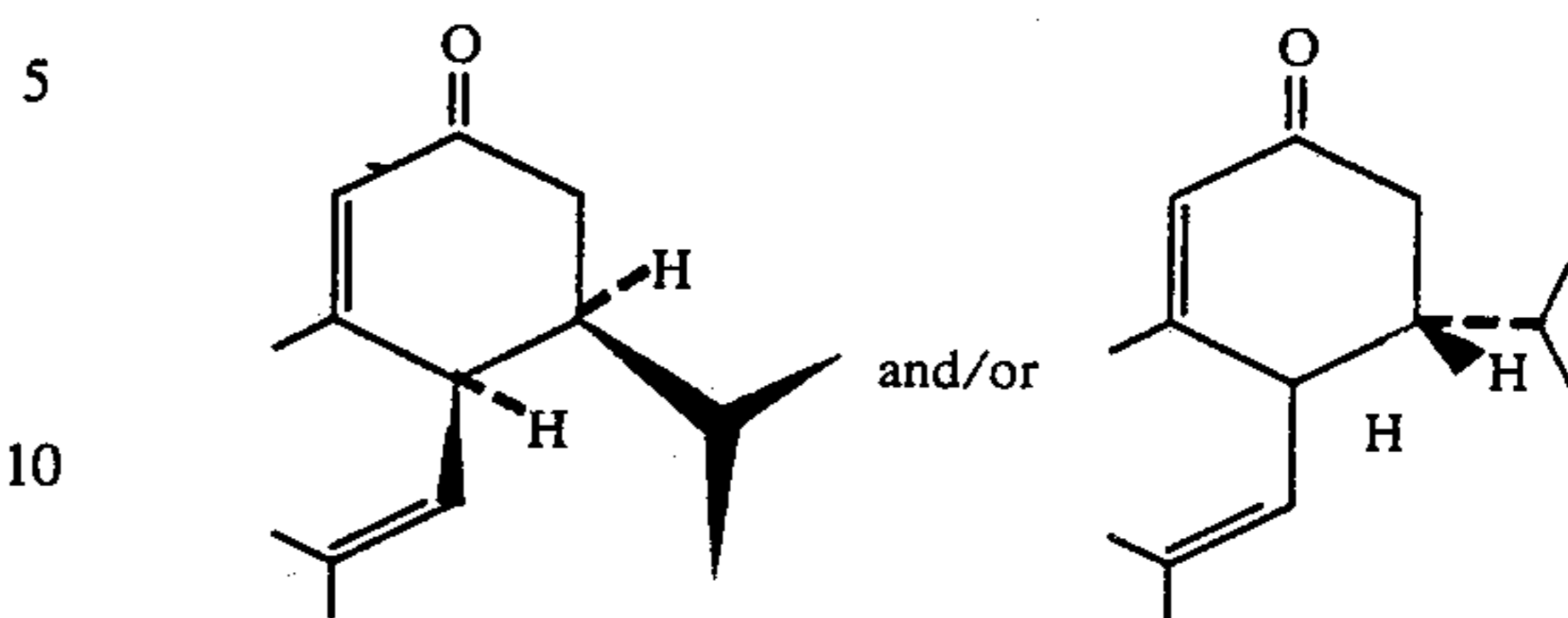
FIG. 16 is the NMR spectrum for Peak 5 of the foregoing GLC profile having the structure:
