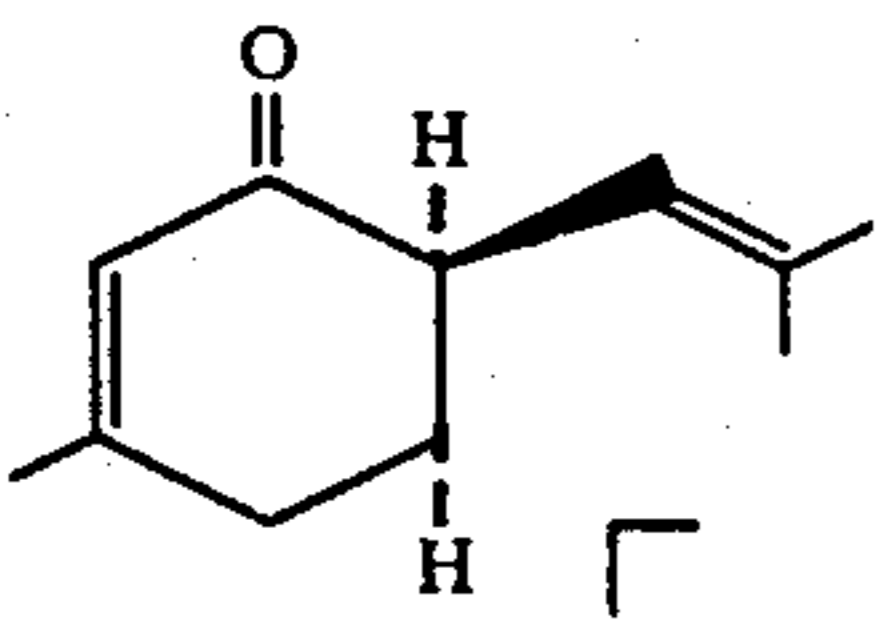
FIG. 14 is the NMR spectrum for Peak 4B of the foregoing GLC profile having the structure:
