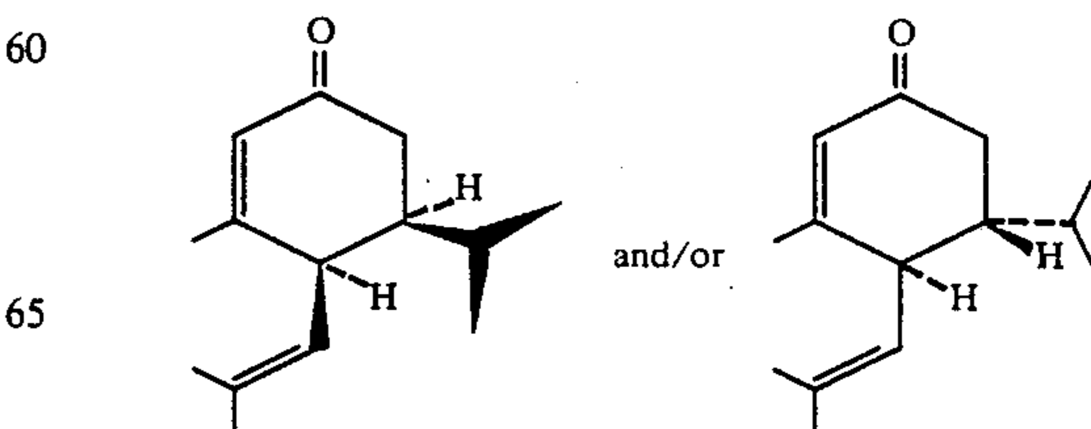
FIG. 14 is the NMR spectrum for Peak 4B of the GLC profile of FIG. 4 signifying the compound having the structure:
