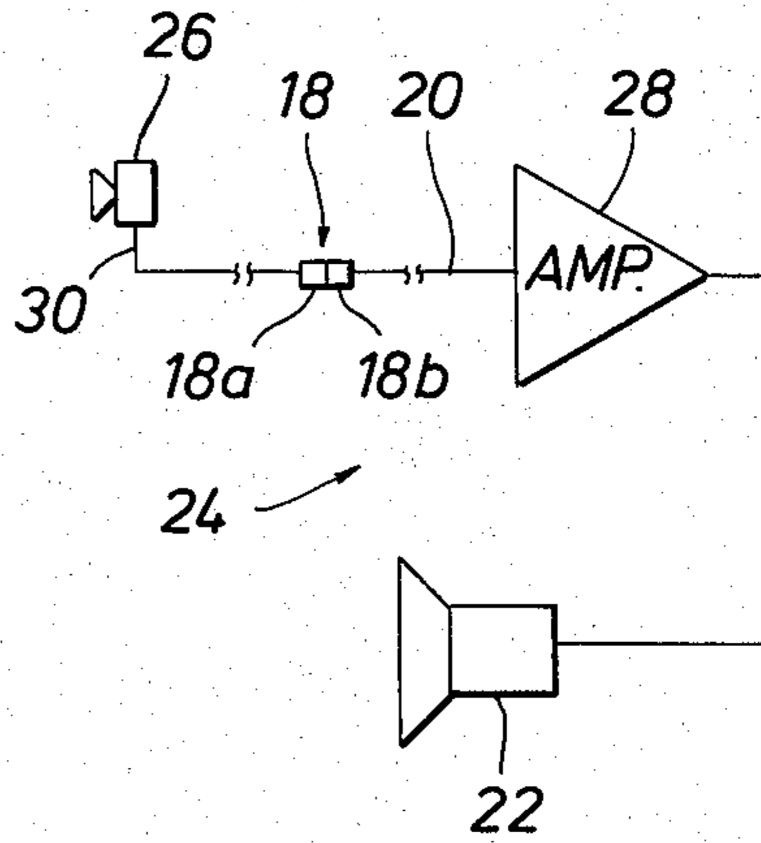
FIG. 2 (PRIOR ART)
