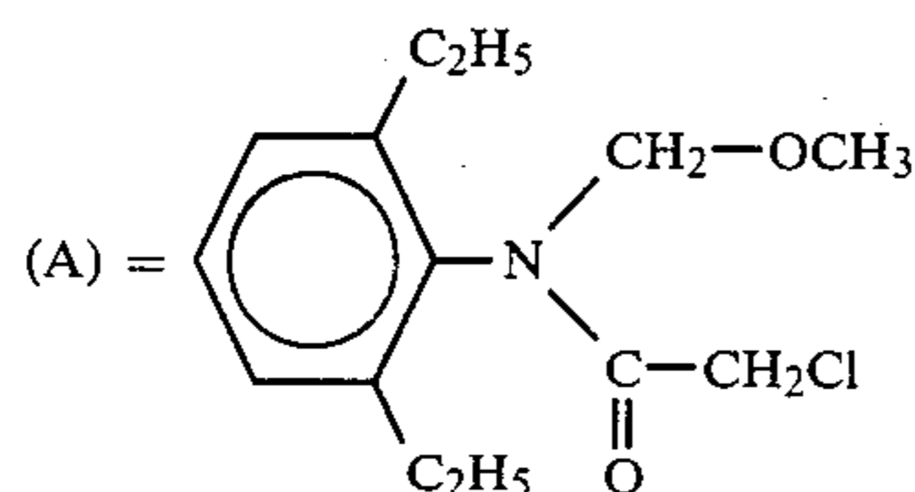
(2,6-diethyl)-N-methoxymethyl-chloroacetanilide.
